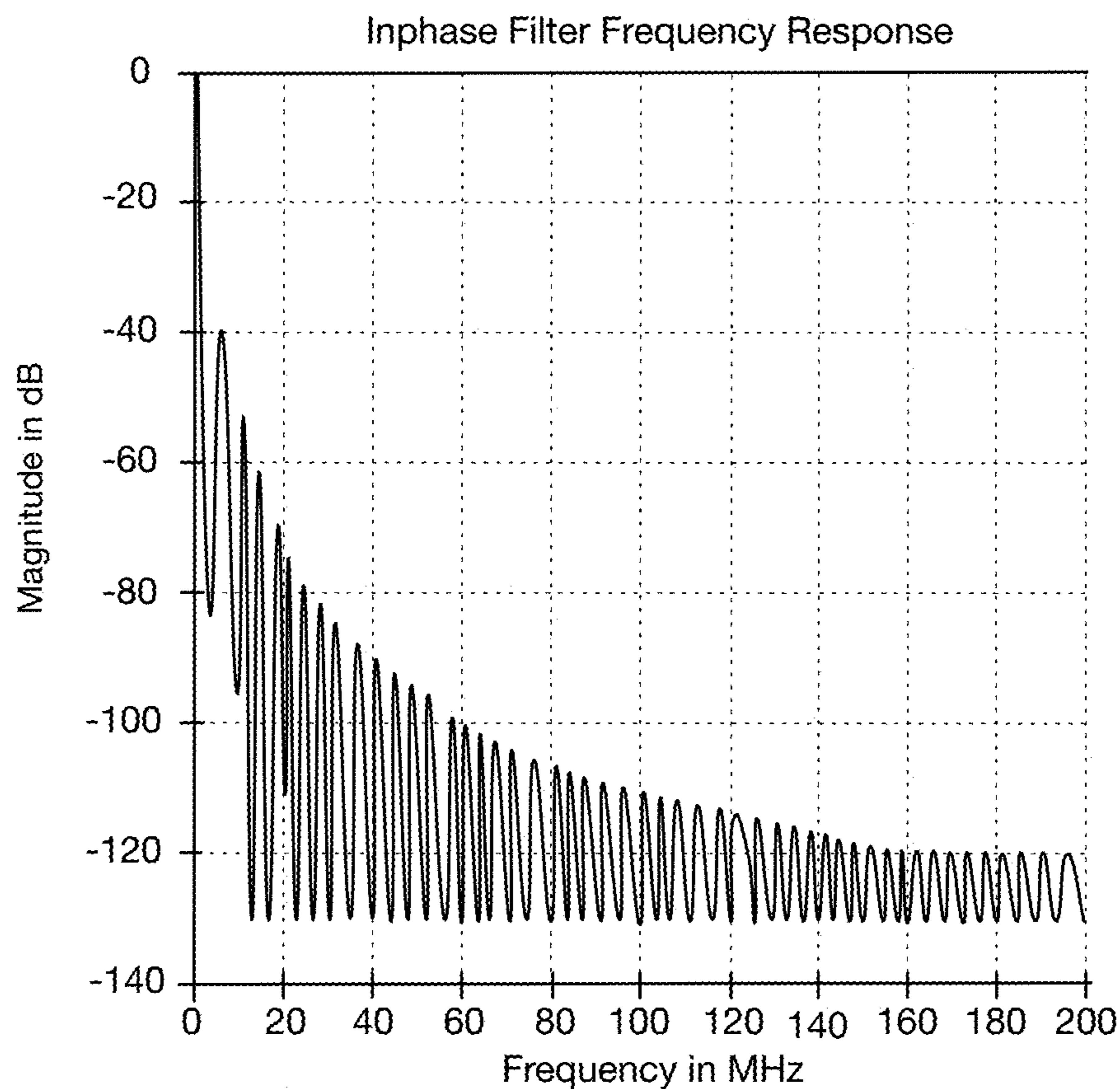
Inphase Filter Frequency Response
