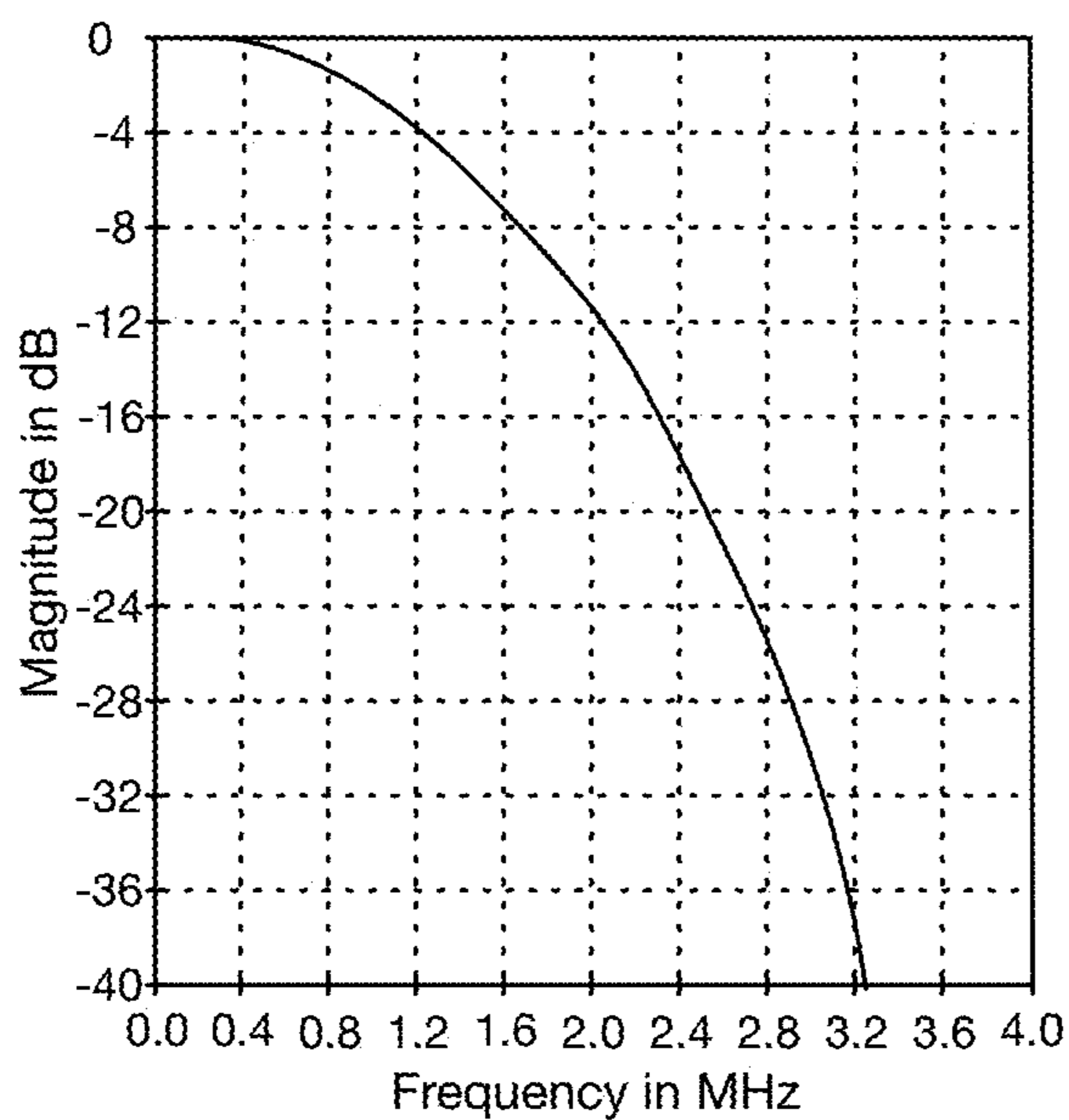
Inphase Filter Frequency Response
