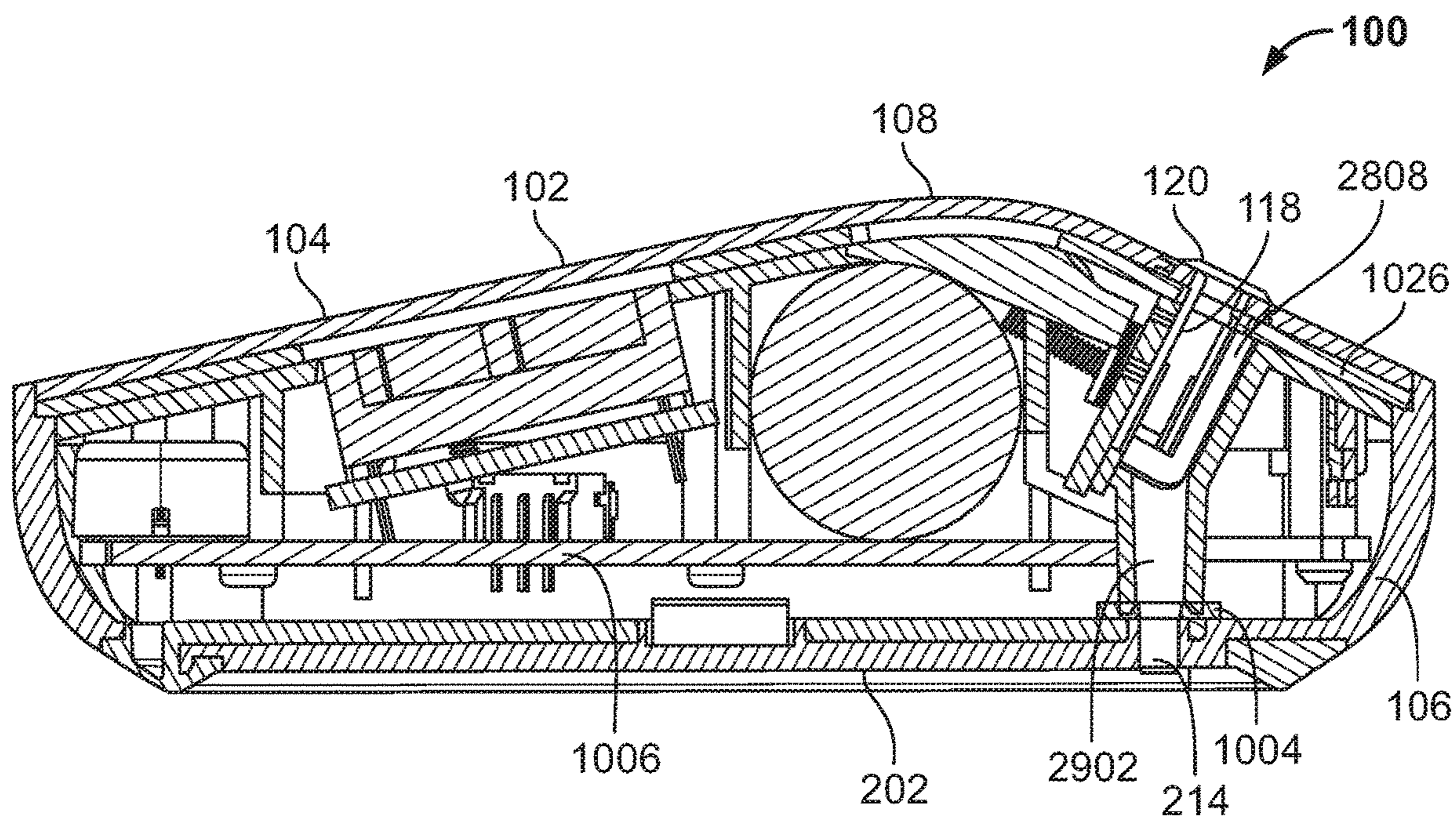
SECTION G-G
