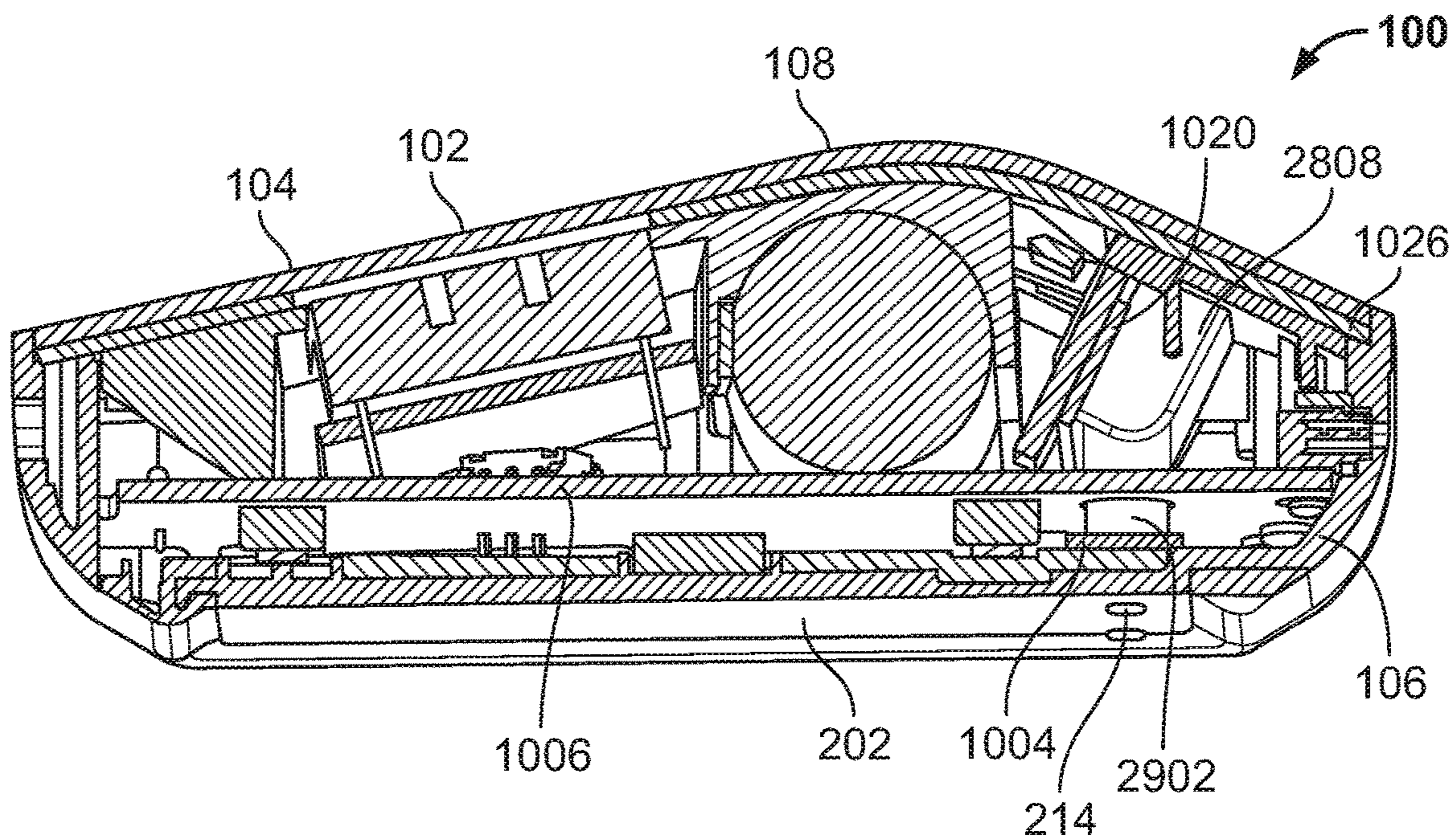
SECTION E-E
