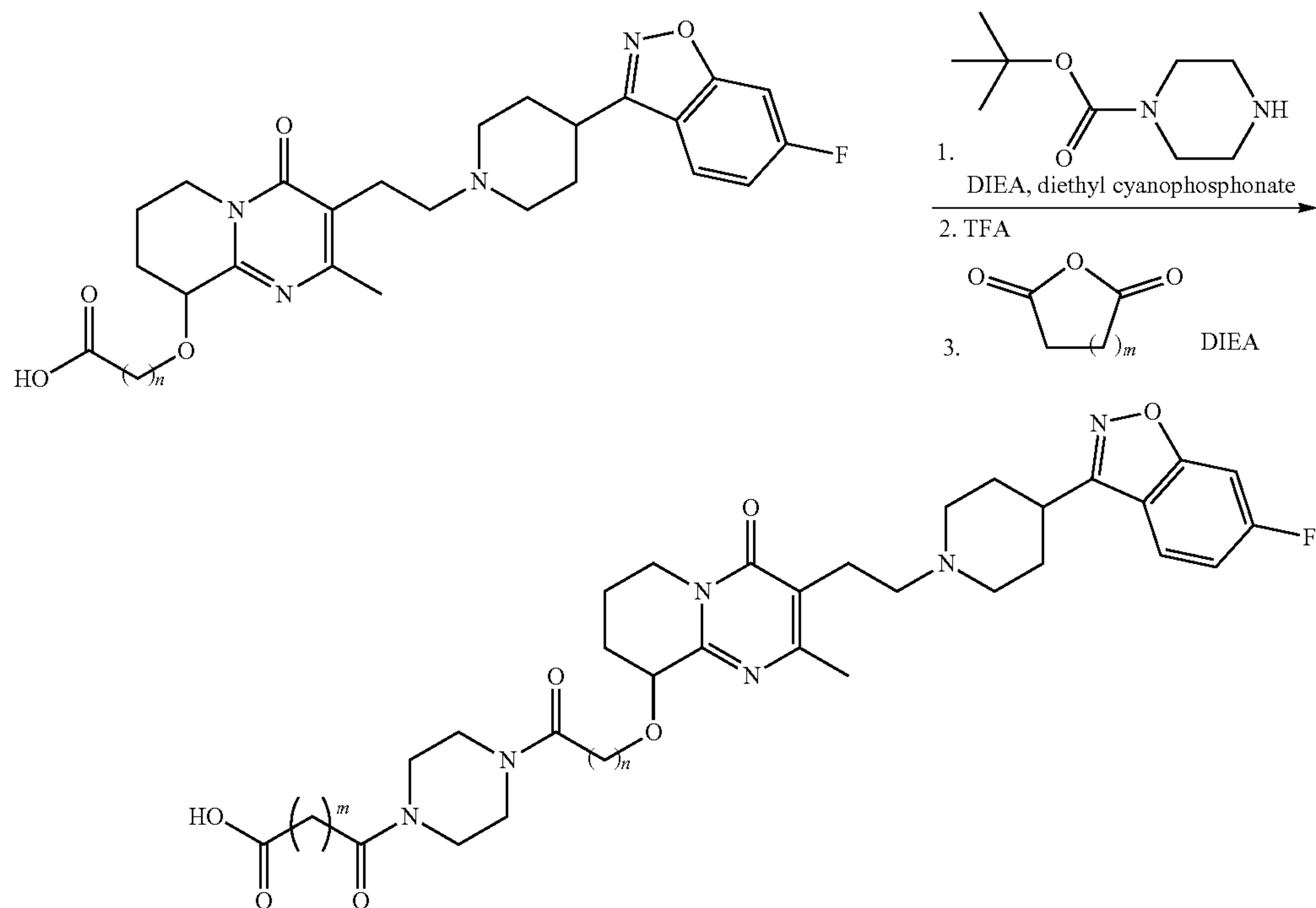
Scheme 4
