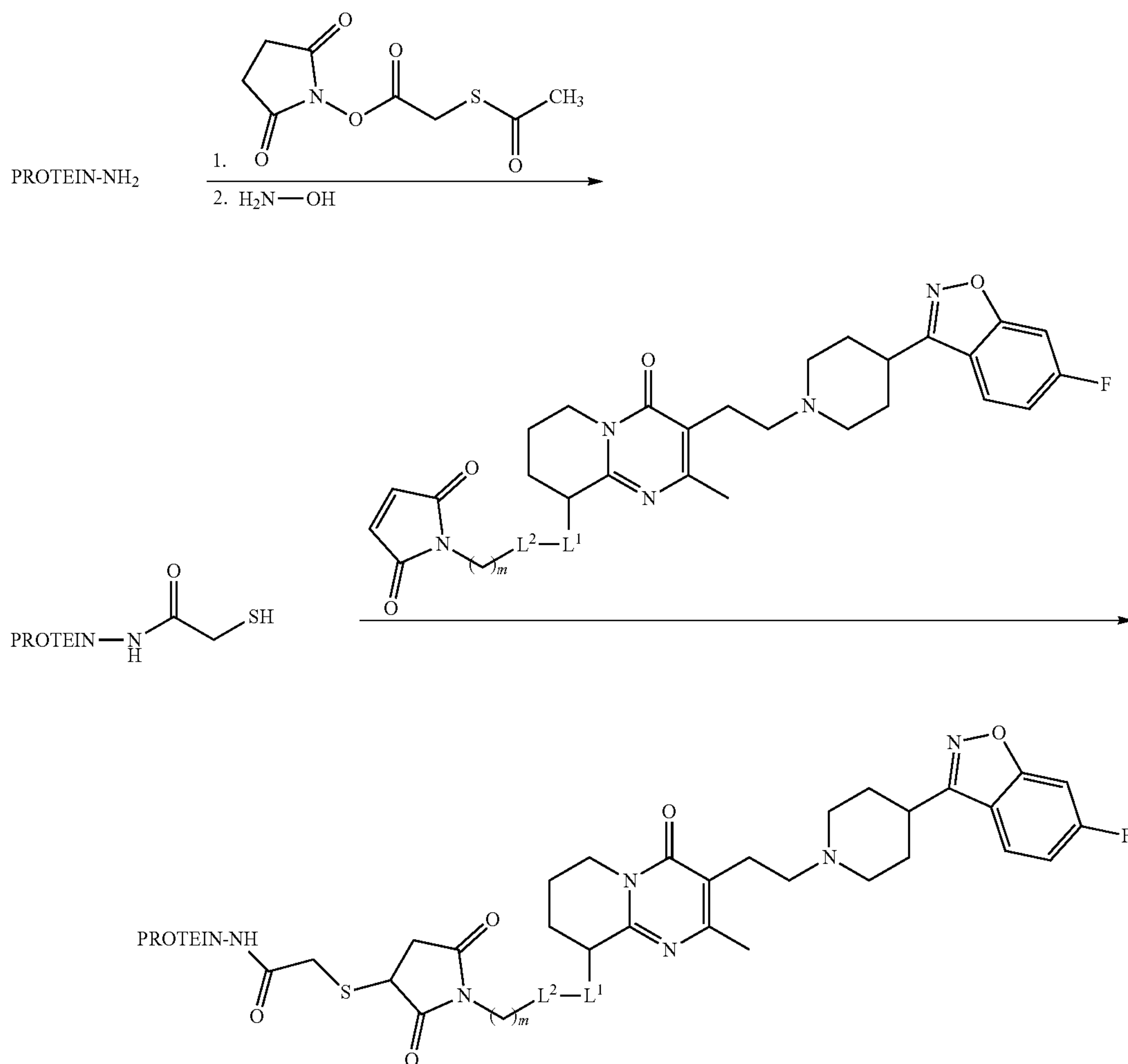
Scheme 5
