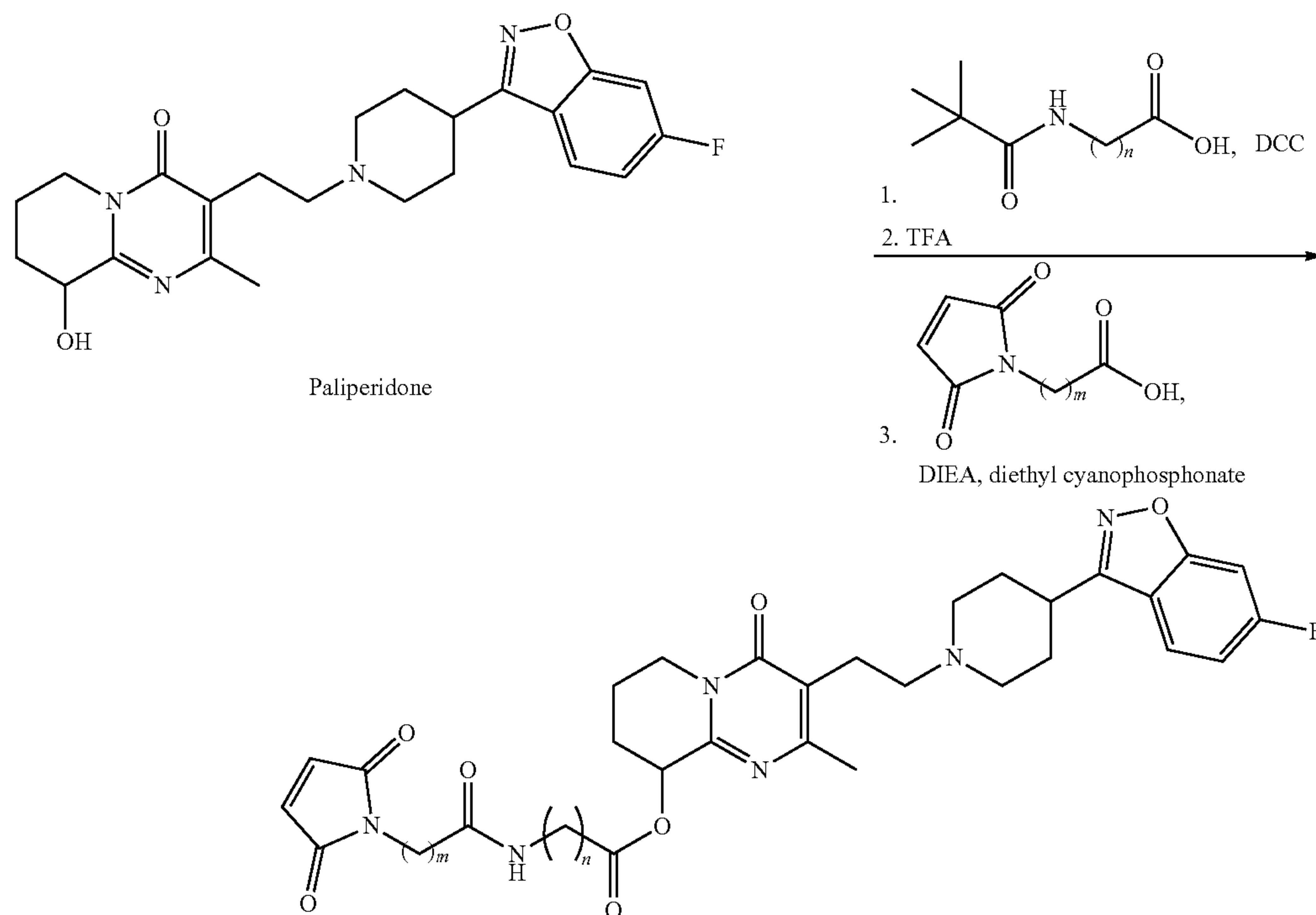
Scheme 2
