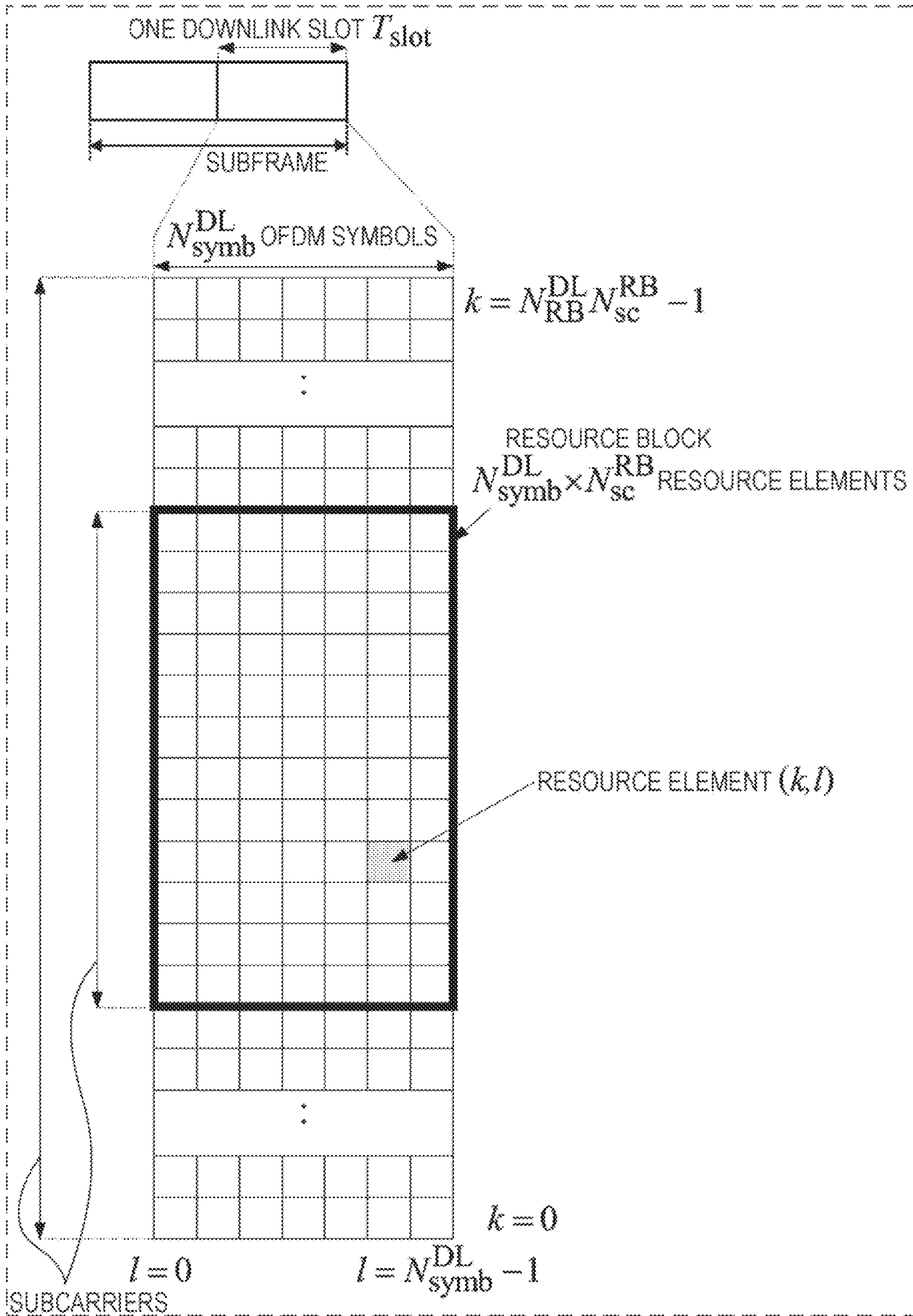
FIG. 2 (PRIOR ART)
