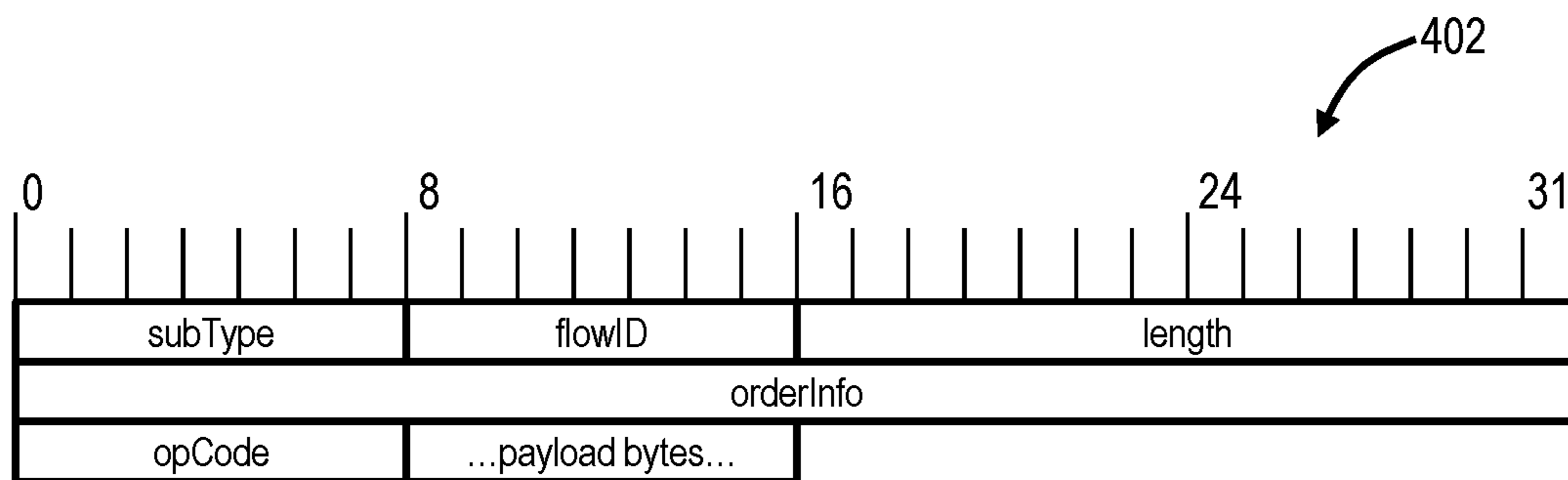
RoE control packet common frame format
