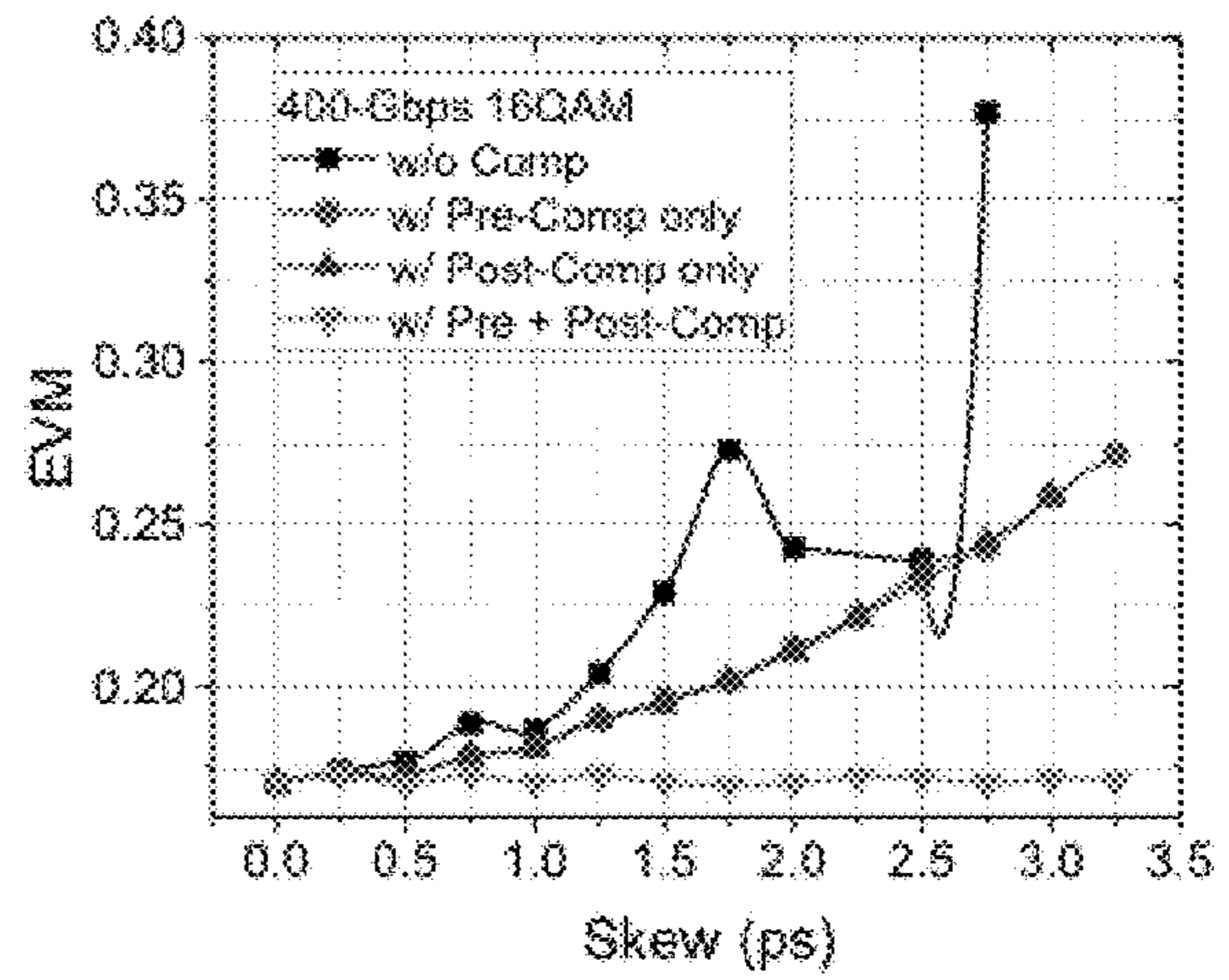
64GBd 400Gb/s 16QAM
