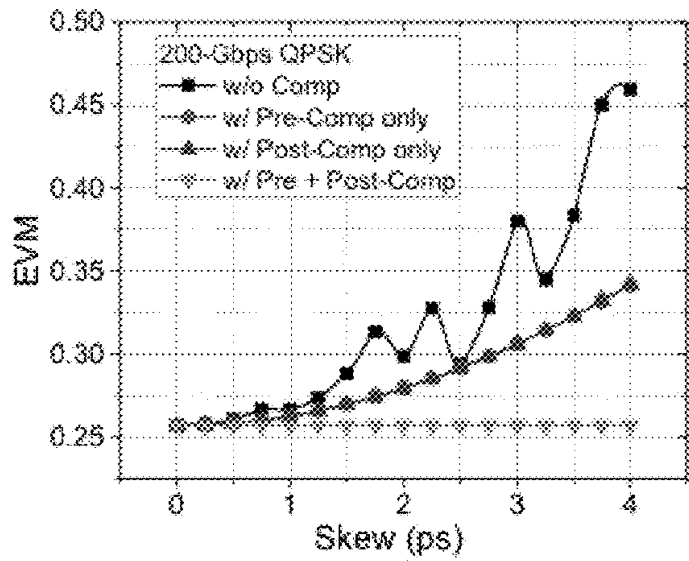
62GBd 200Gb/s QPSK
