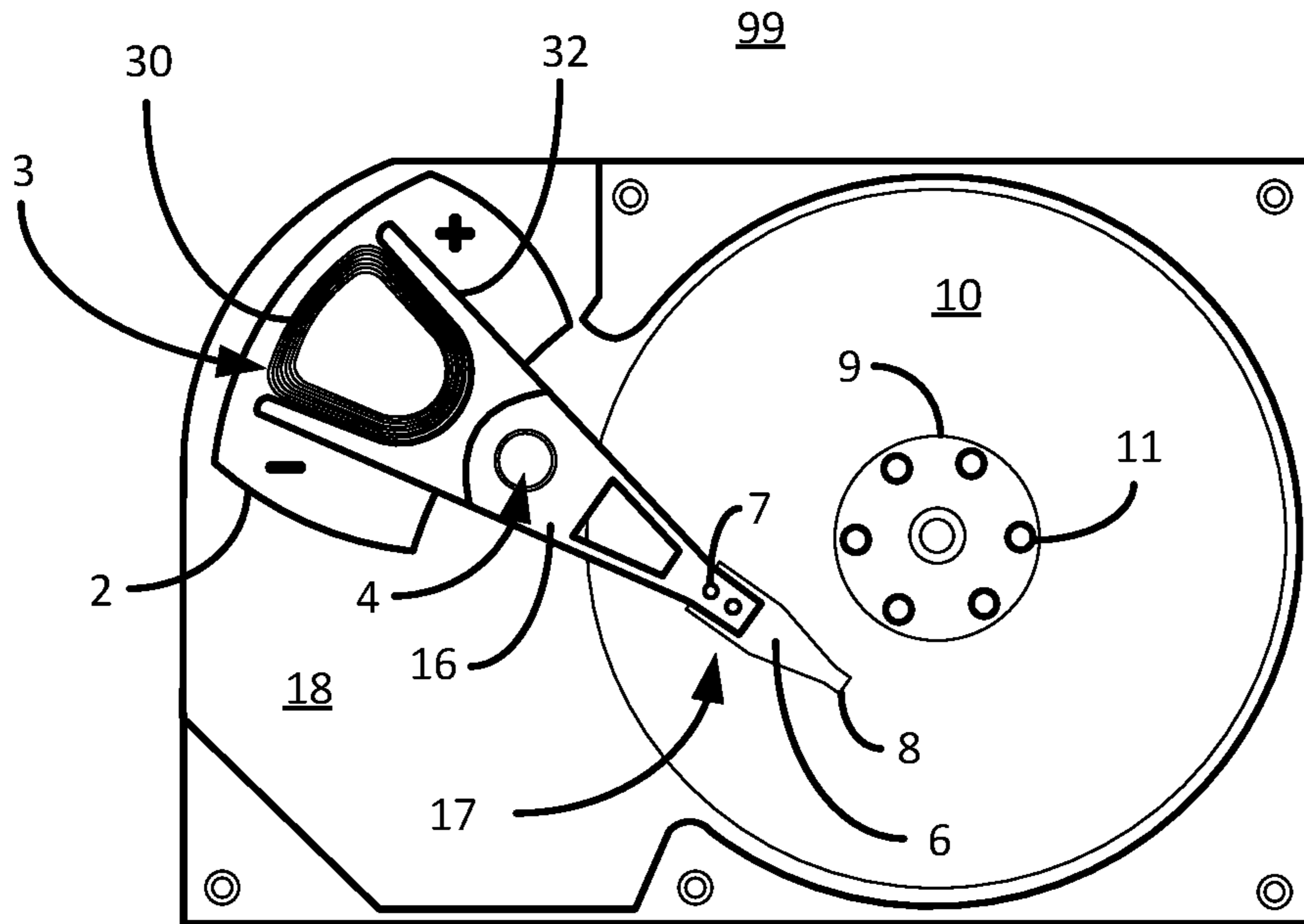
PRIOR ART FIG. 1B
