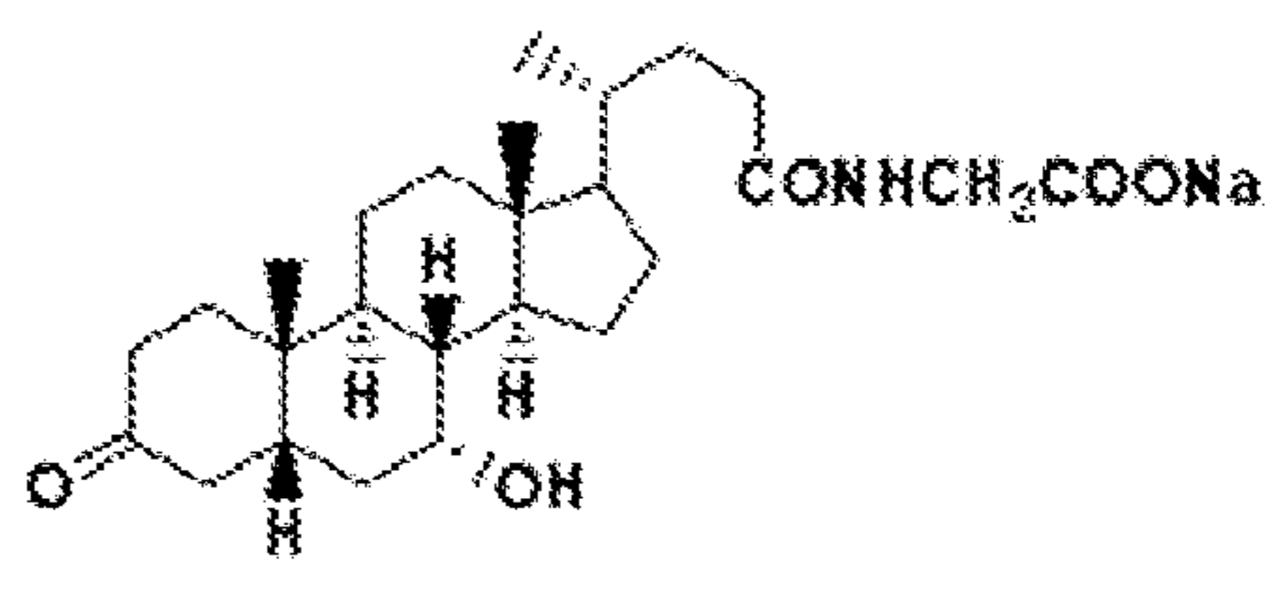
Sodium glycochenodoxycholate
