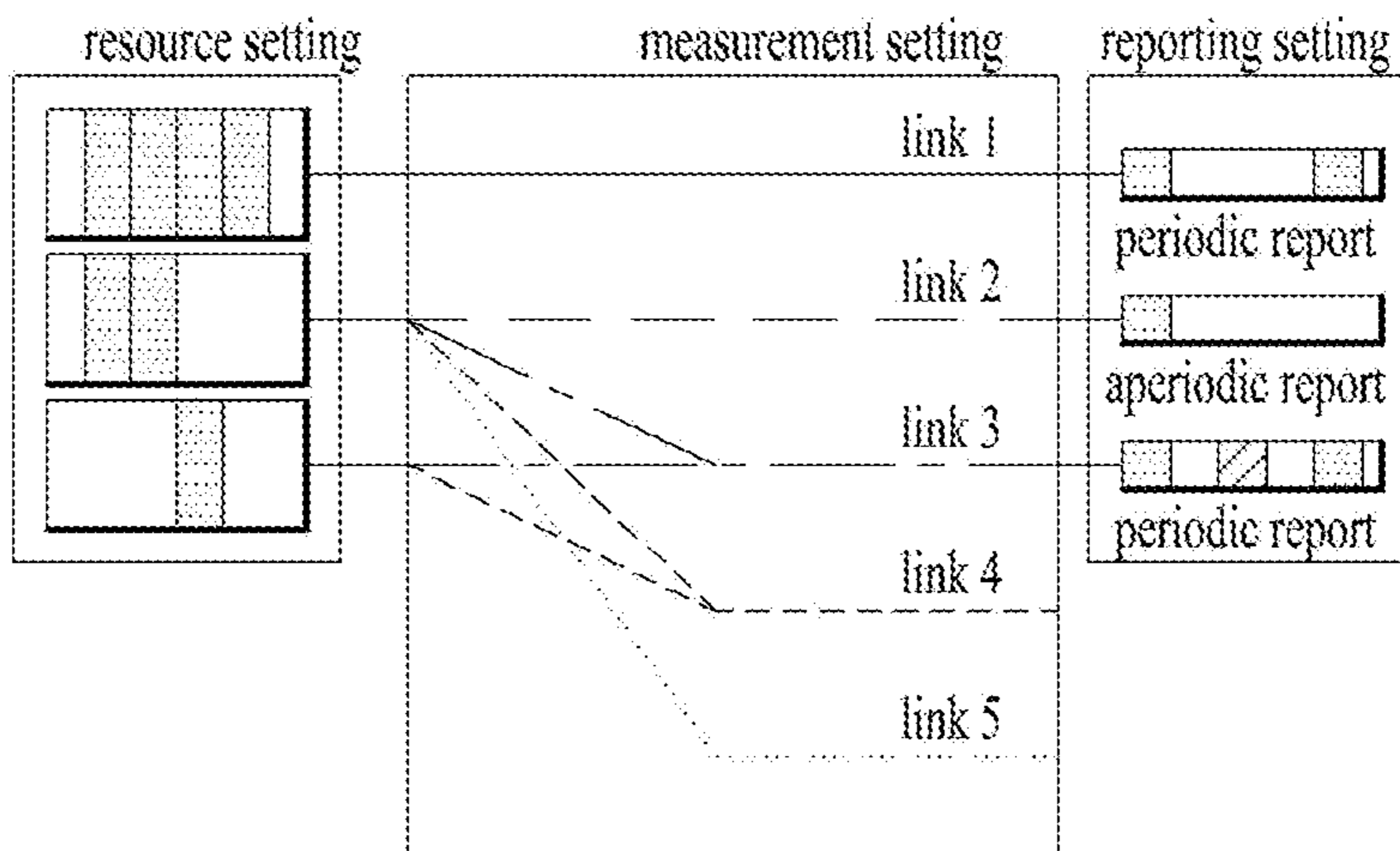
CSI acquisition/beam management framework
