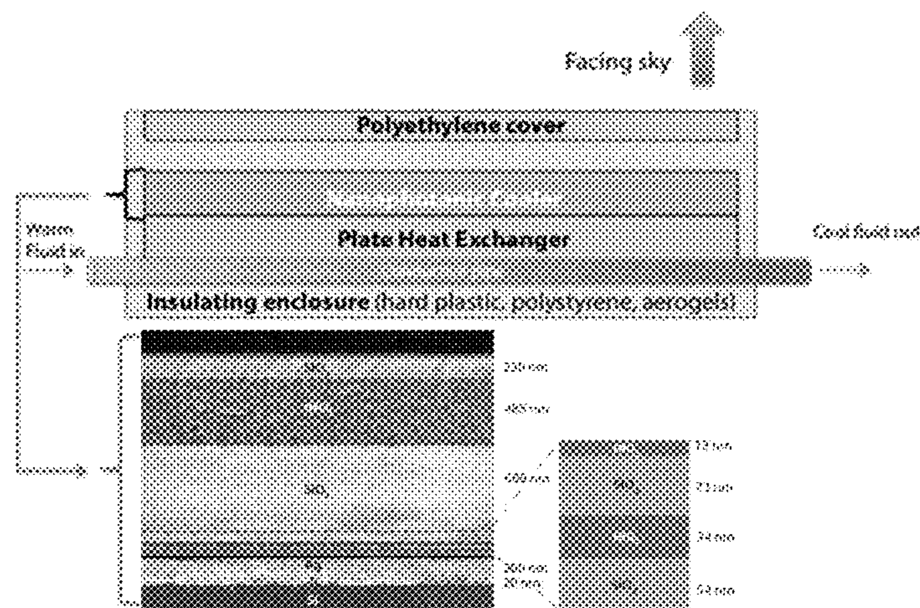
Side Profile of Radiative Cooler
