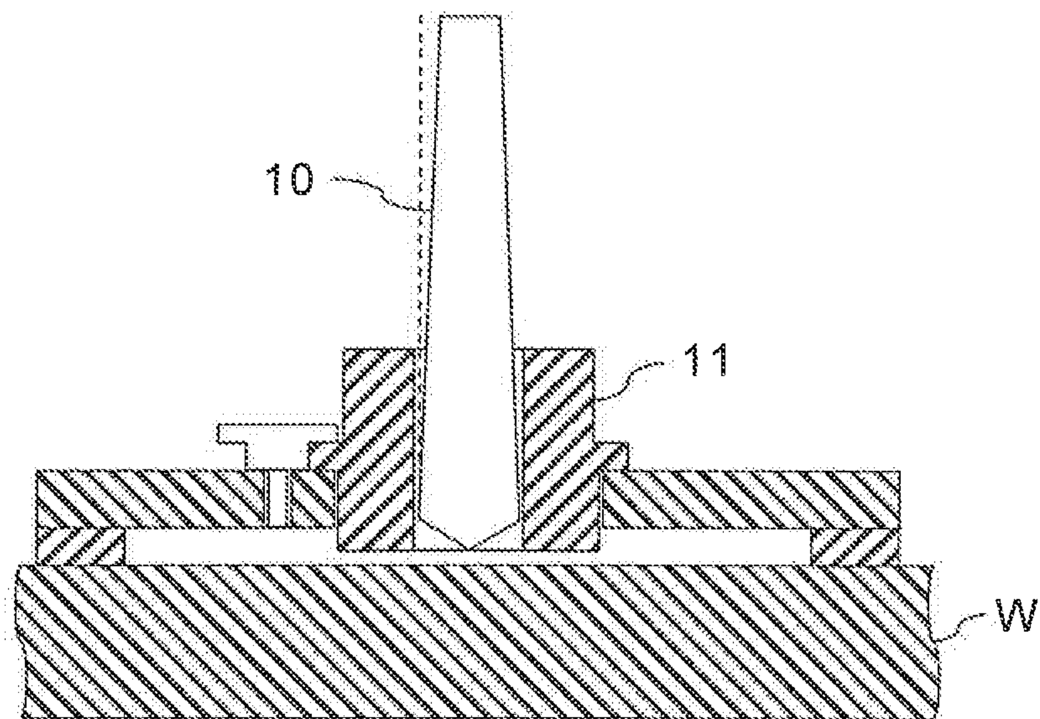
FIG. 3 PRIOR ART
