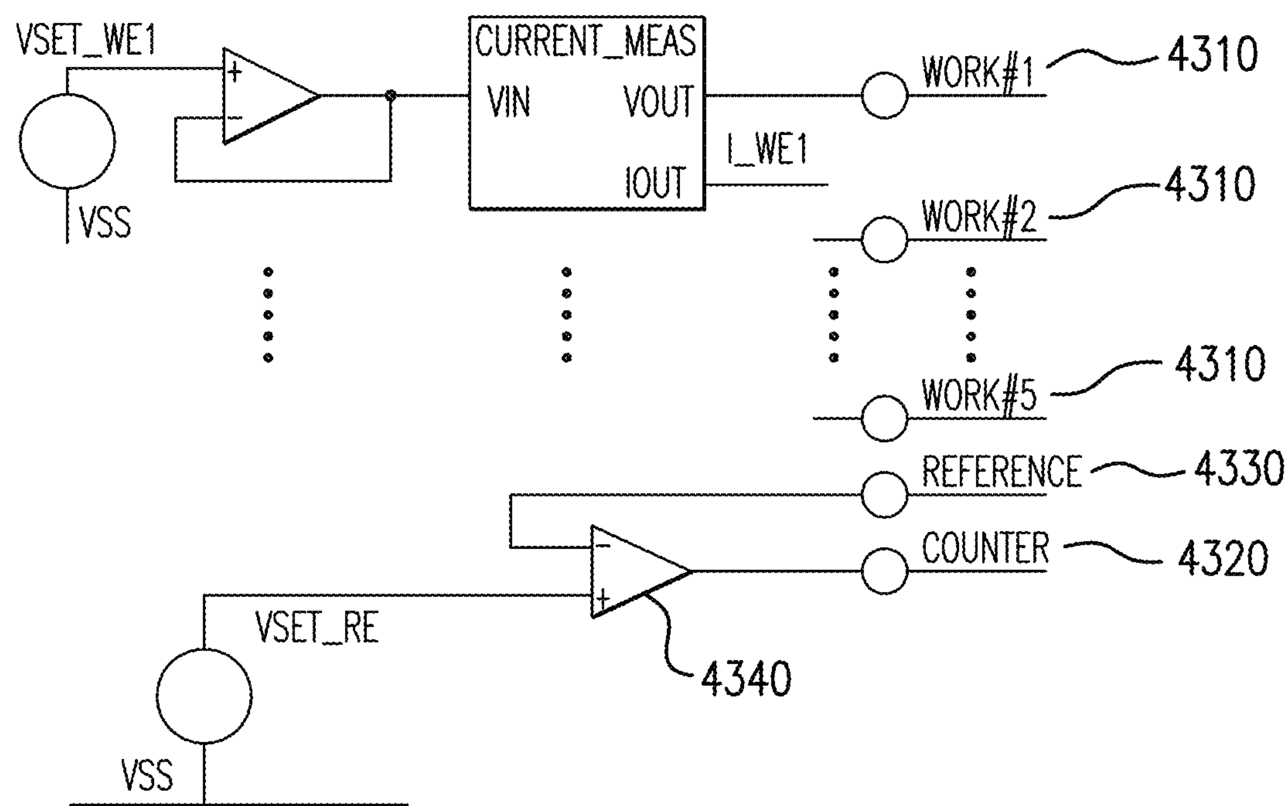
POTENTIOSTAT CONFIGURATION
