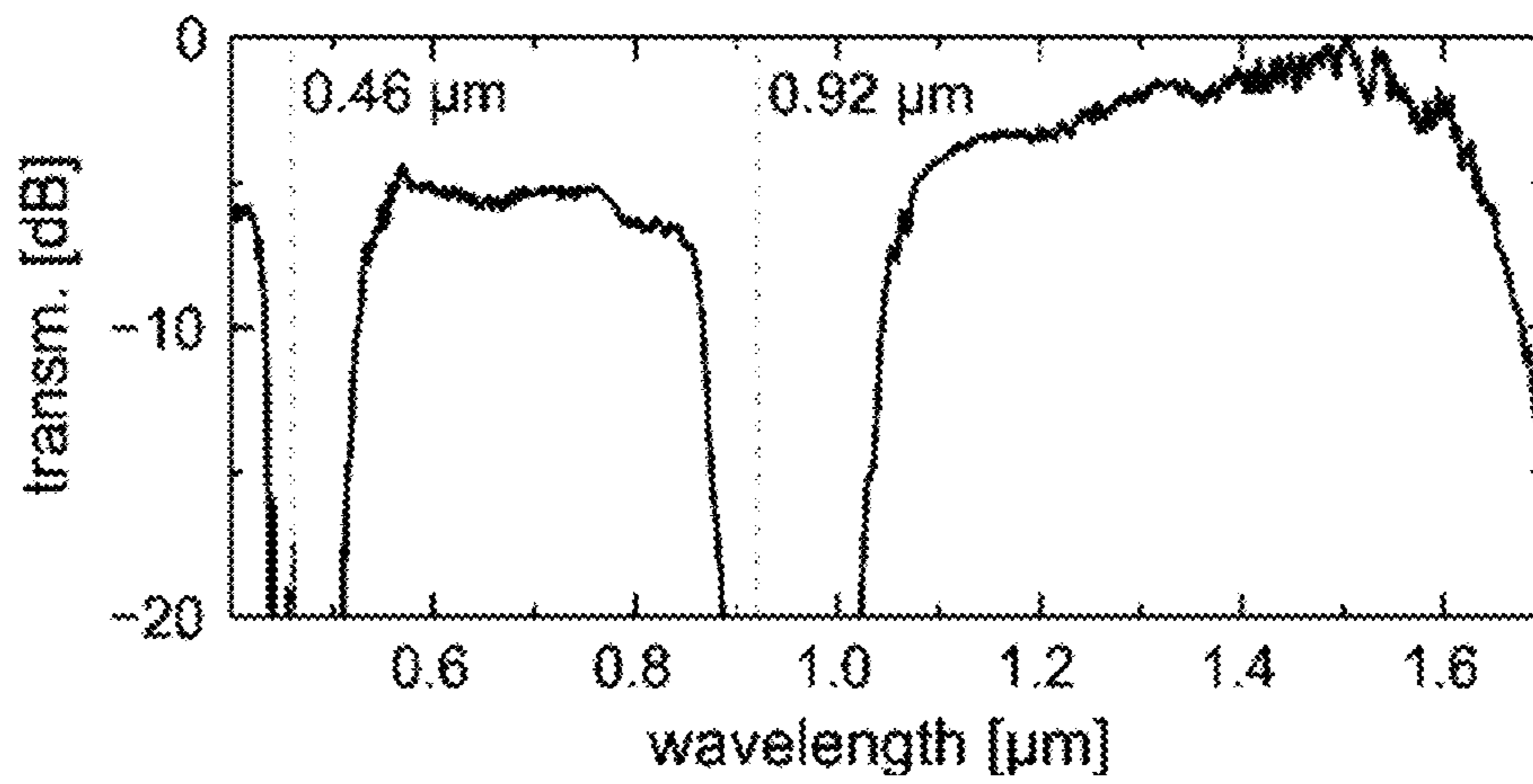
FIG. 7 (Prior art)
