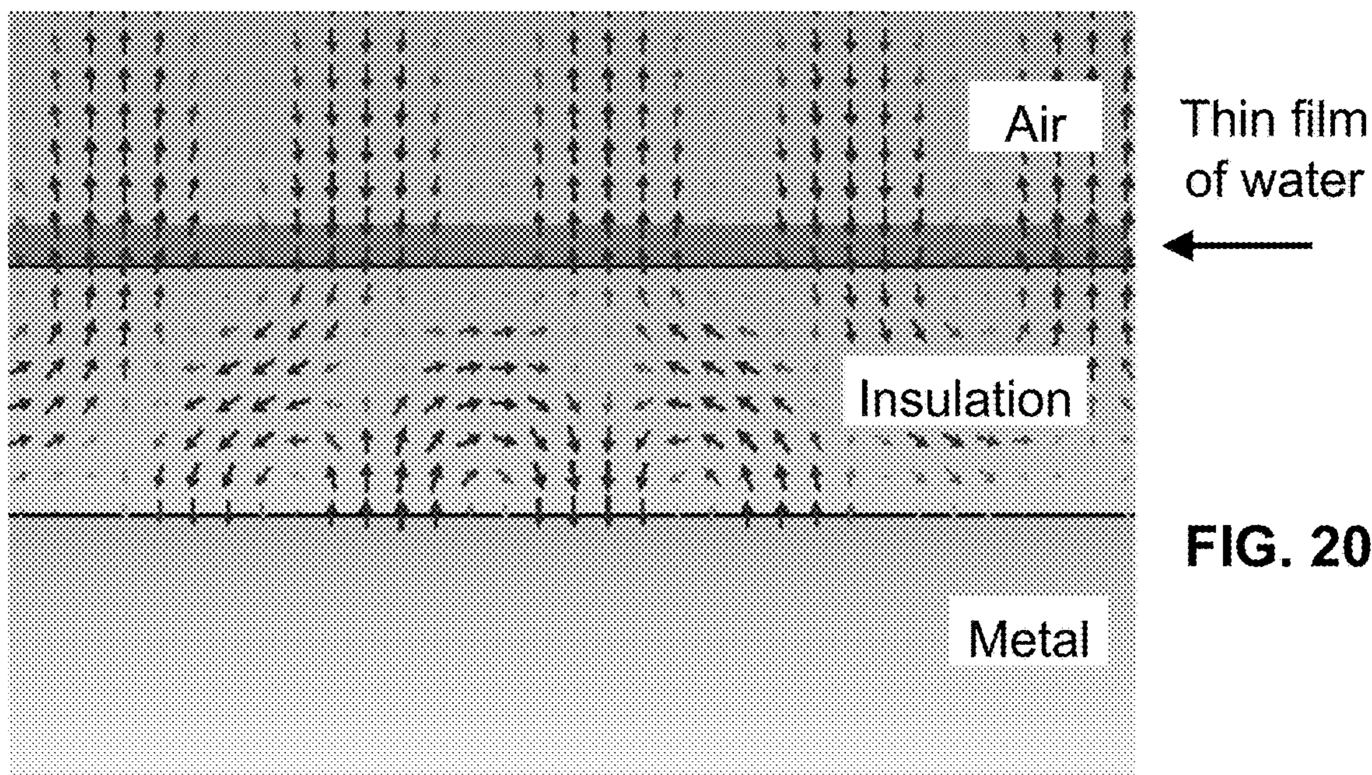
Longitudinal Section of Cable showing e-fields of waves that include a component of TM 01 waves at 40 GHz
