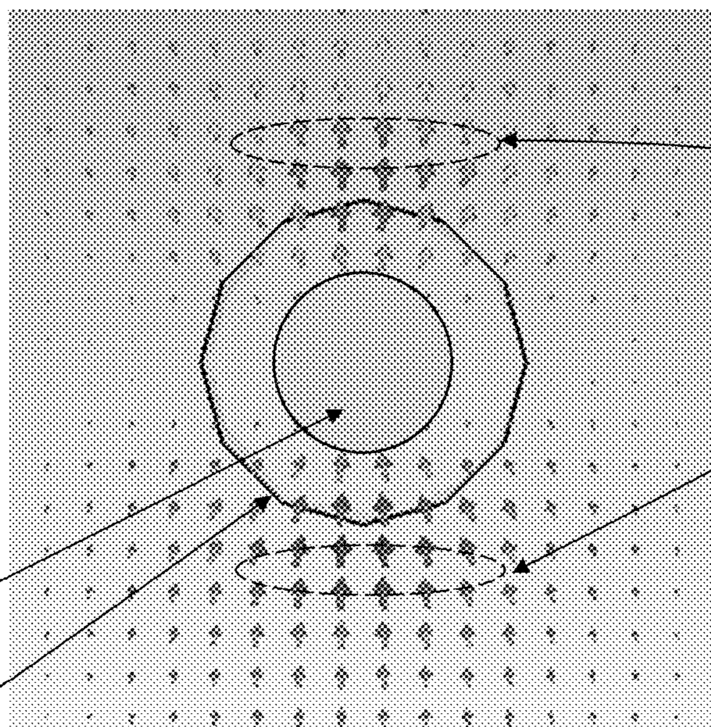
FIG. 20L HE Wave Mode (Large Mode Size)
