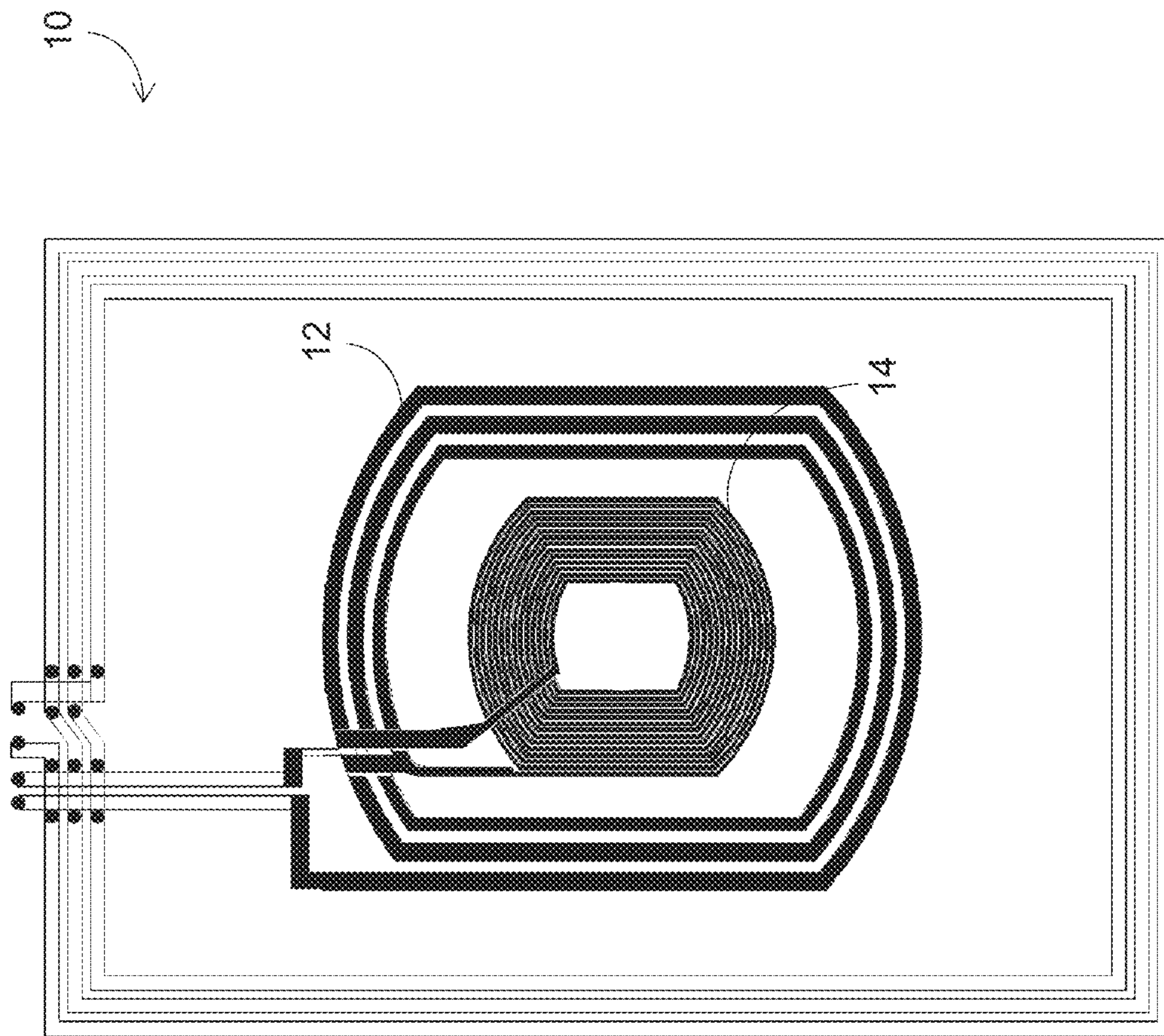
FIG. 1 PRIOR ART
