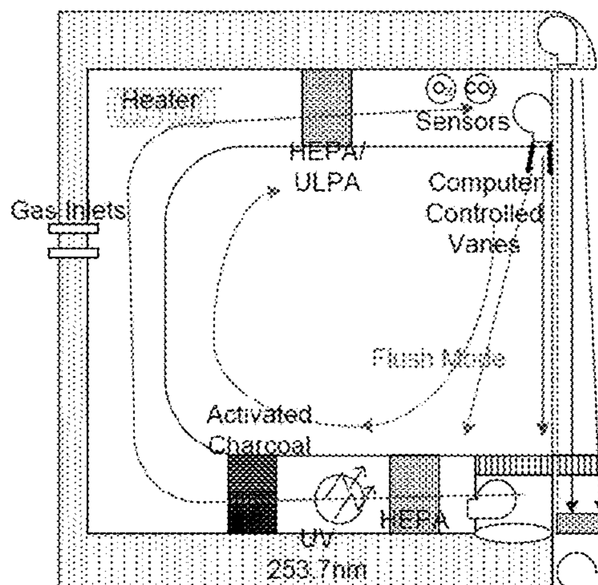
Air Interchange (Flush) Mode
