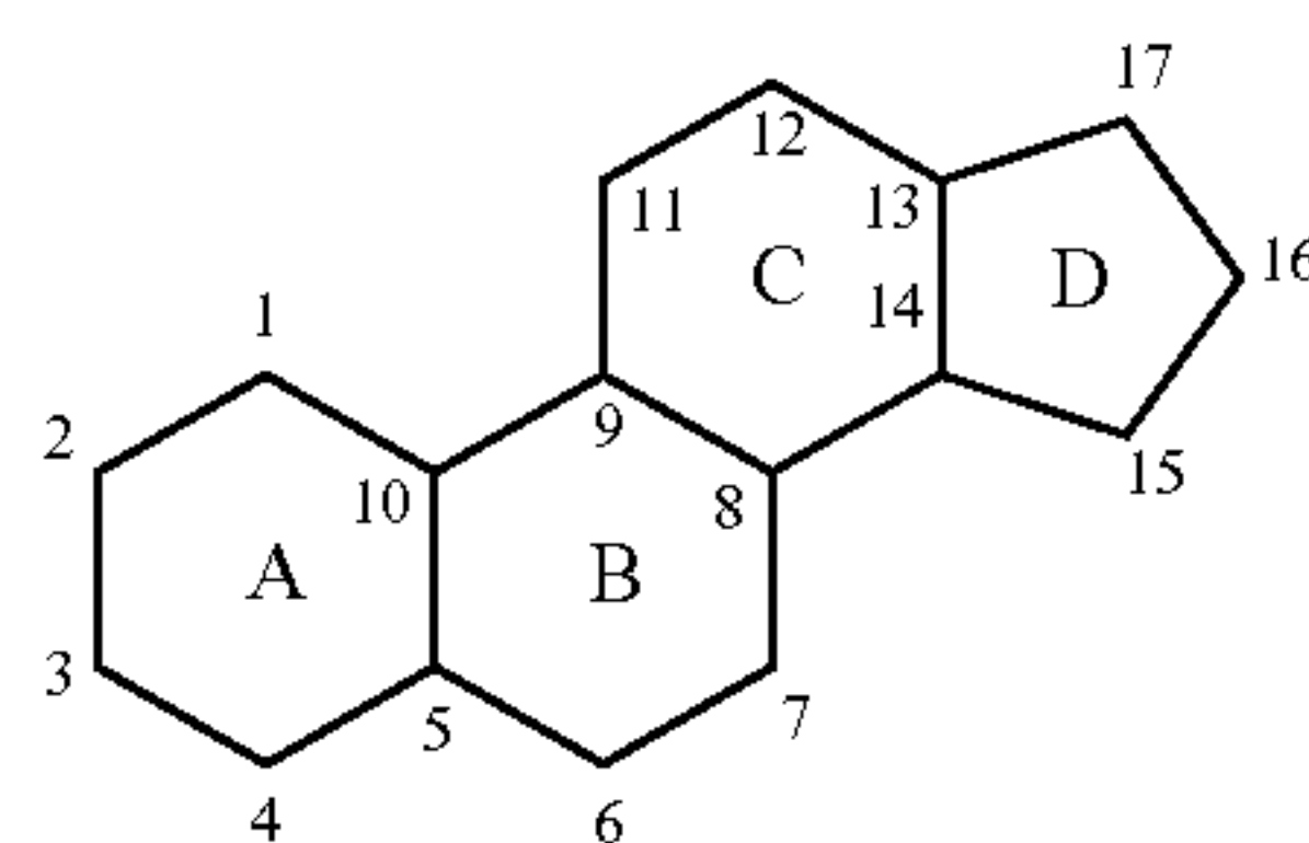
Steroidal Backbone
