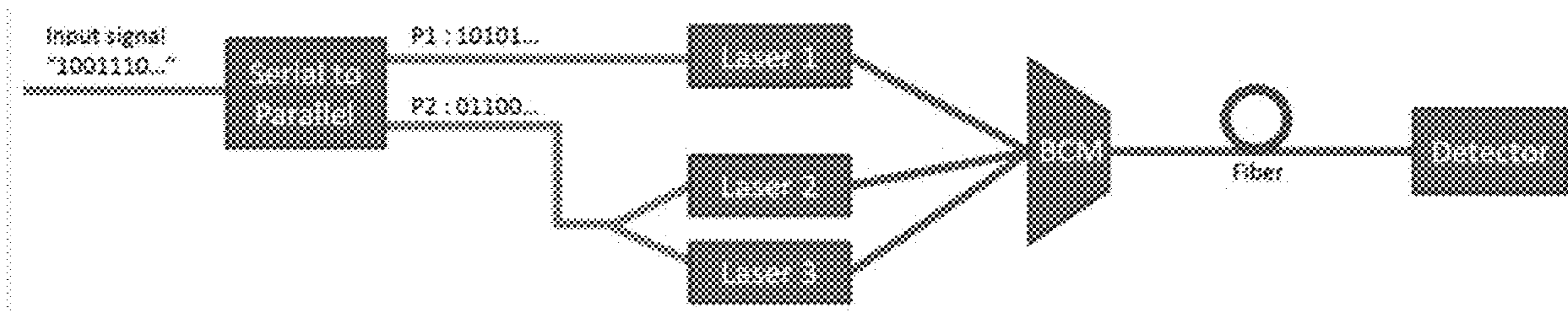
Fig. 21A PAM-4 system
