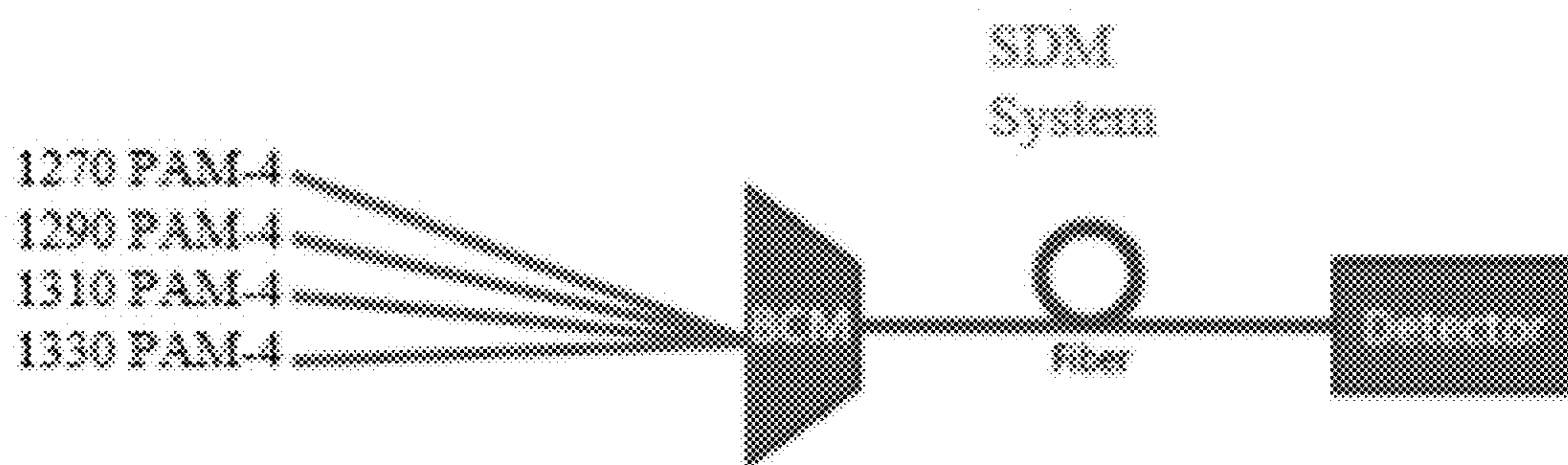
Fig. 33 Spatial domain multiplexing and PAM-4 with CWDM
