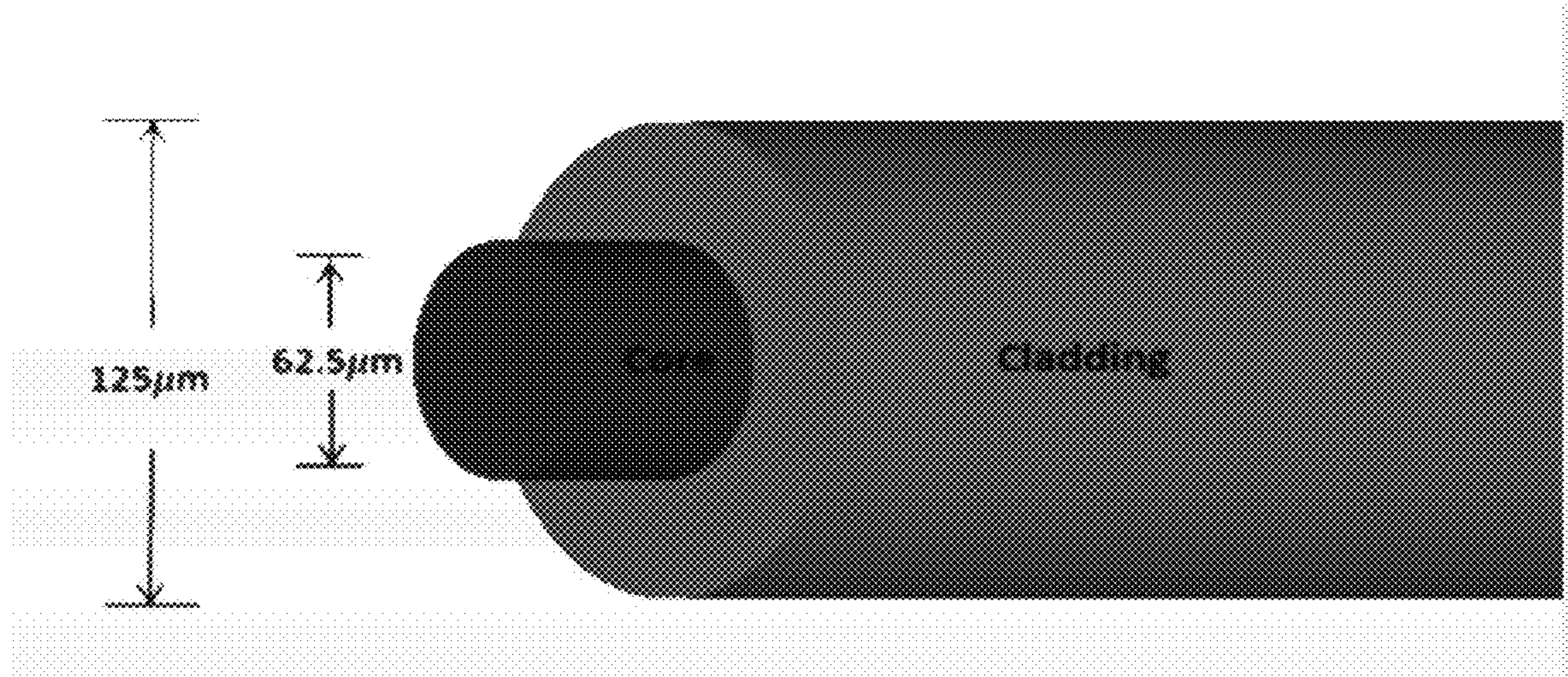
Fig. 5A Standard multi-mode fiber
