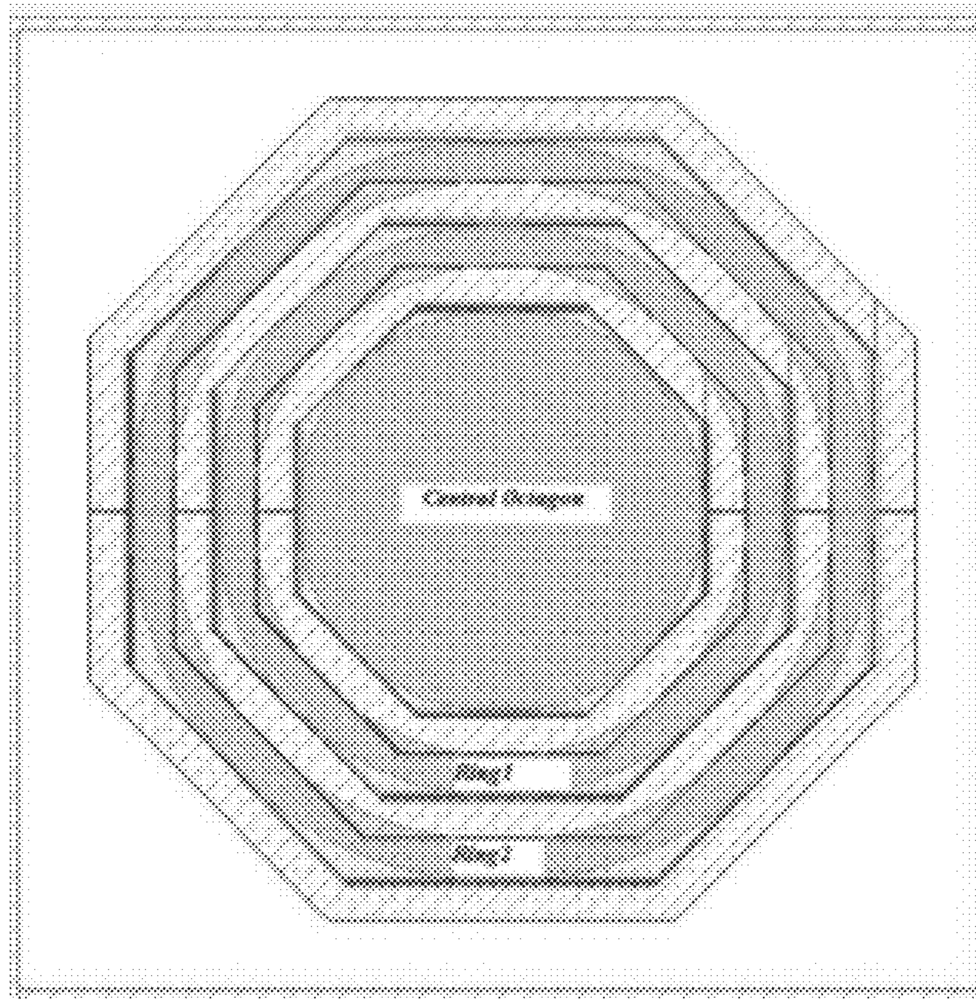
Fig. 14 Concentric rings CMOS SDM optical detector
