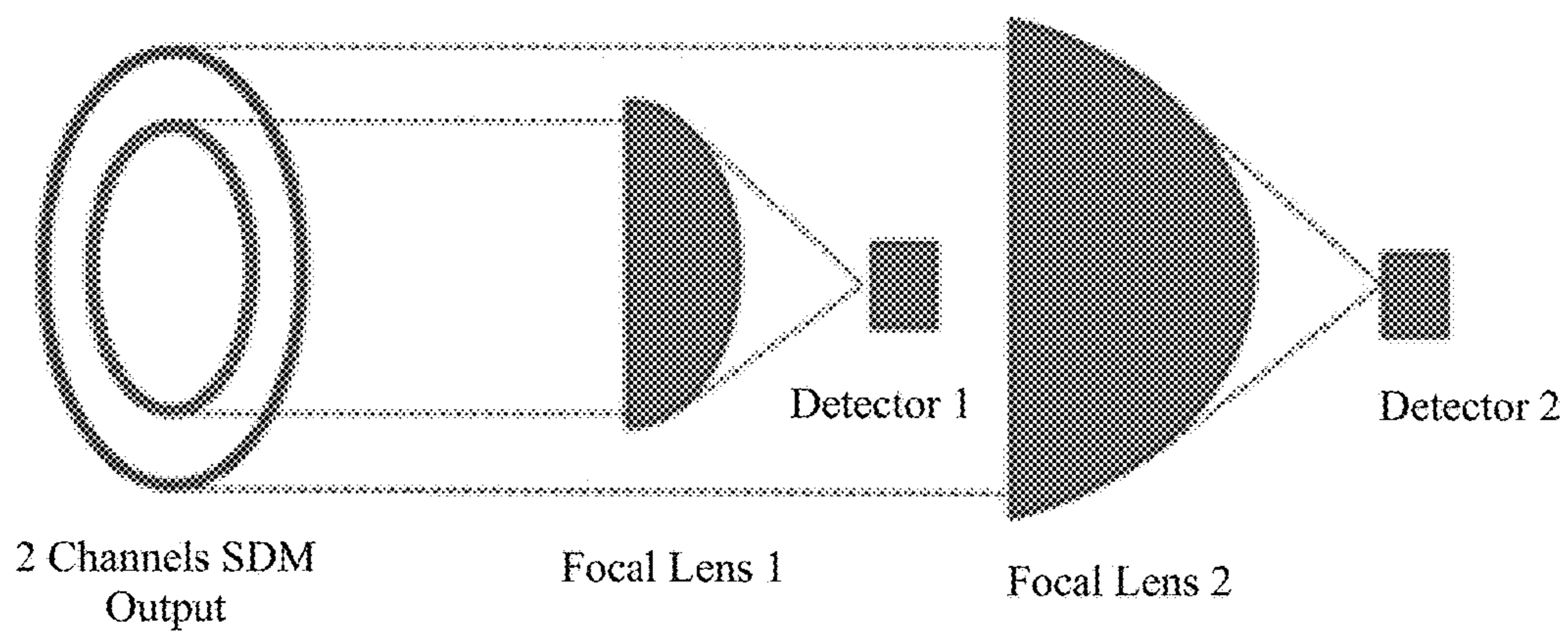
FIG. 13 Bulk lens for de-multiplexing SDM
