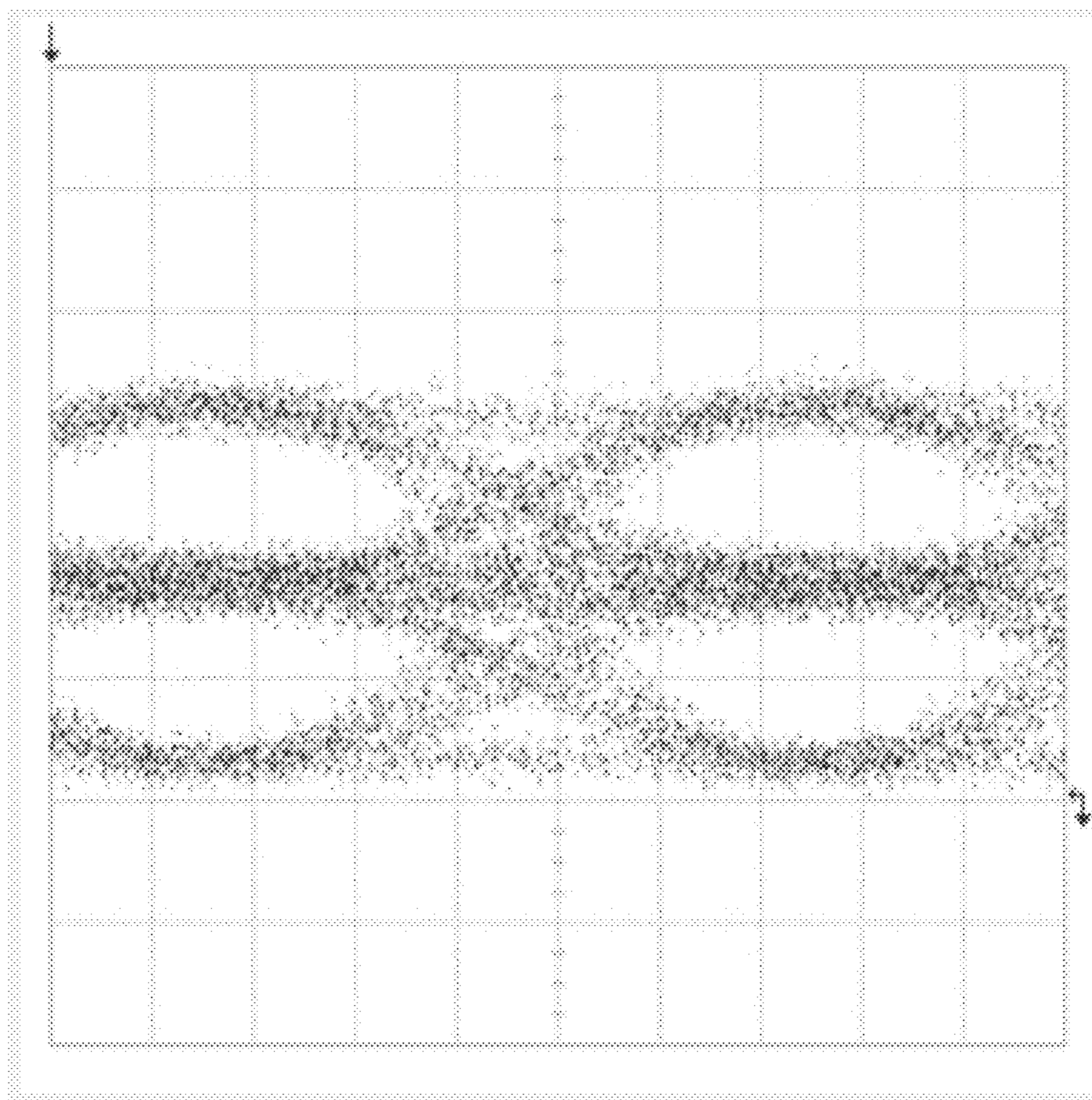
Fig. 23B Eye diagram of PAM-3 system
