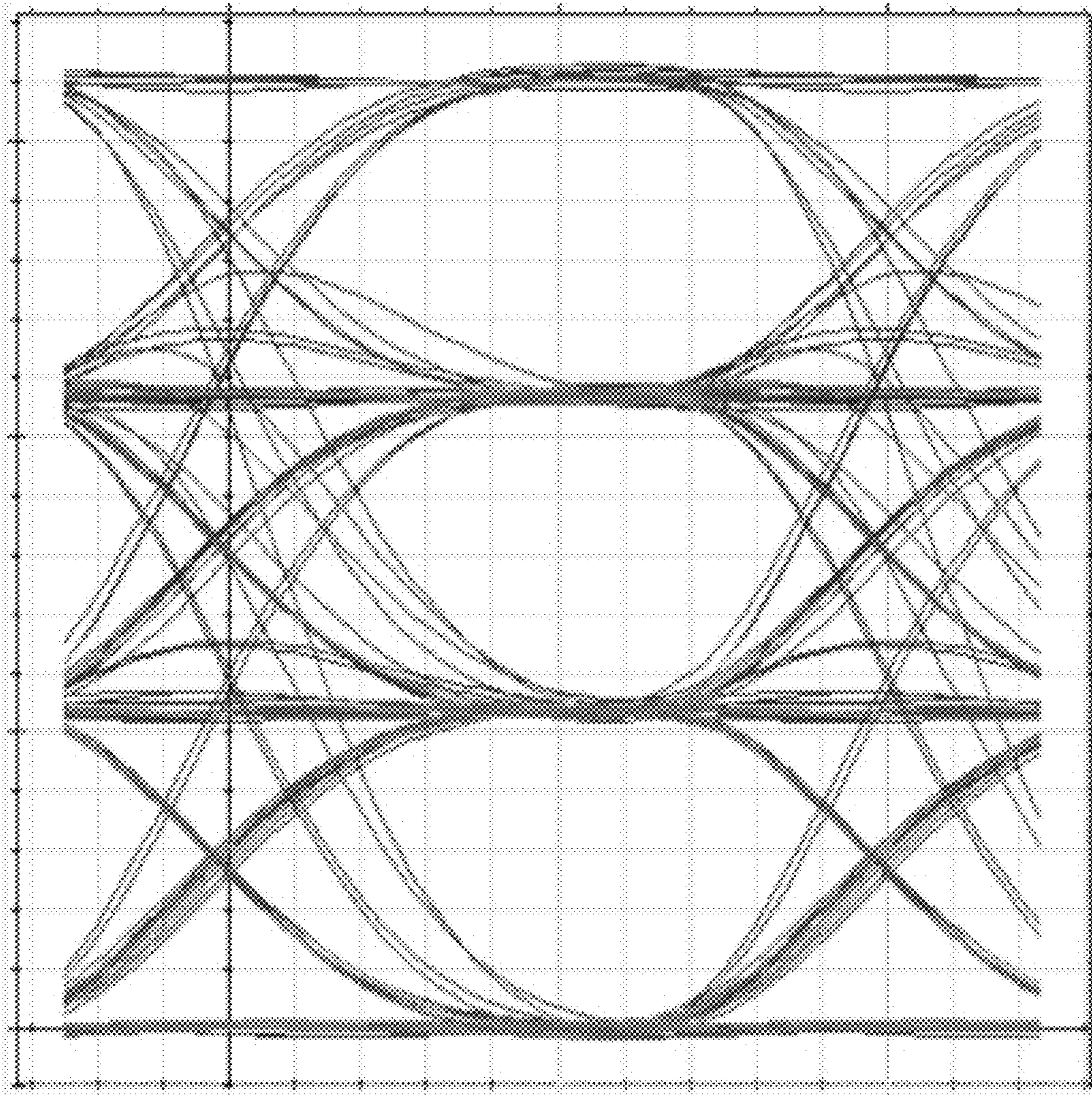
Fig. 26 Simulation results for Modified PAM-4 at 1550nm
