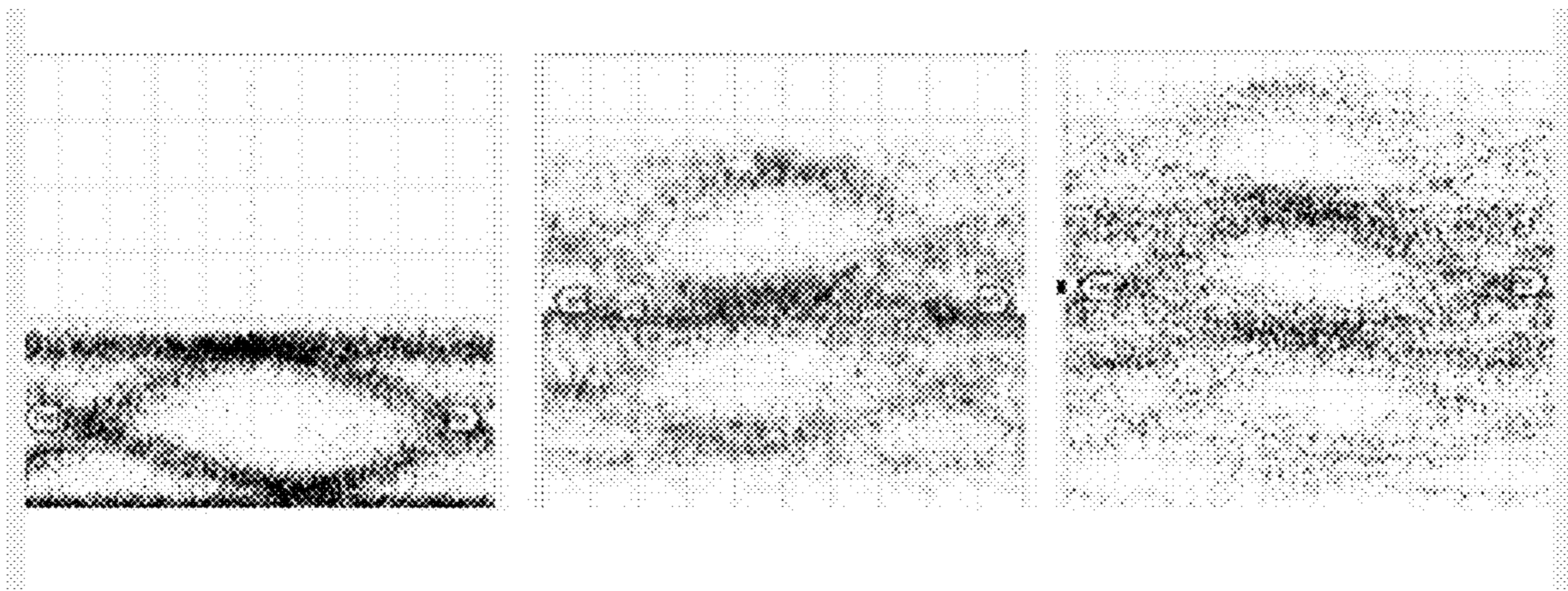
Fig. 35 Eye diagram of PAM-2, PAM-3 and PAM-4 with CWDM
