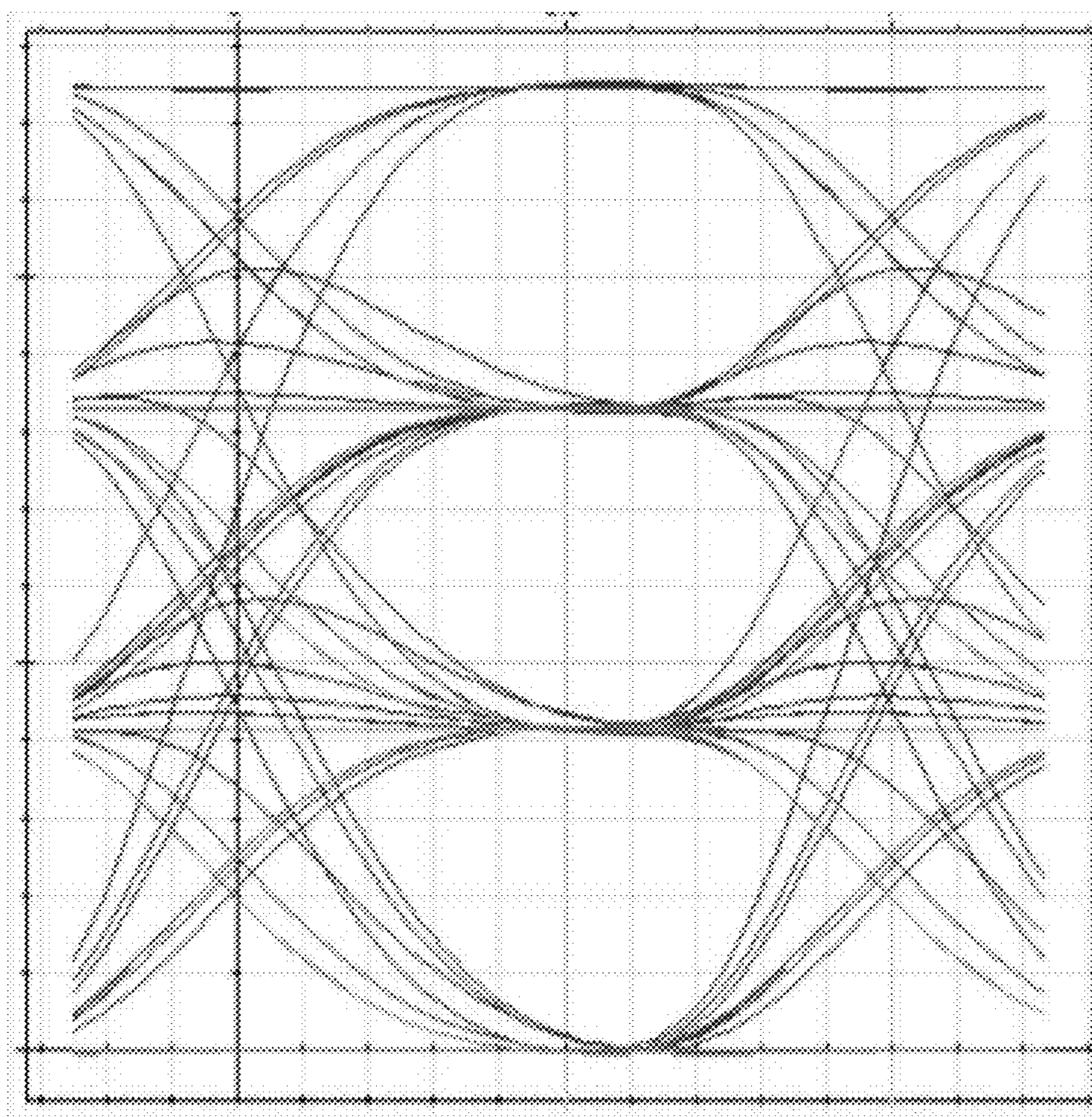
Fig. 24 Simulation results for Modified PAM-4 at 850nm
