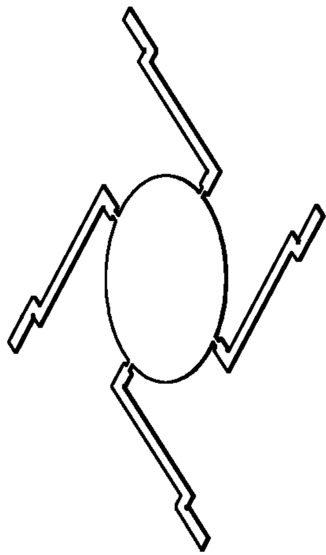
SMA OIS SPRING SHOWN IN THE FLAT STATE
