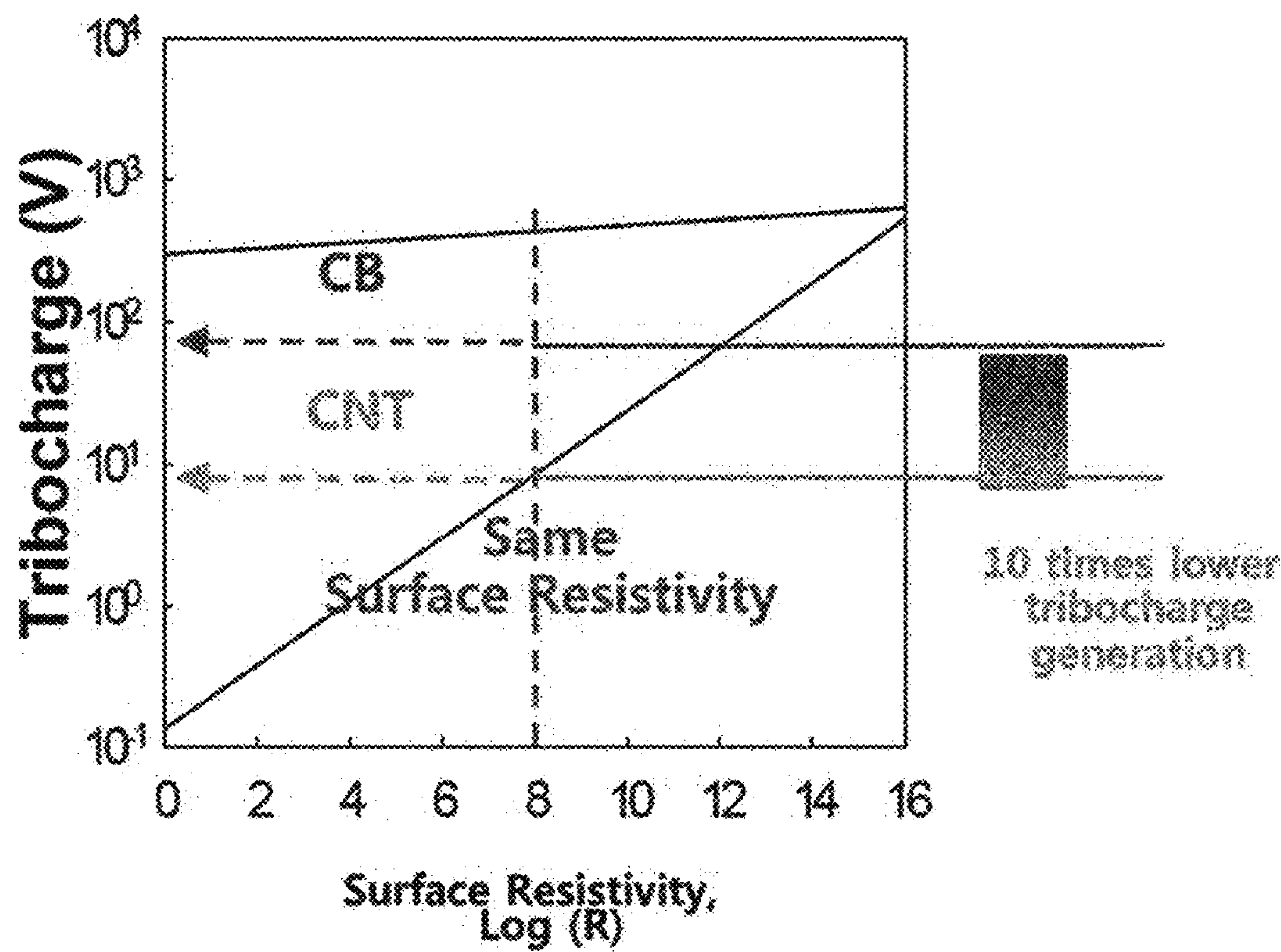
Electrostatic dispersion characteristic of carbon nanotube
