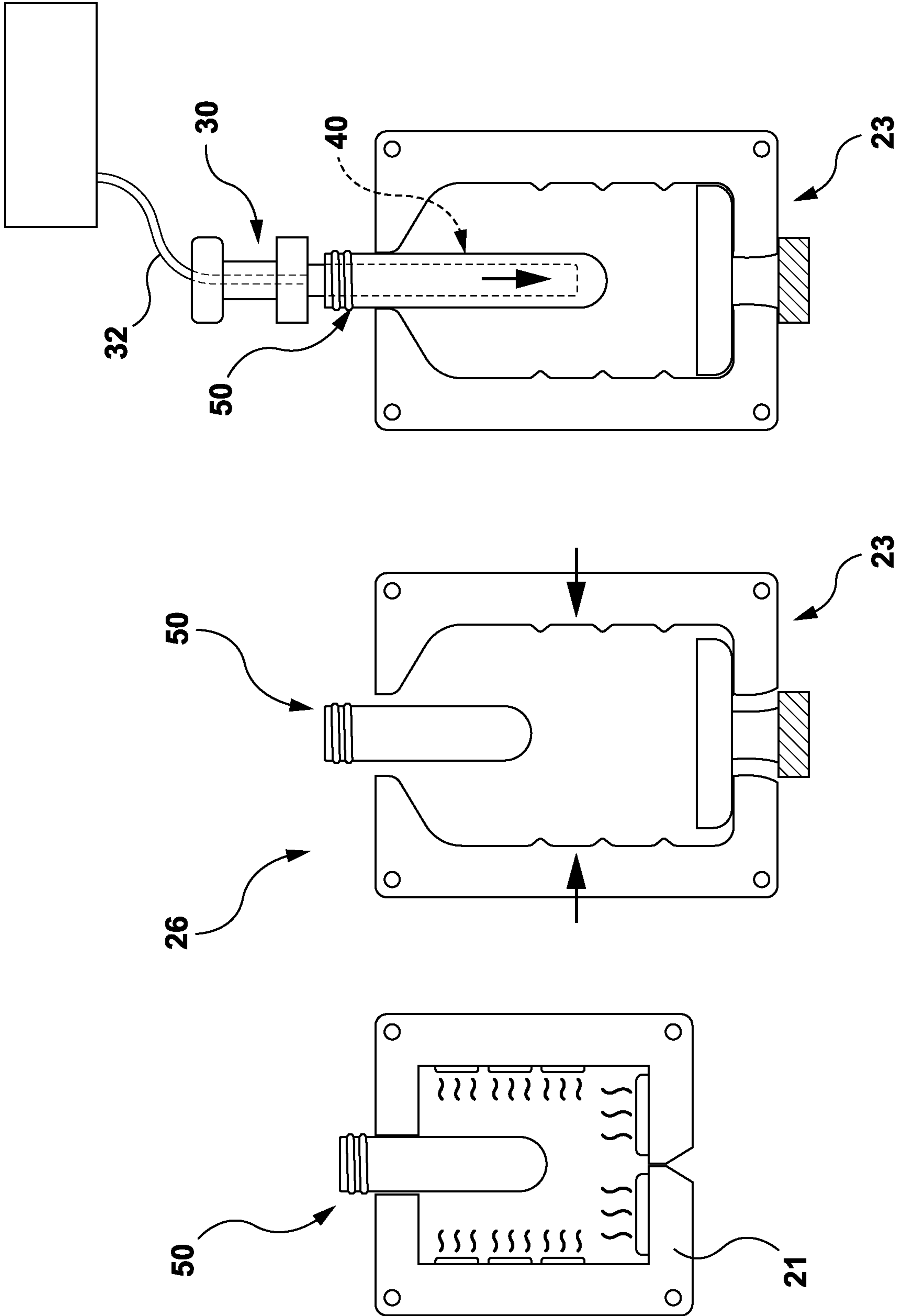
FIG. 1C (PRIOR ART)
