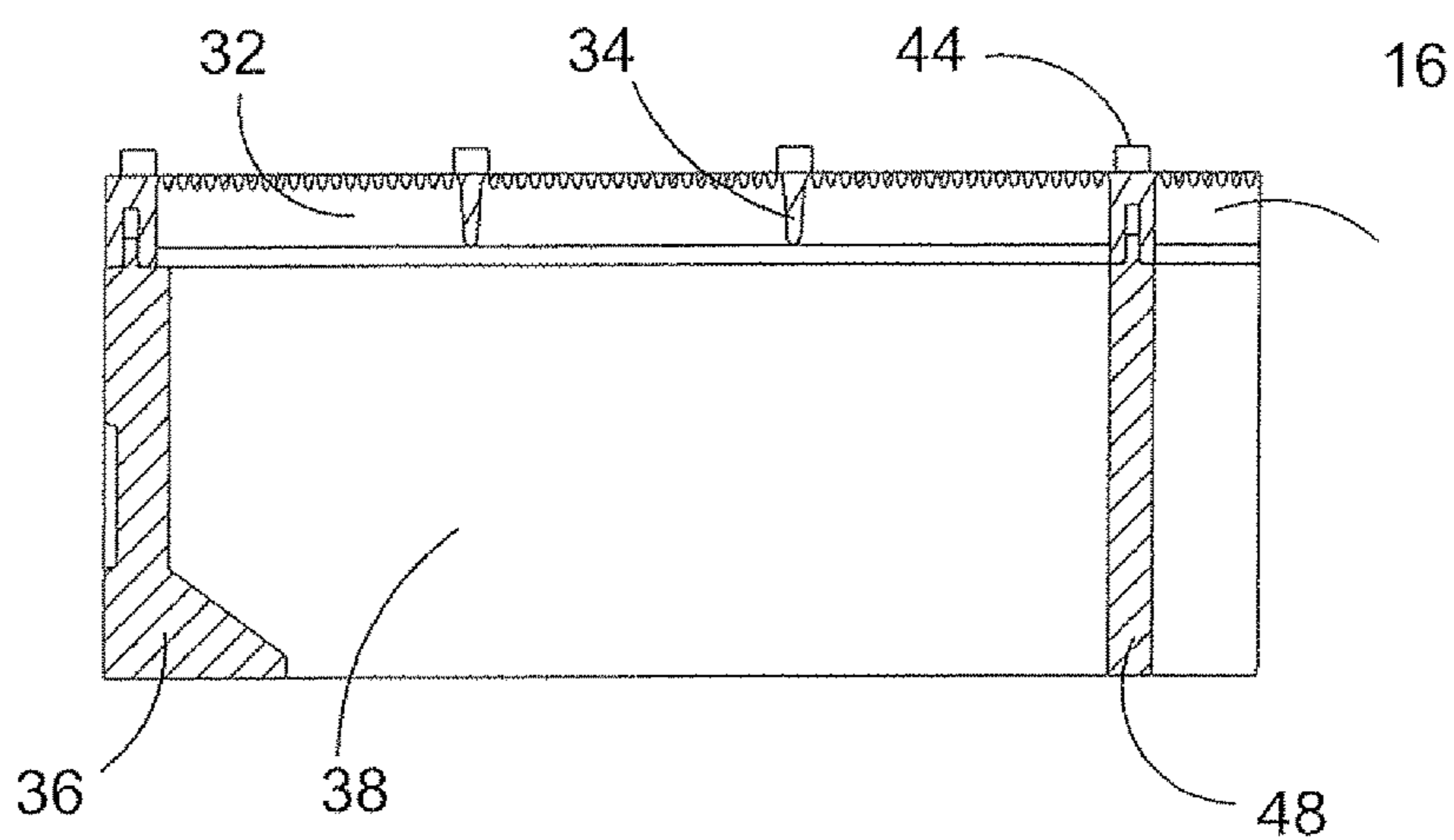
SECTION B-B
