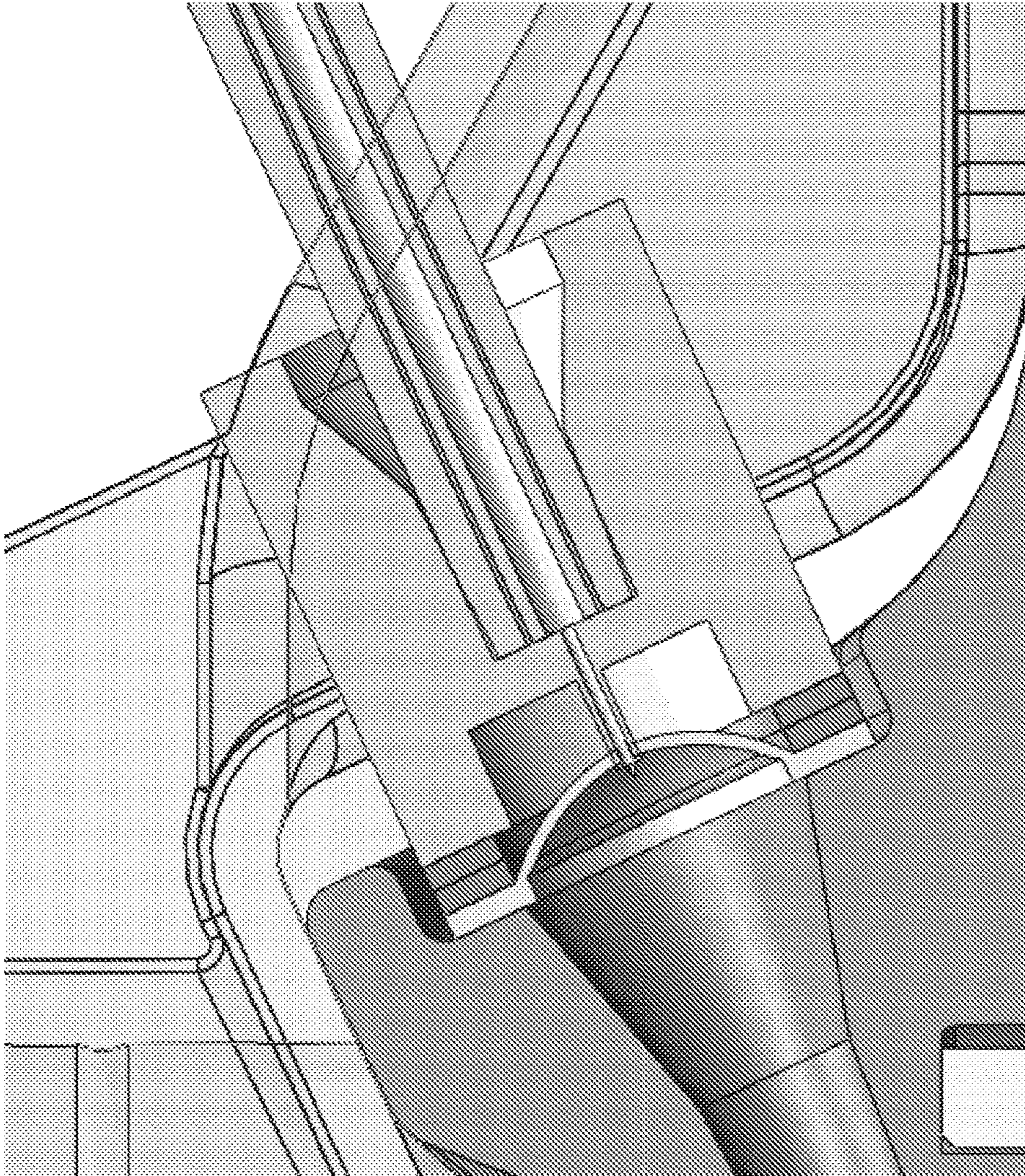
Tubing Connector and Infusion Site Connector Interface
