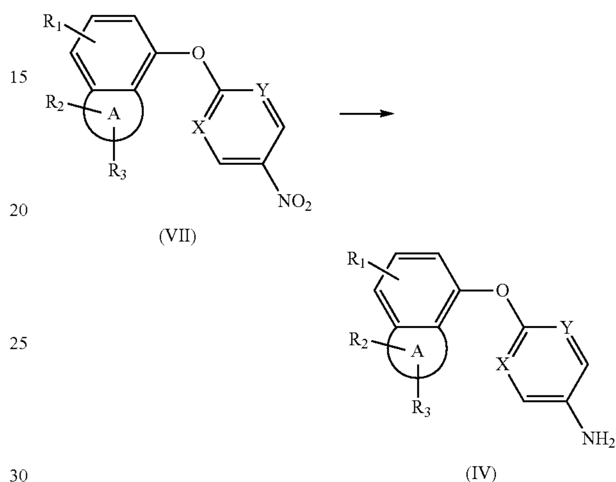
Scheme 3
