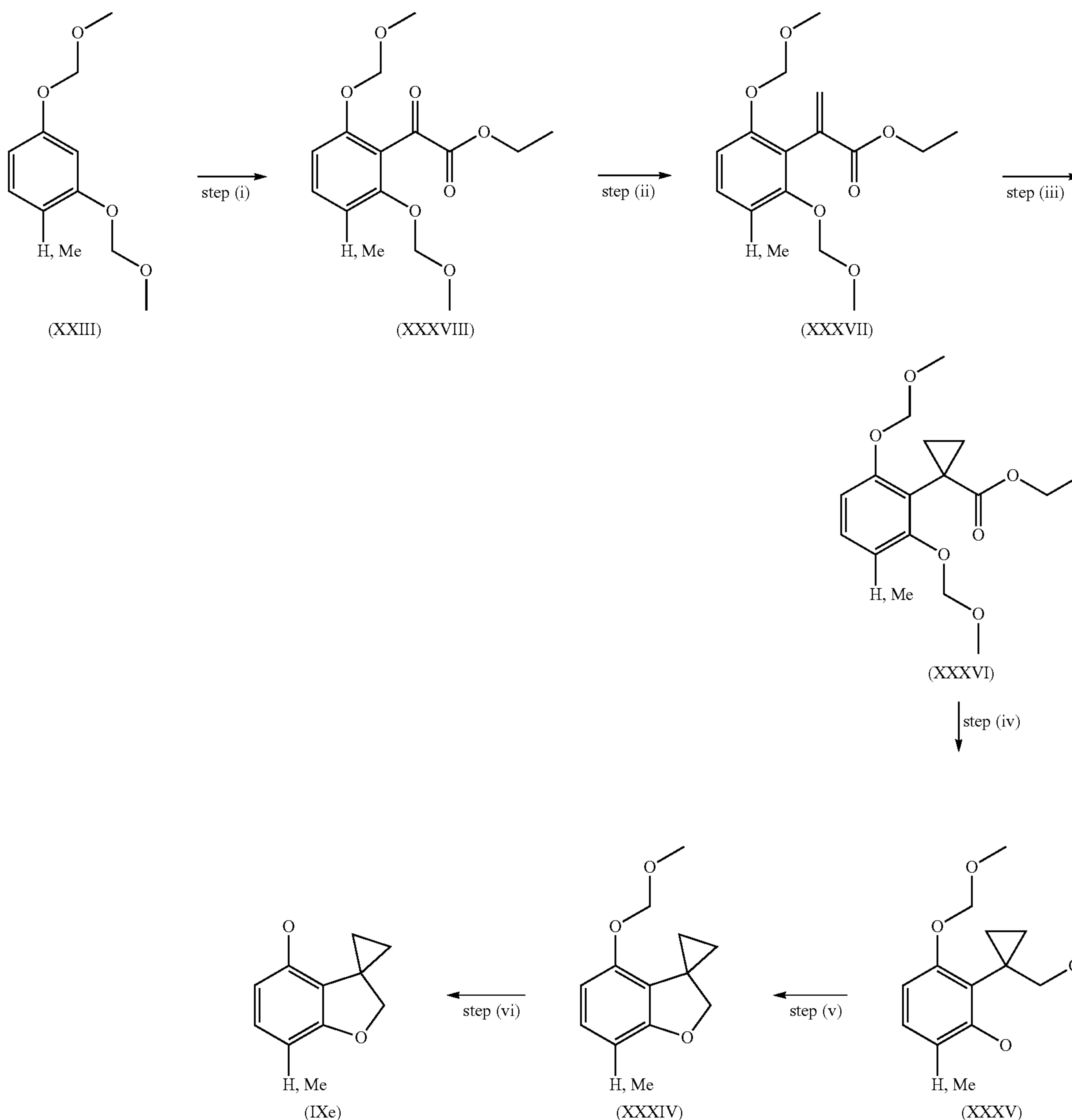
Scheme 16
