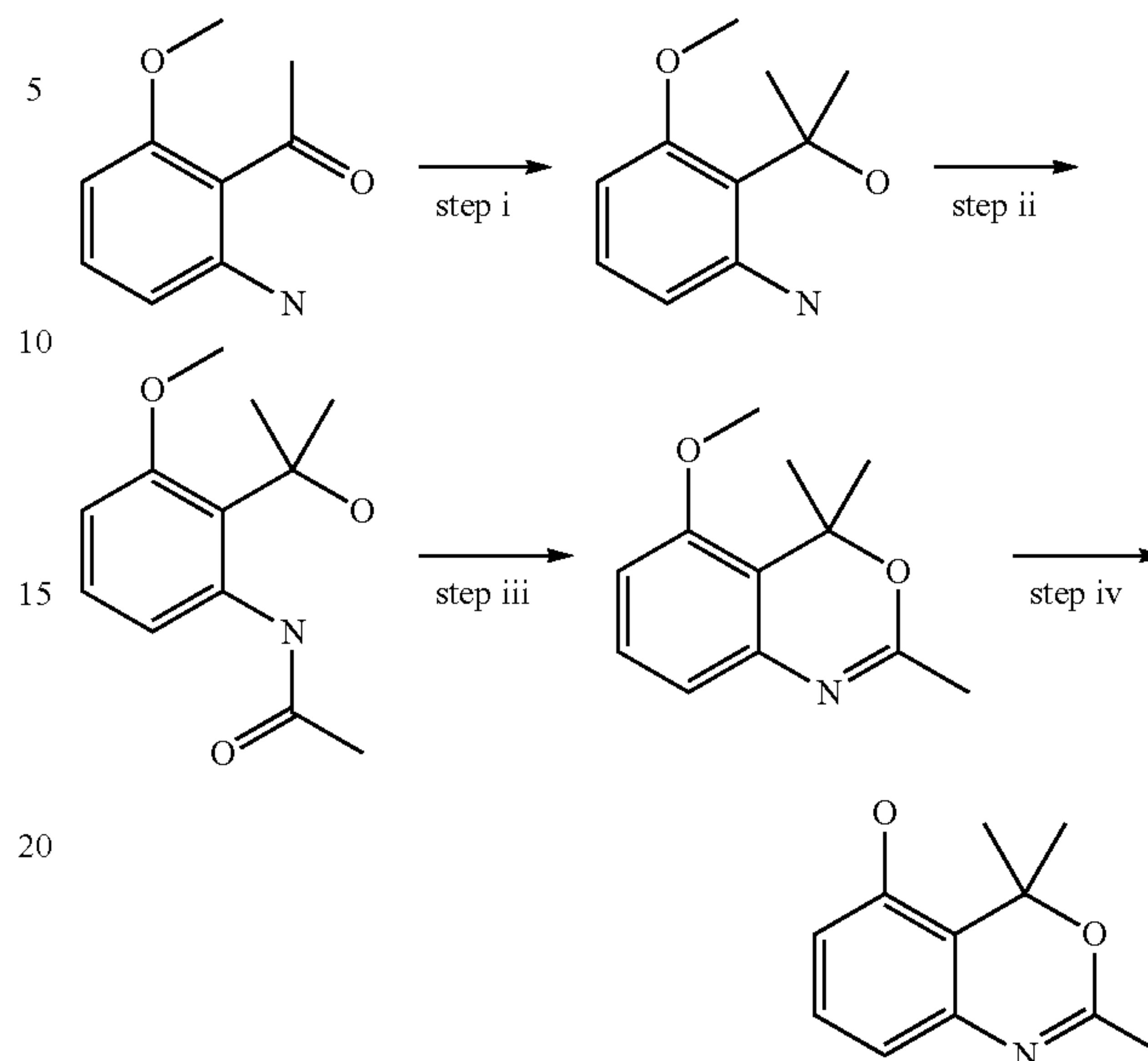
Scheme 24
