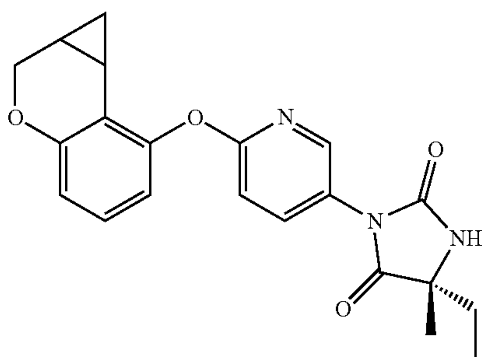
diastereoisomeric 1
