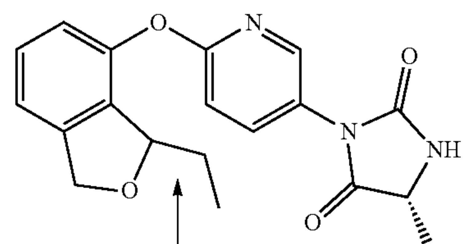
chiral - diastereoisomer 1
