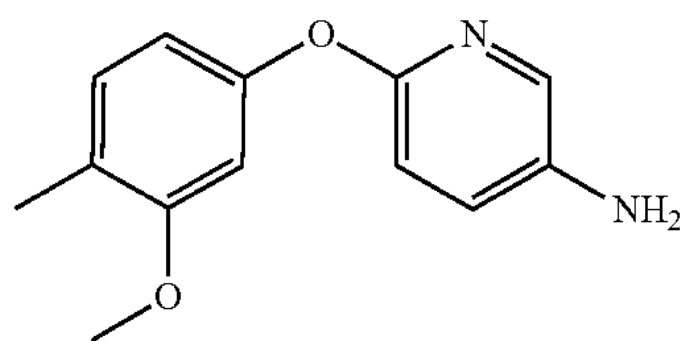
6-{{[4-methyl-3-(methoxy)phenyl]oxy}}-3-pyridinamine
