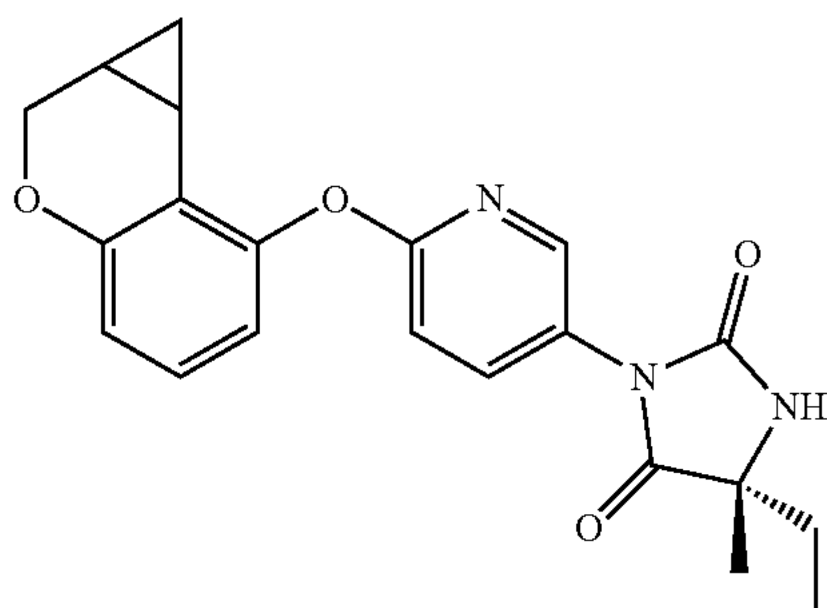
diastereoisomer 2
