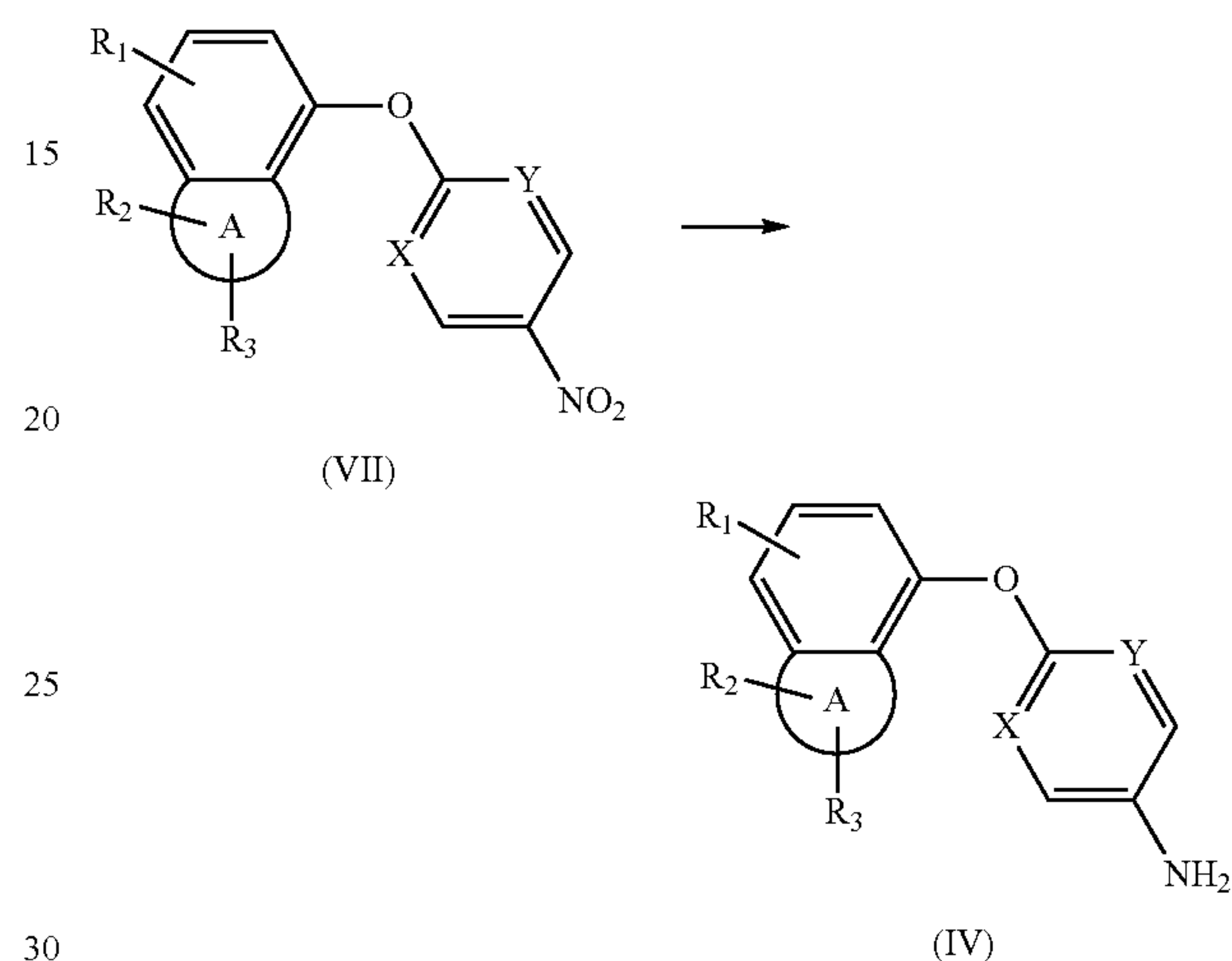
Scheme 3
