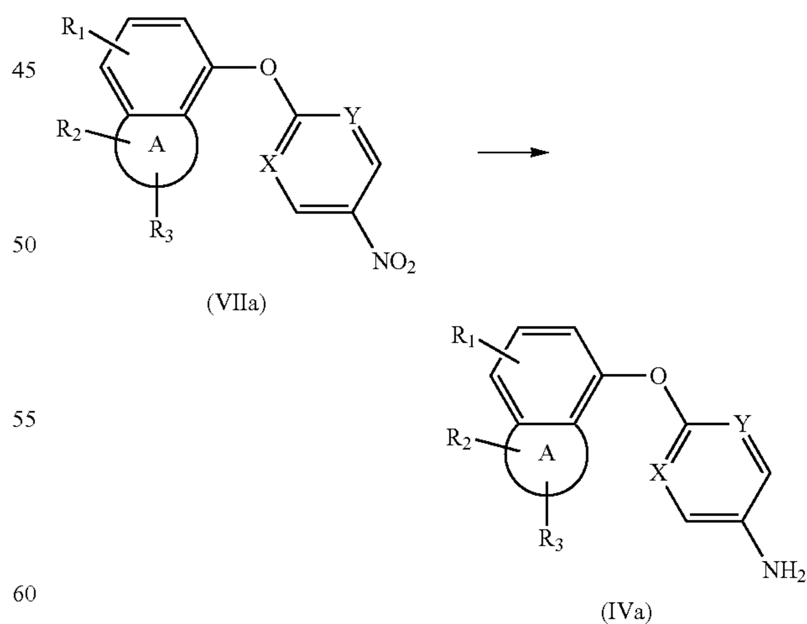
Scheme 4
