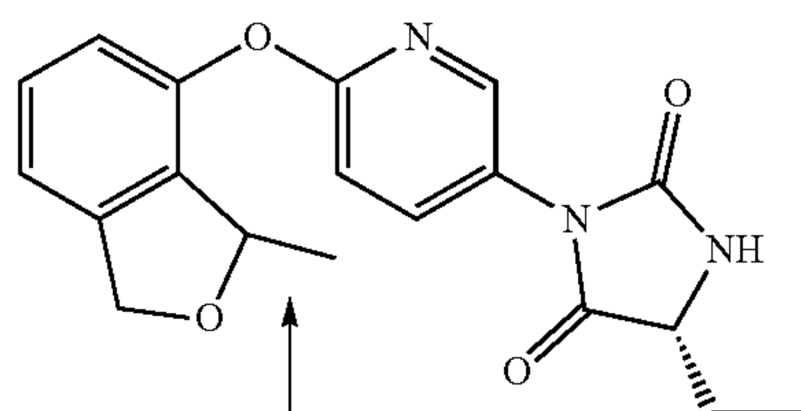
chiral - diastereoisomer 1
