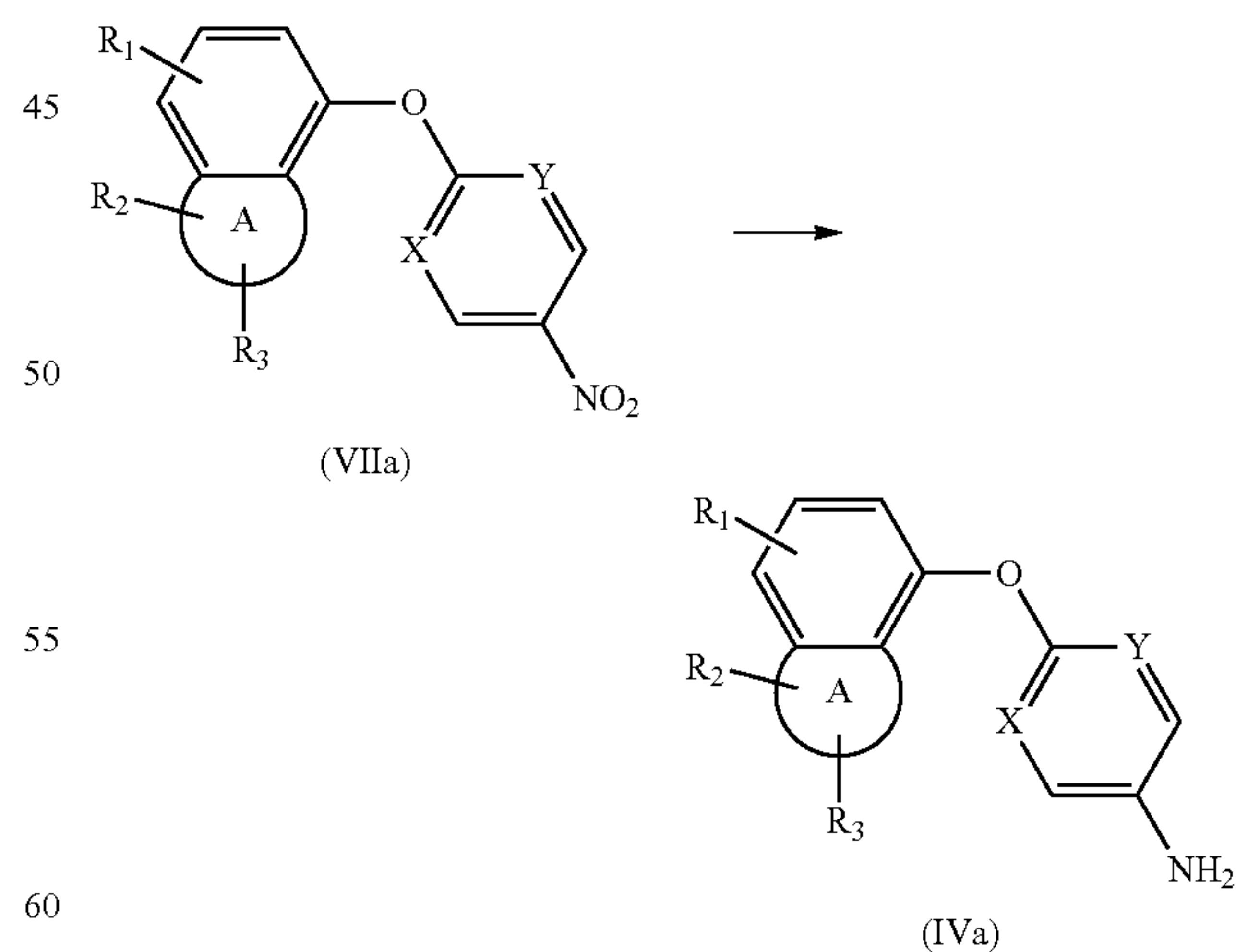
Scheme 4
