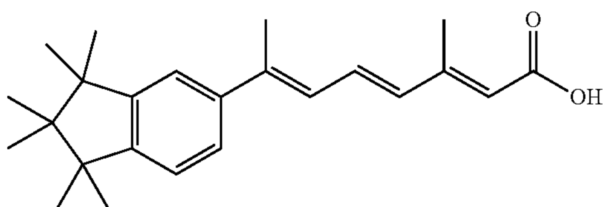
(2E,4E,6E)-7-(1,1,2,2,3,3-hexamethyl-2,3-dihydro-1H-inden-5-yl)-3-methylocta-2,4,6-trienoic acid
