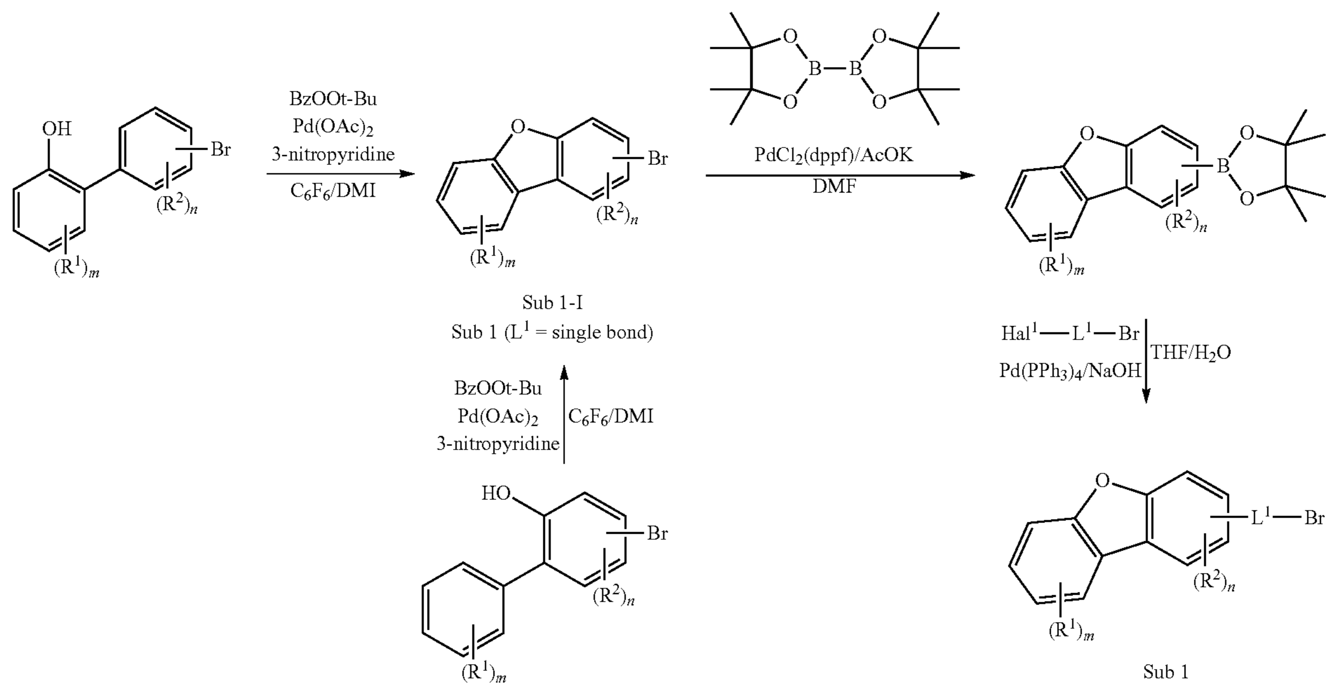
&lt;Reaction Scheme 2&gt;
