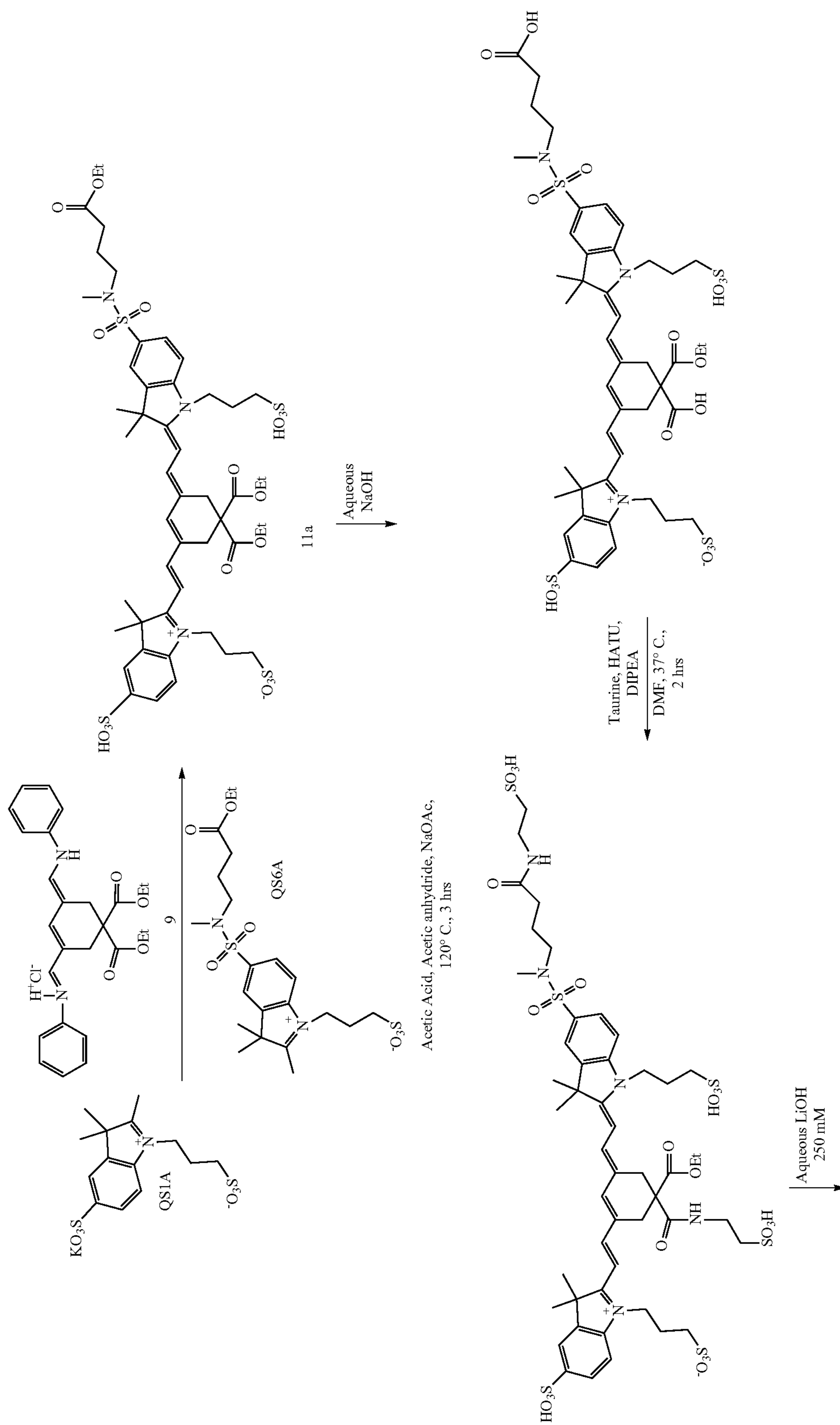
Scheme 3T. Synthesis of Asymmetric Indolinium Dye
