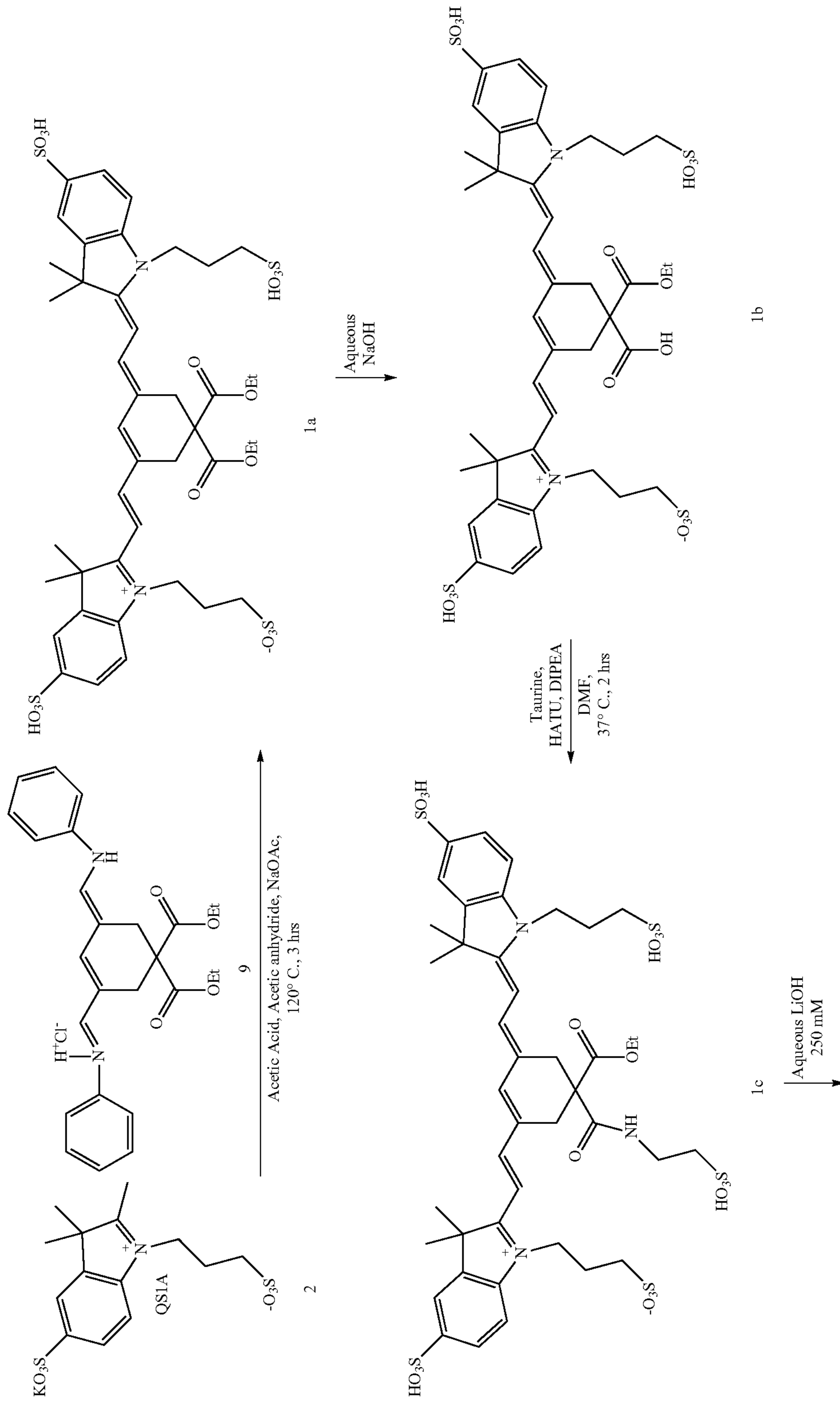
Scheme 3A. Synthesis of Symmetric Indolinium Hydrophilic Dye
