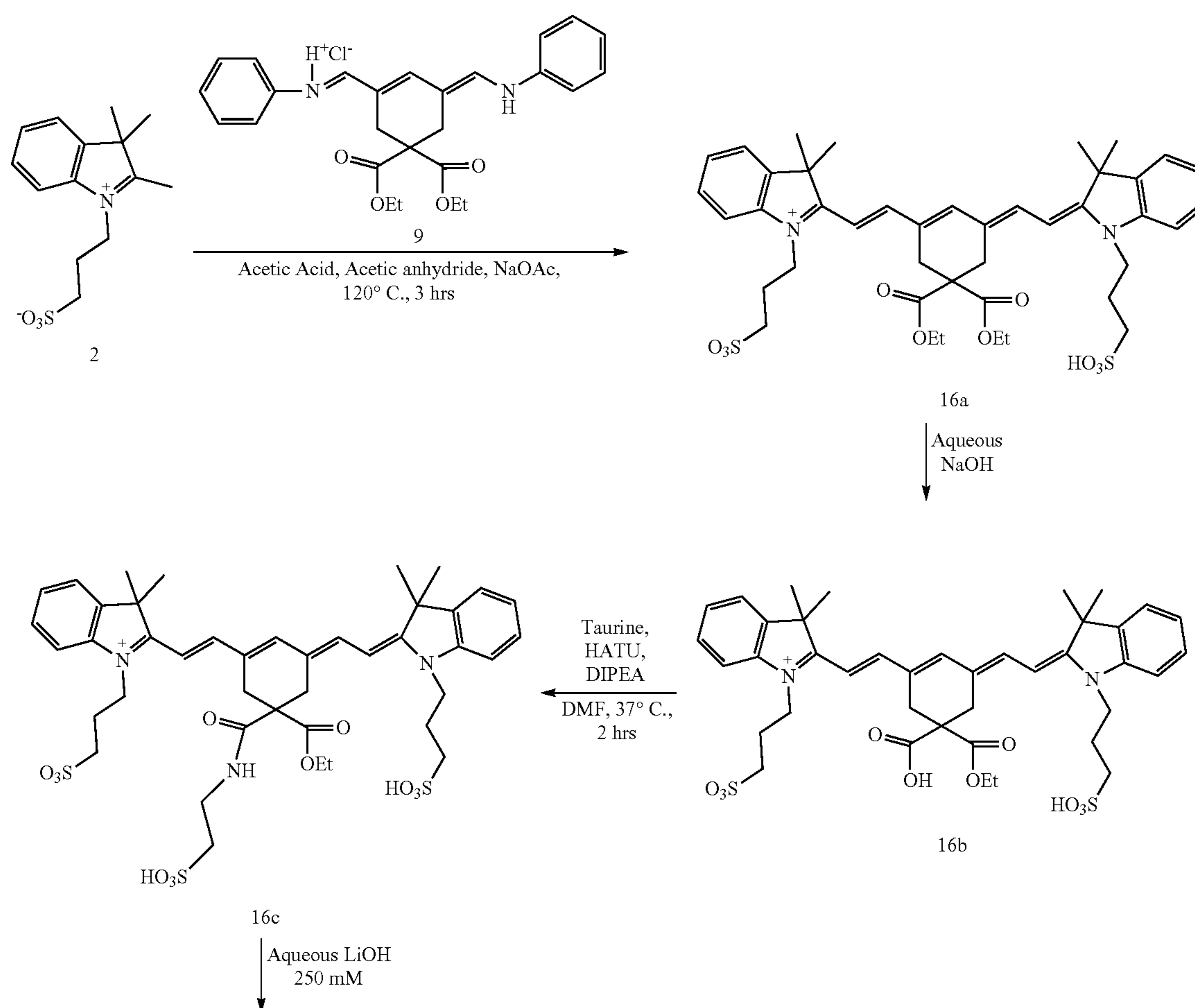
Scheme 3Q. Synthesis of Symmetric Indolinium Dye
