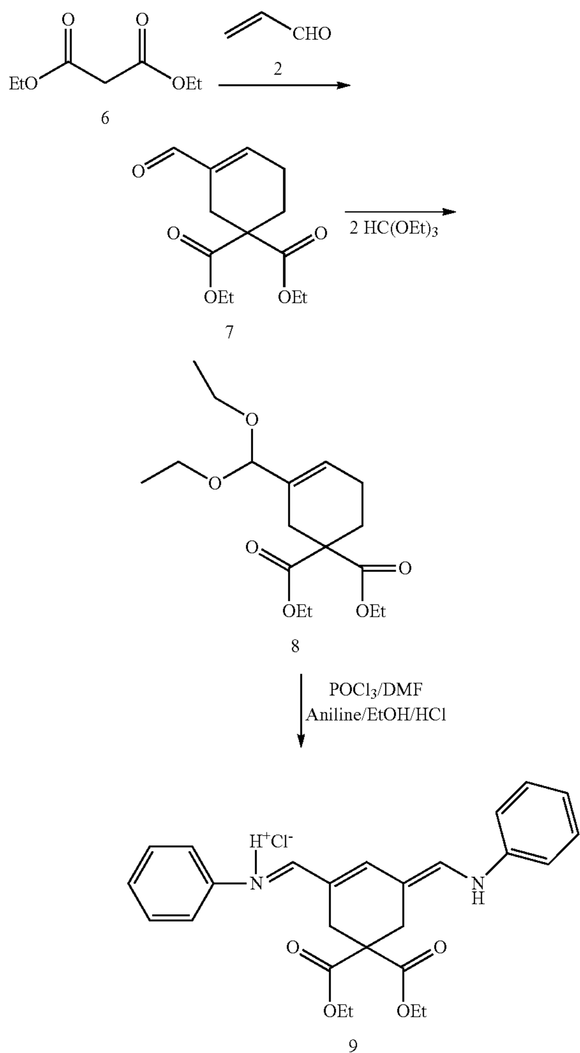
Scheme 2. Preparation of Bridge
