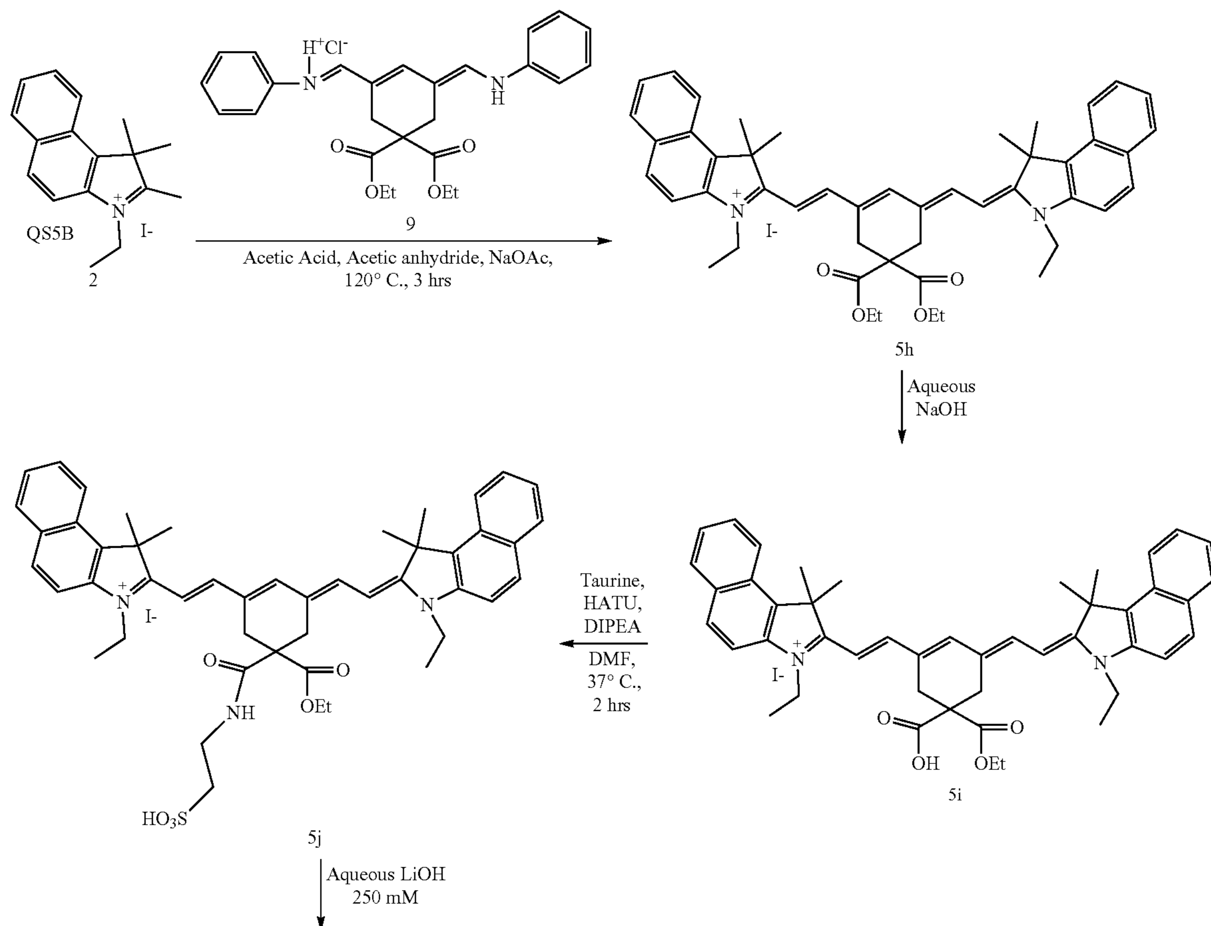
Scheme 3J. Synthesis of Symmetric Benzindole Dye
