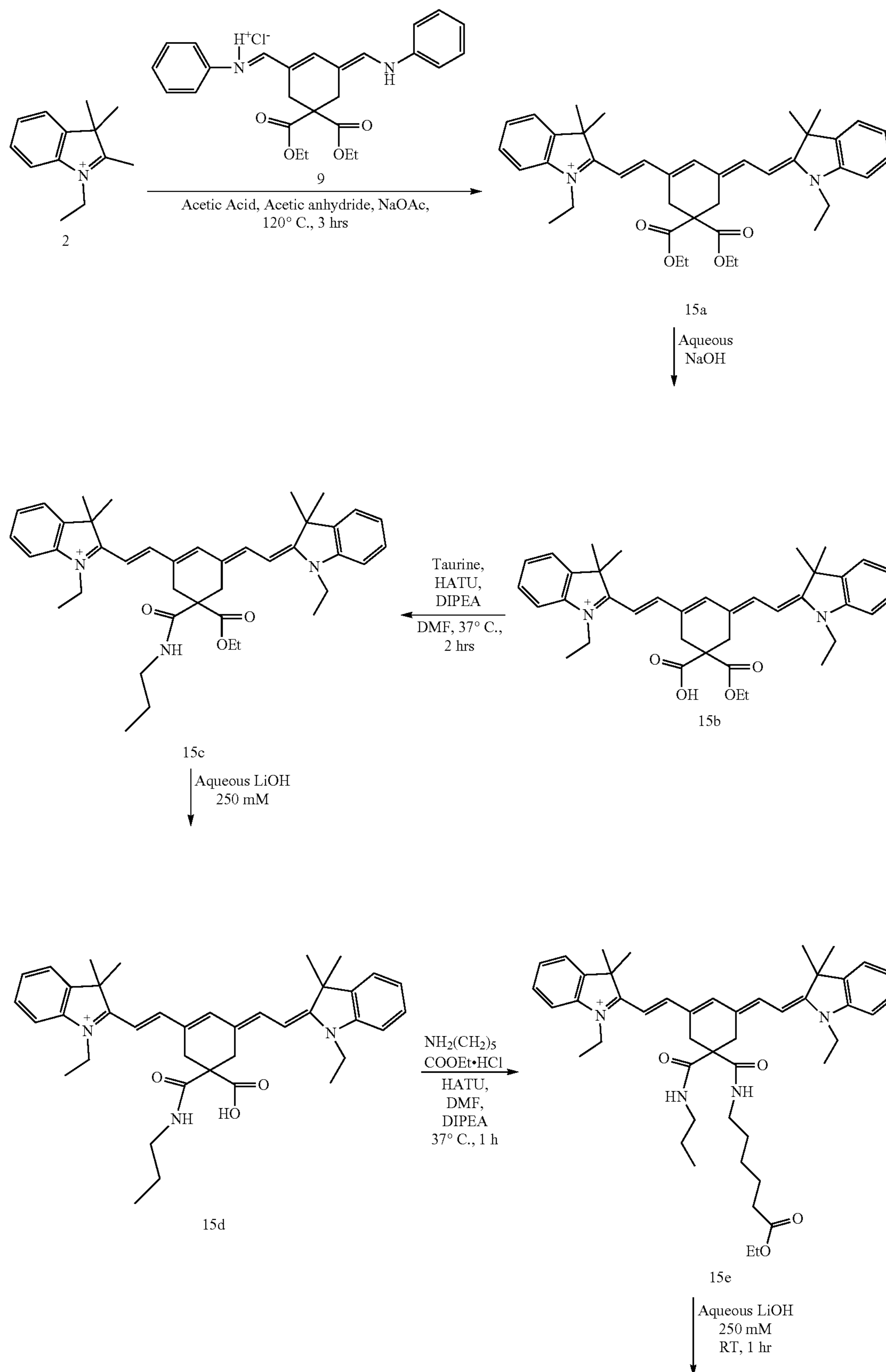
Scheme 3P. Synthesis of Symmetric Indolinium Hydrophobic Dye
