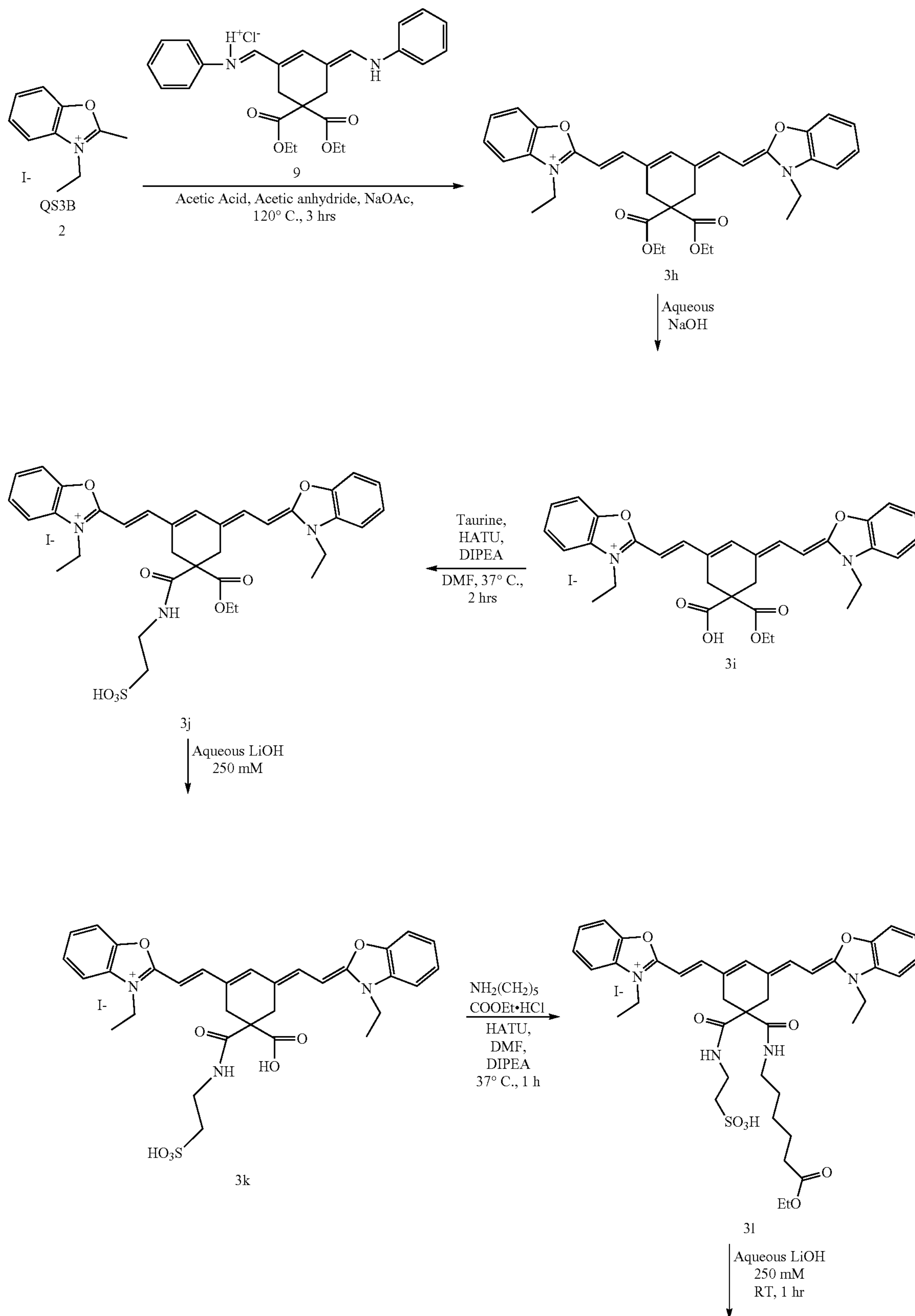
Scheme 3F. Synthesis of Symmetric Benzothiazolium Dye
