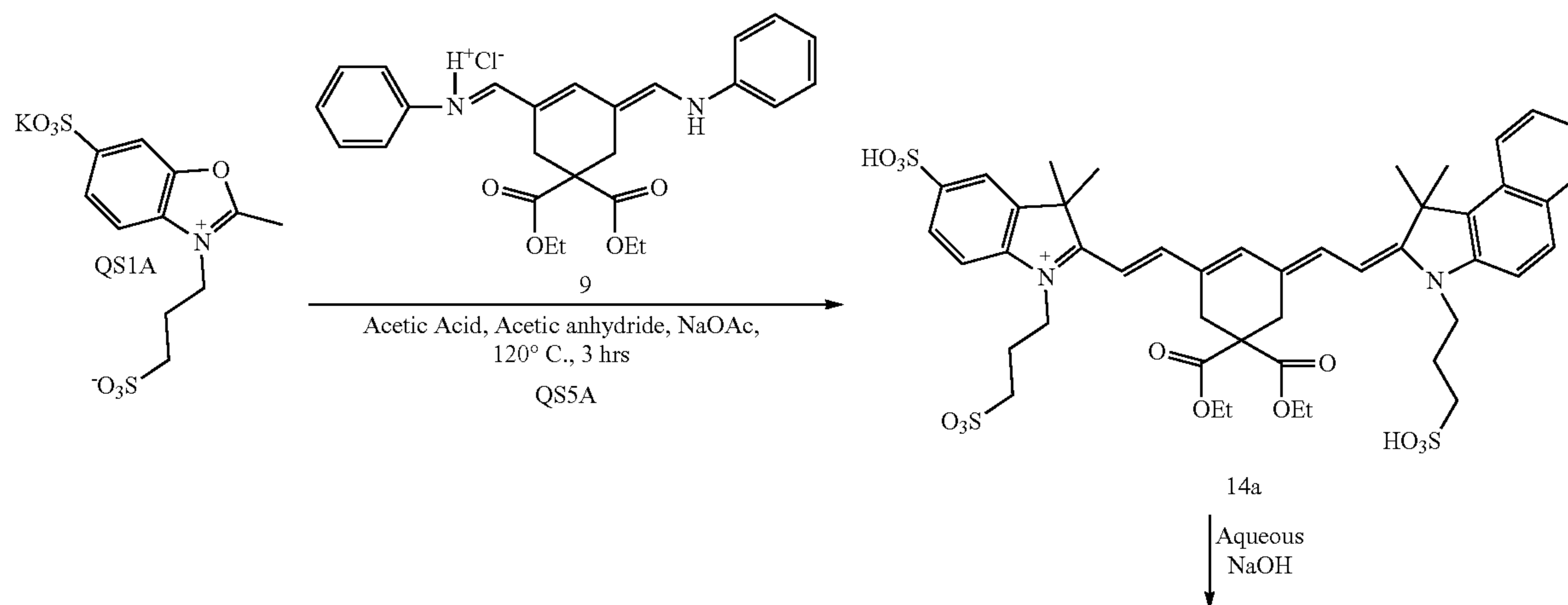
Scheme 3N. Synthesis of Asymmetric Indolinium - Benzindolium Dye
