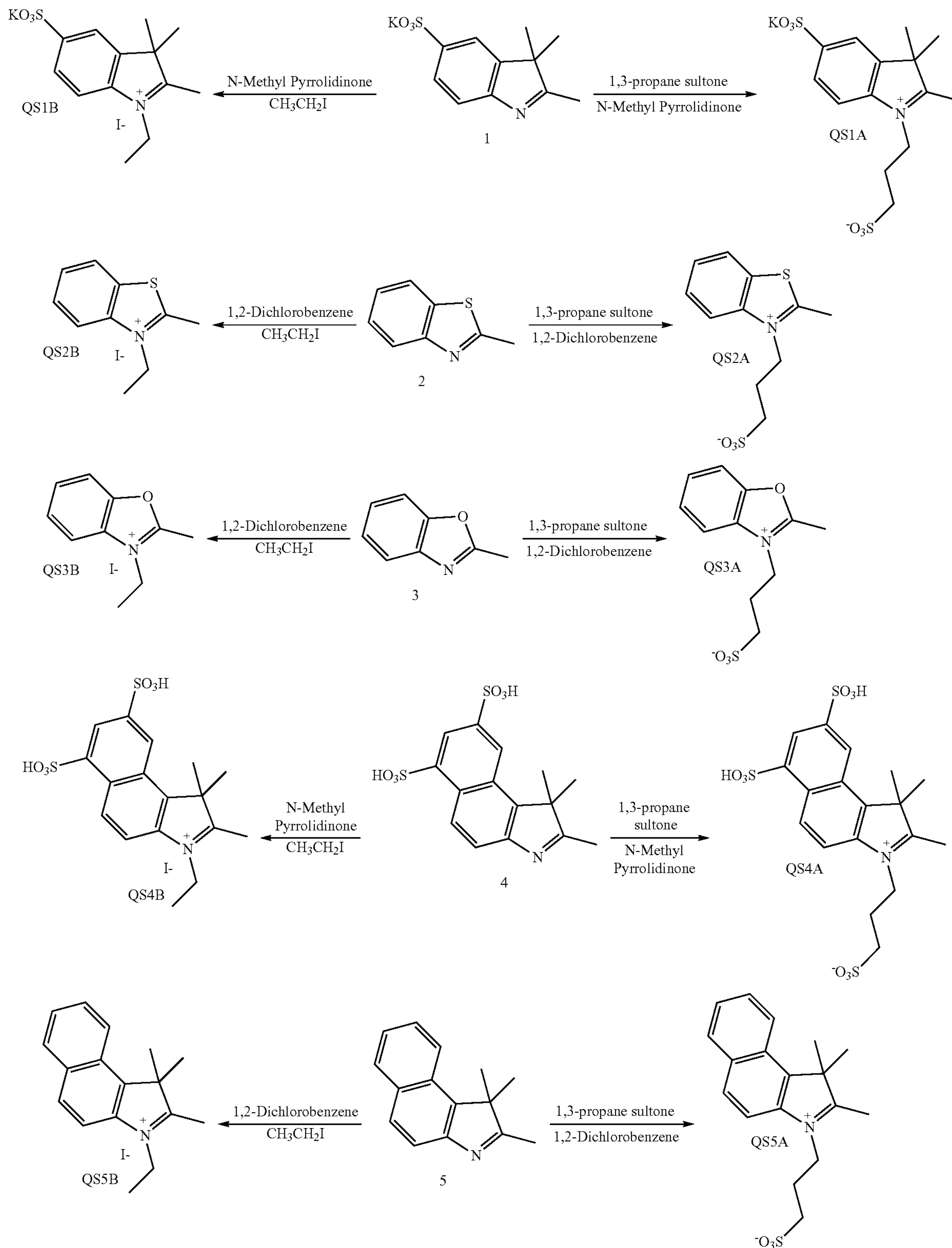
Scheme 1. Preparation of Quaternary Salts
