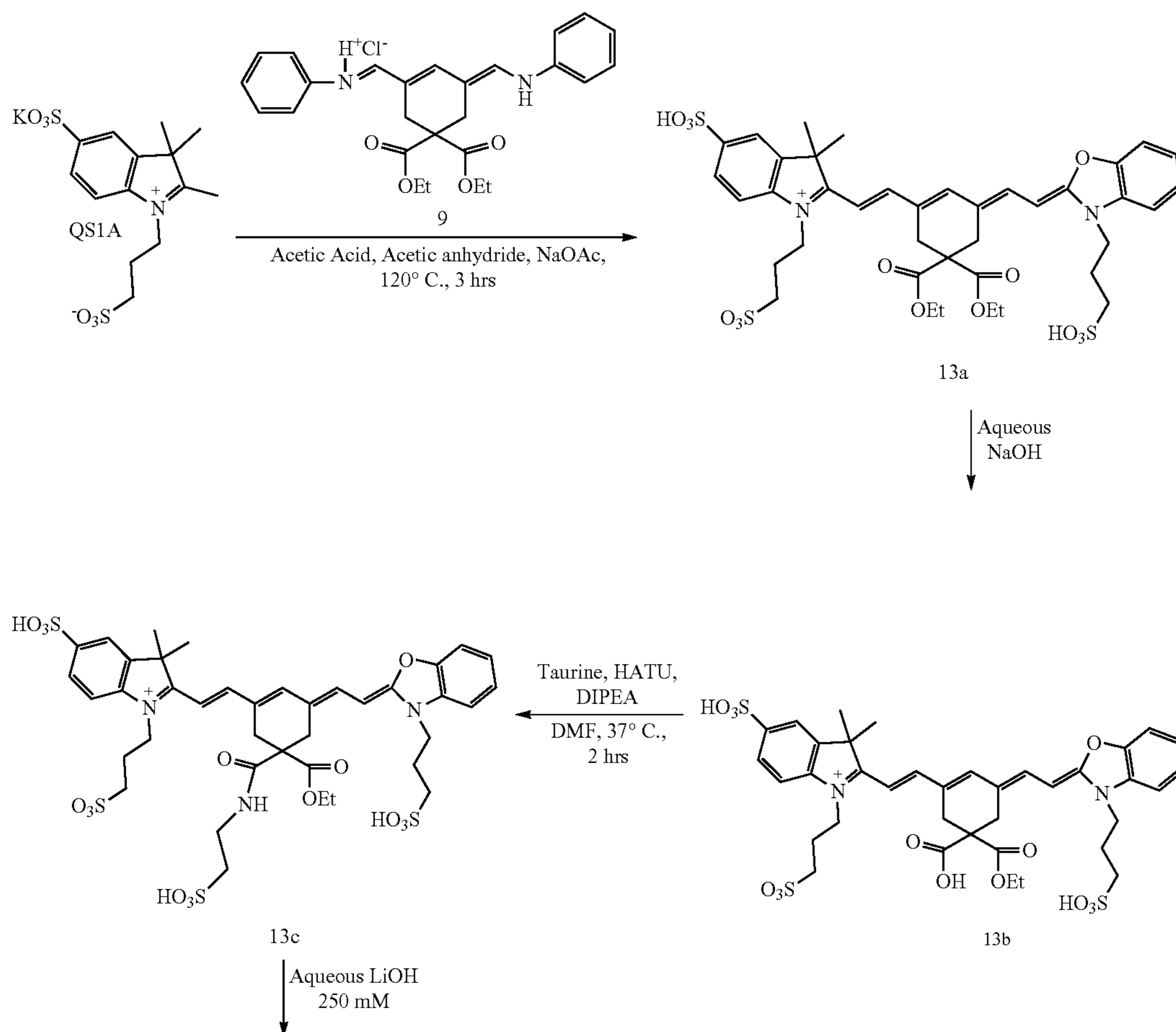
Scheme 3M. Synthesis of Asymmetric Indolinium - Bezoxazole Dye
