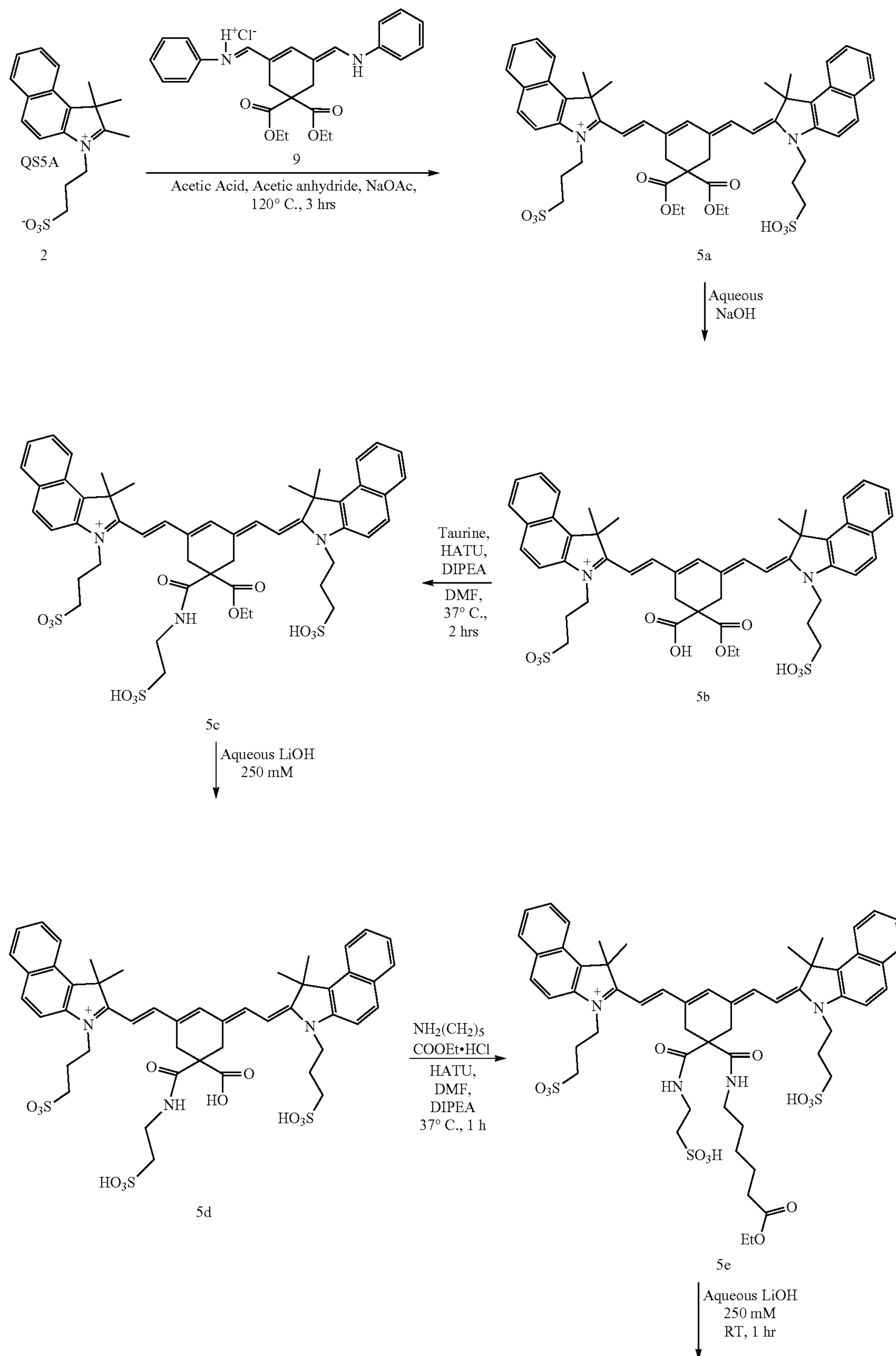
Scheme 3I. Synthesis of Symmetric Benzindole Dye
