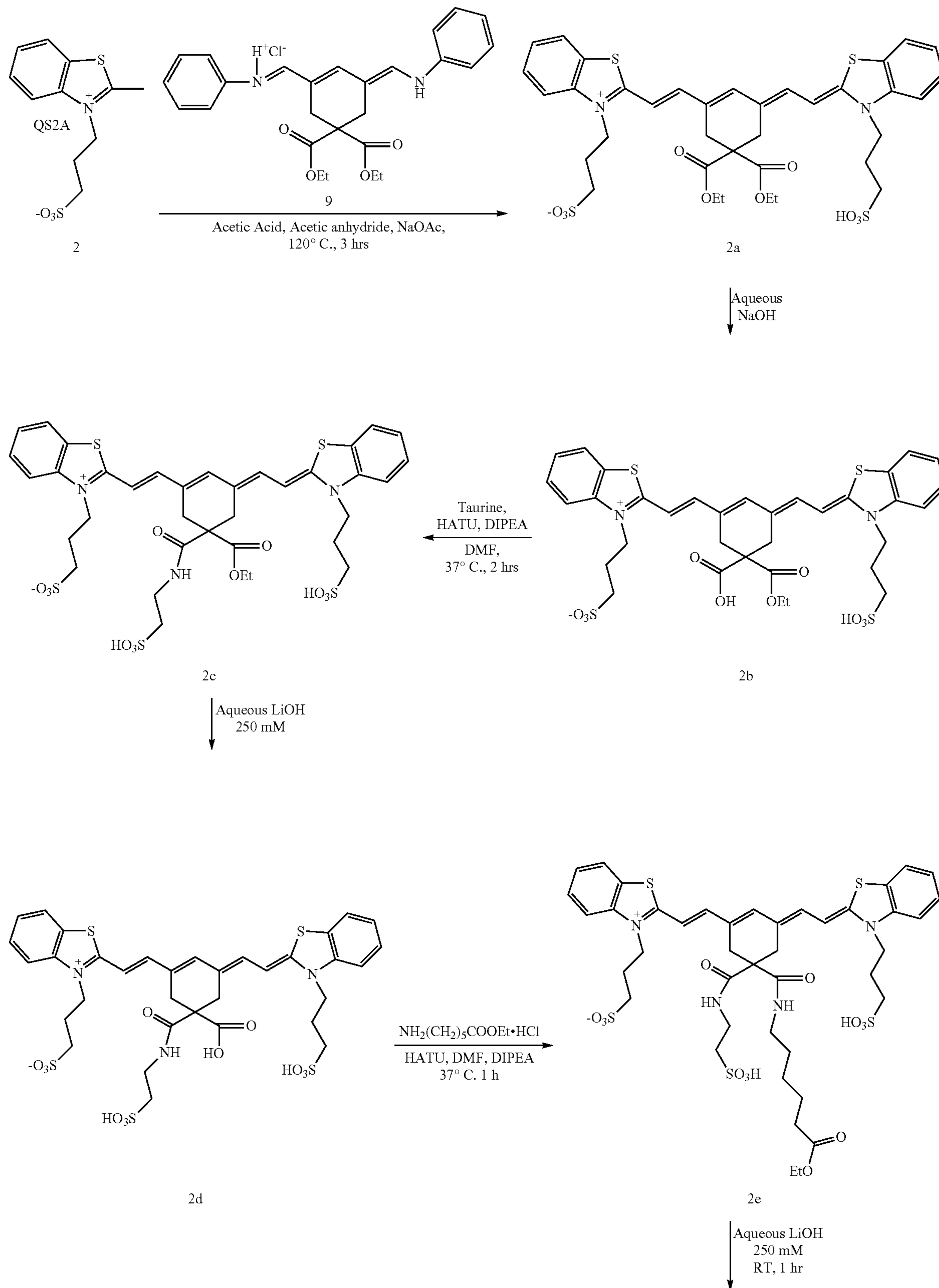
Scheme 3C. Synthesis of Symmetric Benzothiazolium Dye
