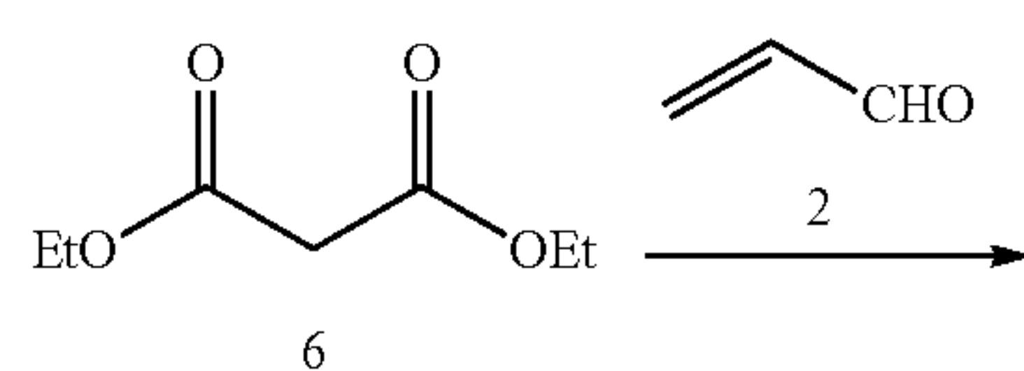
Scheme 2. Preparation of Bridge
