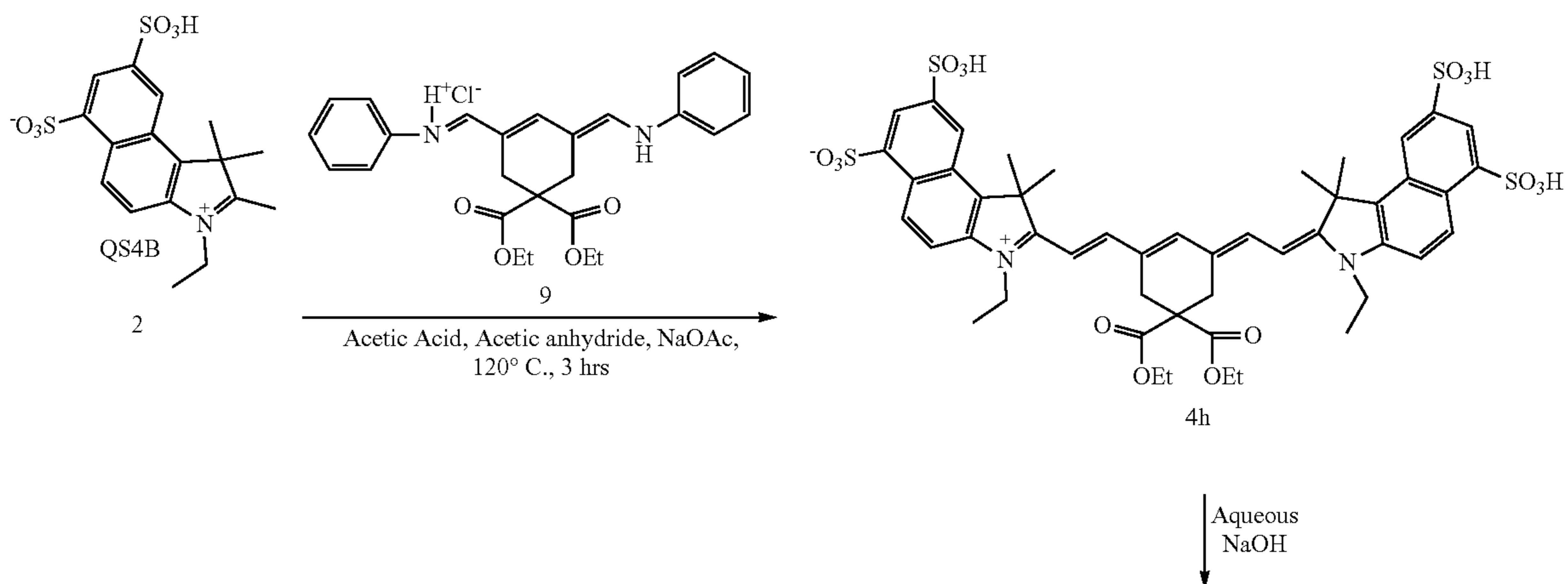
Scheme 3H. Synthesis of Symmetric Benzindole Dye
