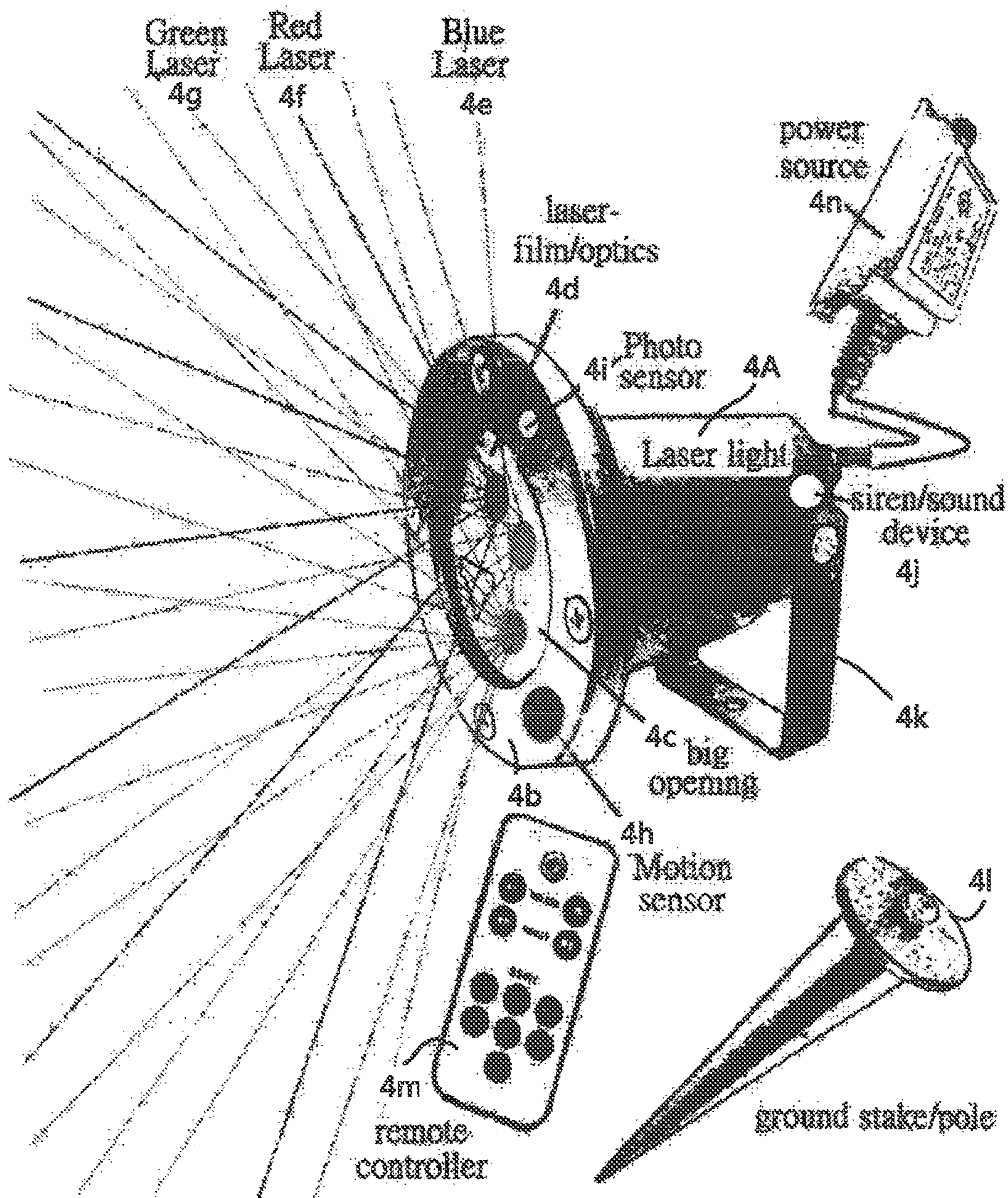
Garden light application with ground stake into soil
