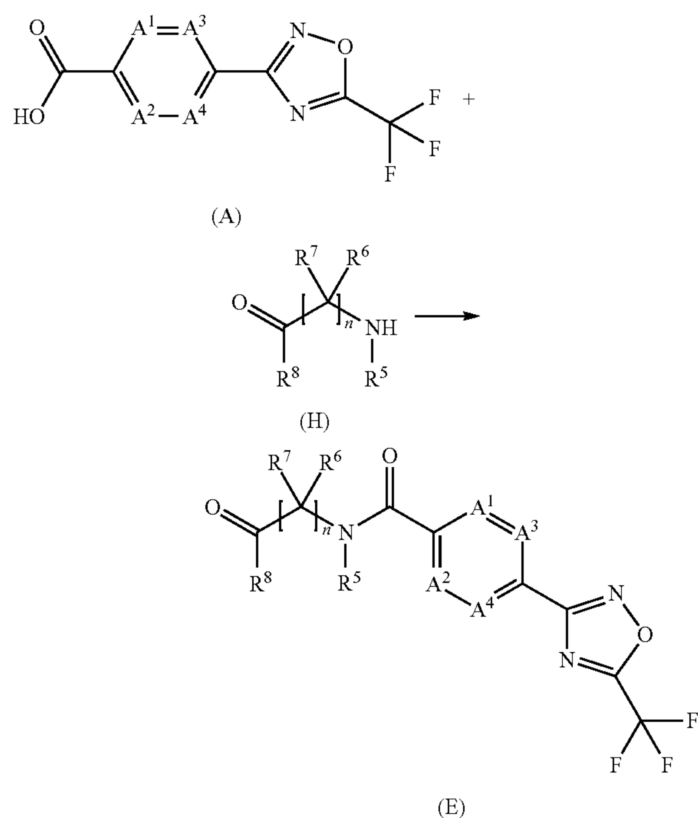
Scheme 7
