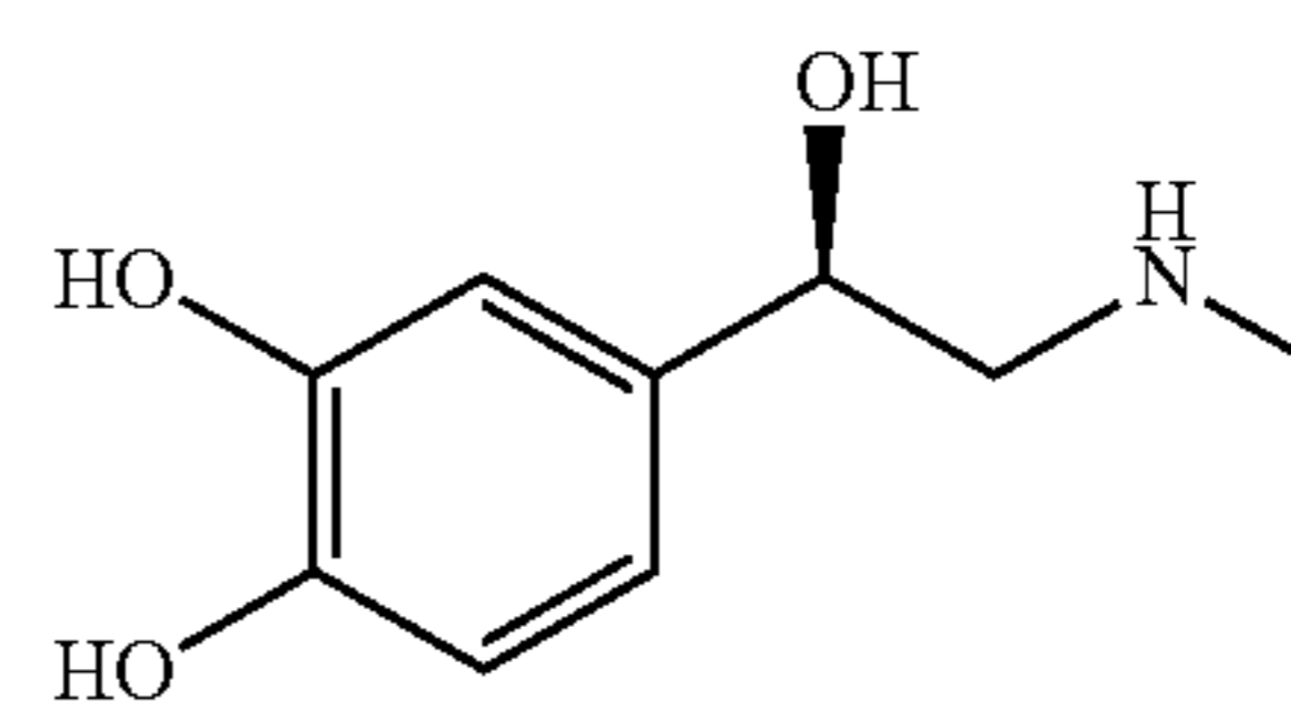
C_9H_{13}NO_3 MW 183.20 CAS Registry Number: 51-43-4
