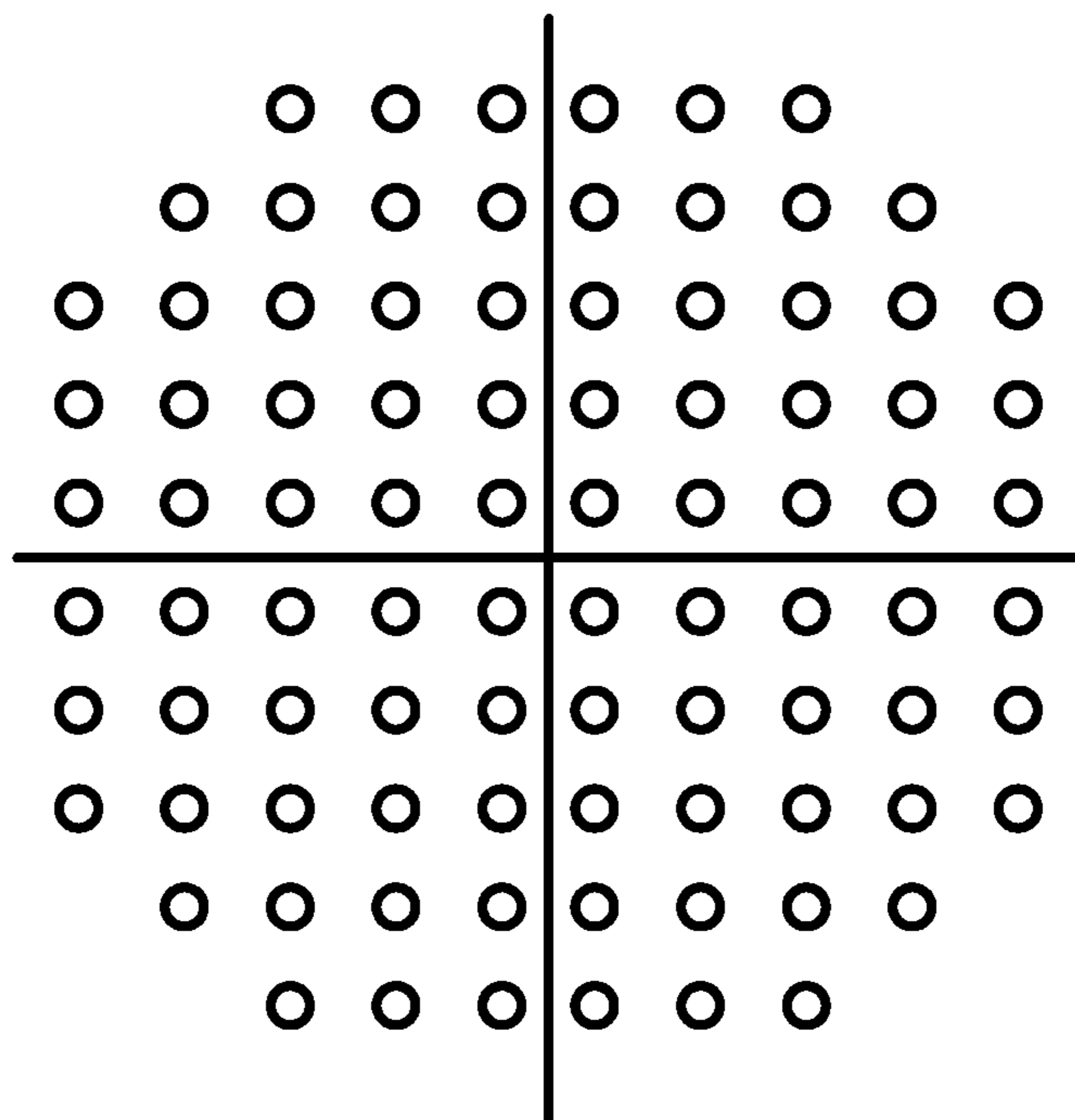
88QAM Modulation
