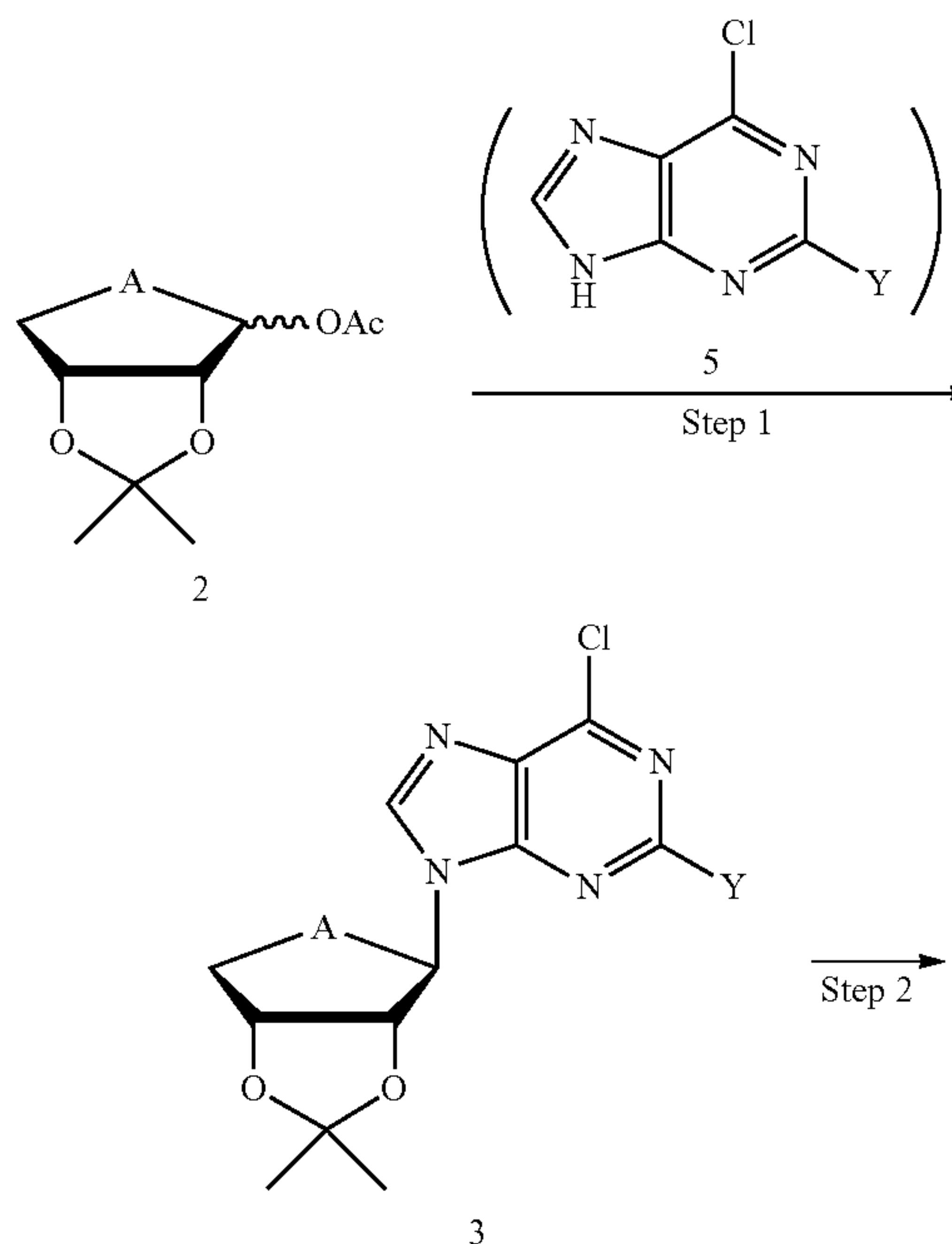
[Reaction Scheme 1]
