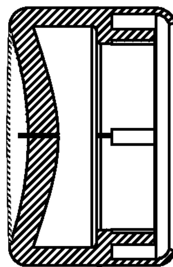
Section B-B
