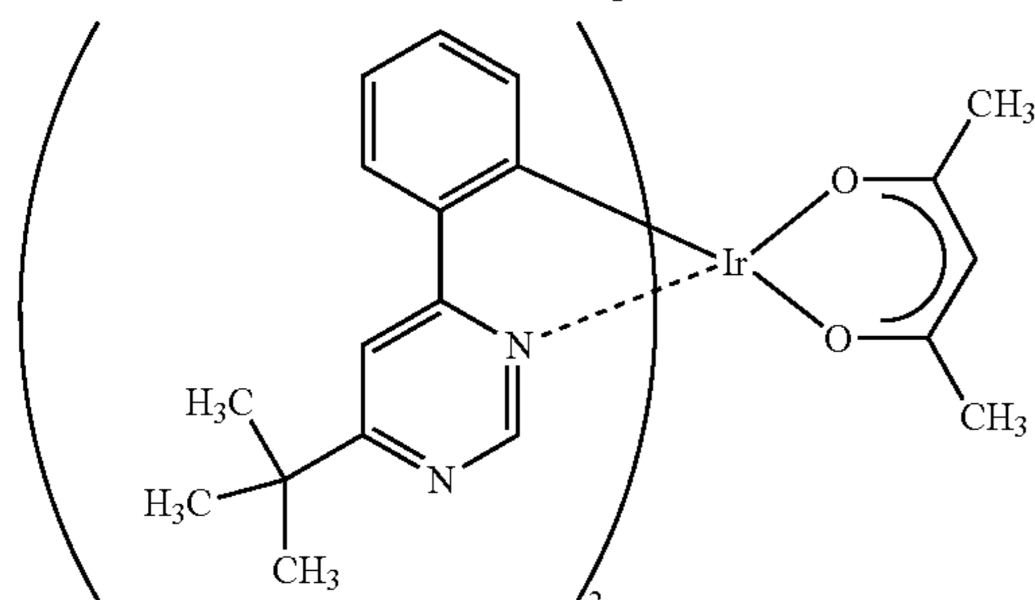
[\text{Ir}(\text{tBuppm})_2(\text{acac})]
