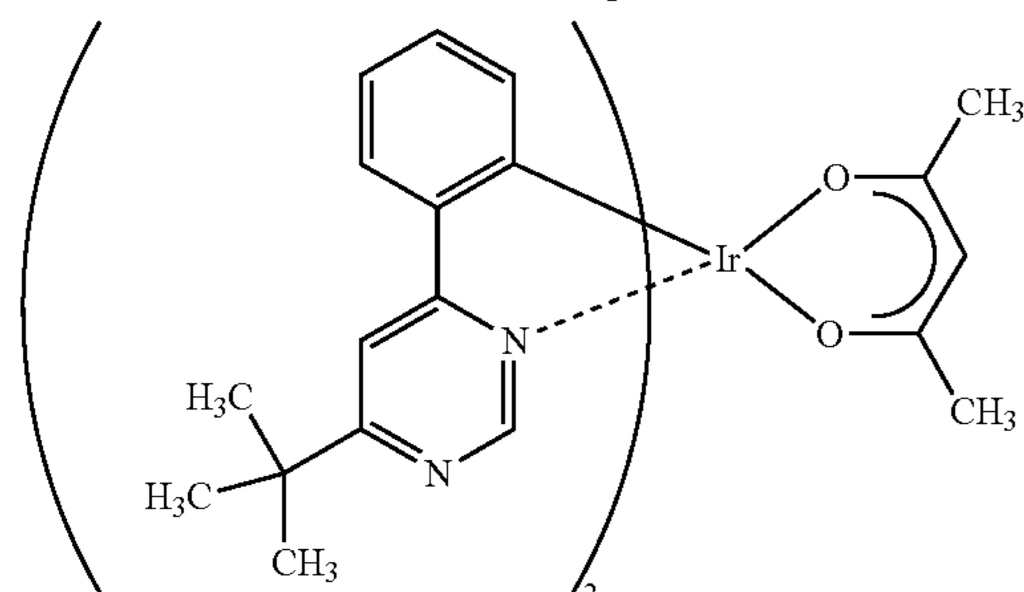
[Ir(tBuppm) 2 (acac)]
