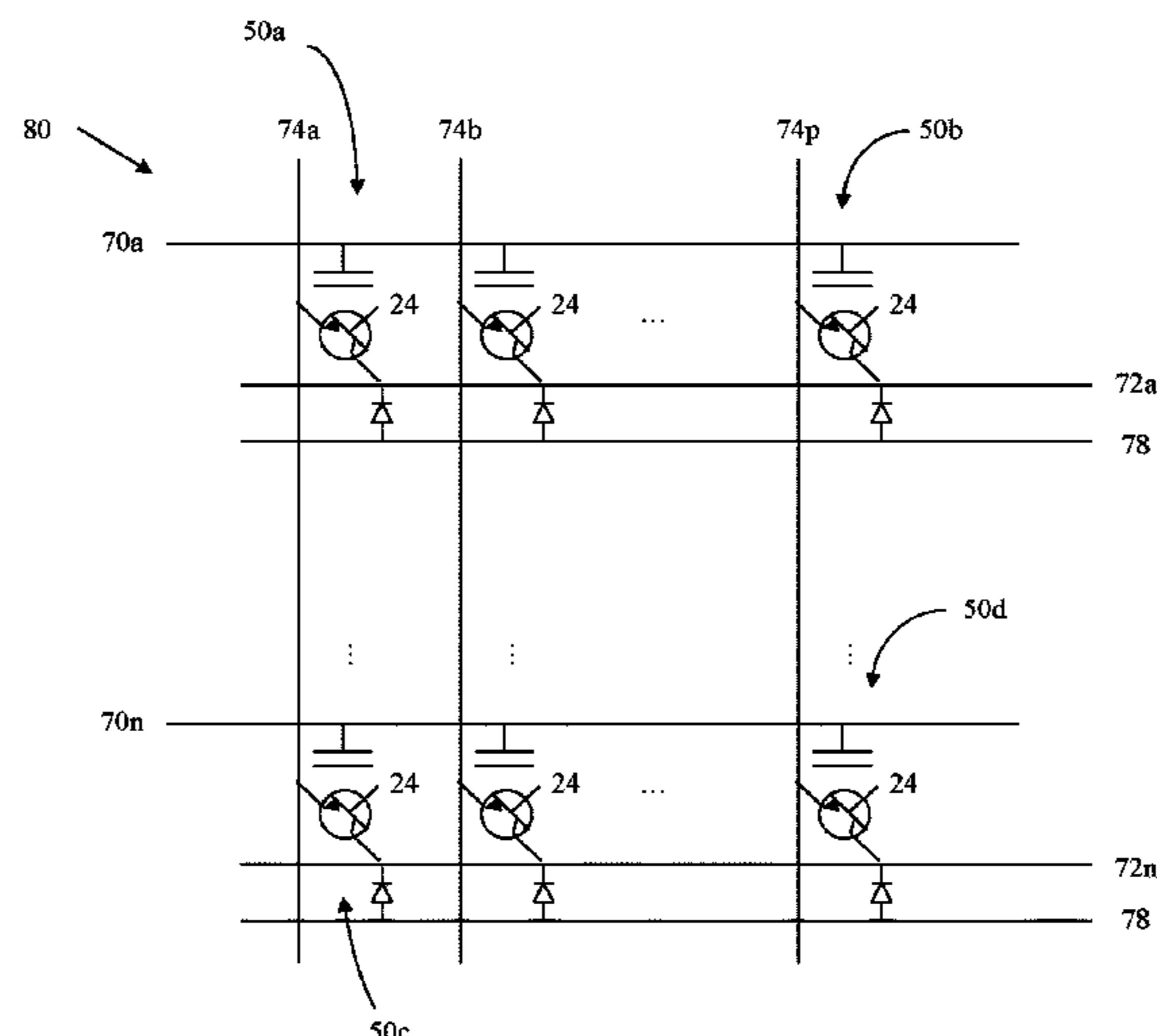
Exemplary Memory Array 80 with Representative Memory Cells 50a, 50b, 50c and 50d
