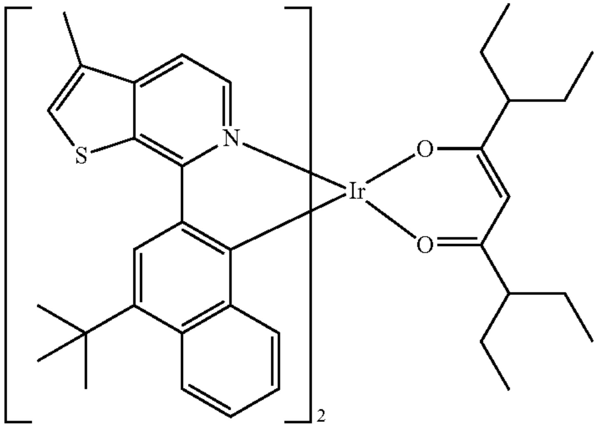
Comparative Compound 1
