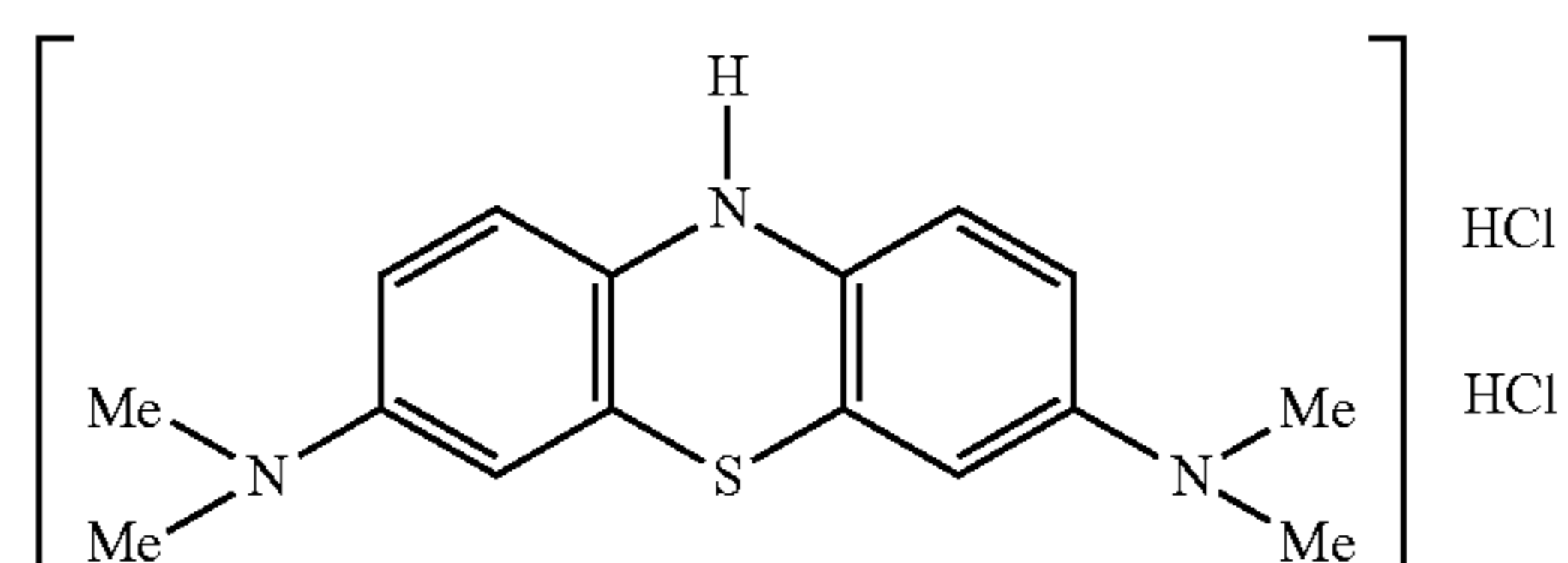
N,N,N',N'-tetramethyl-10H-phenothiazine-3,7-diaminium di(chloride), (LMT•2HCl)
