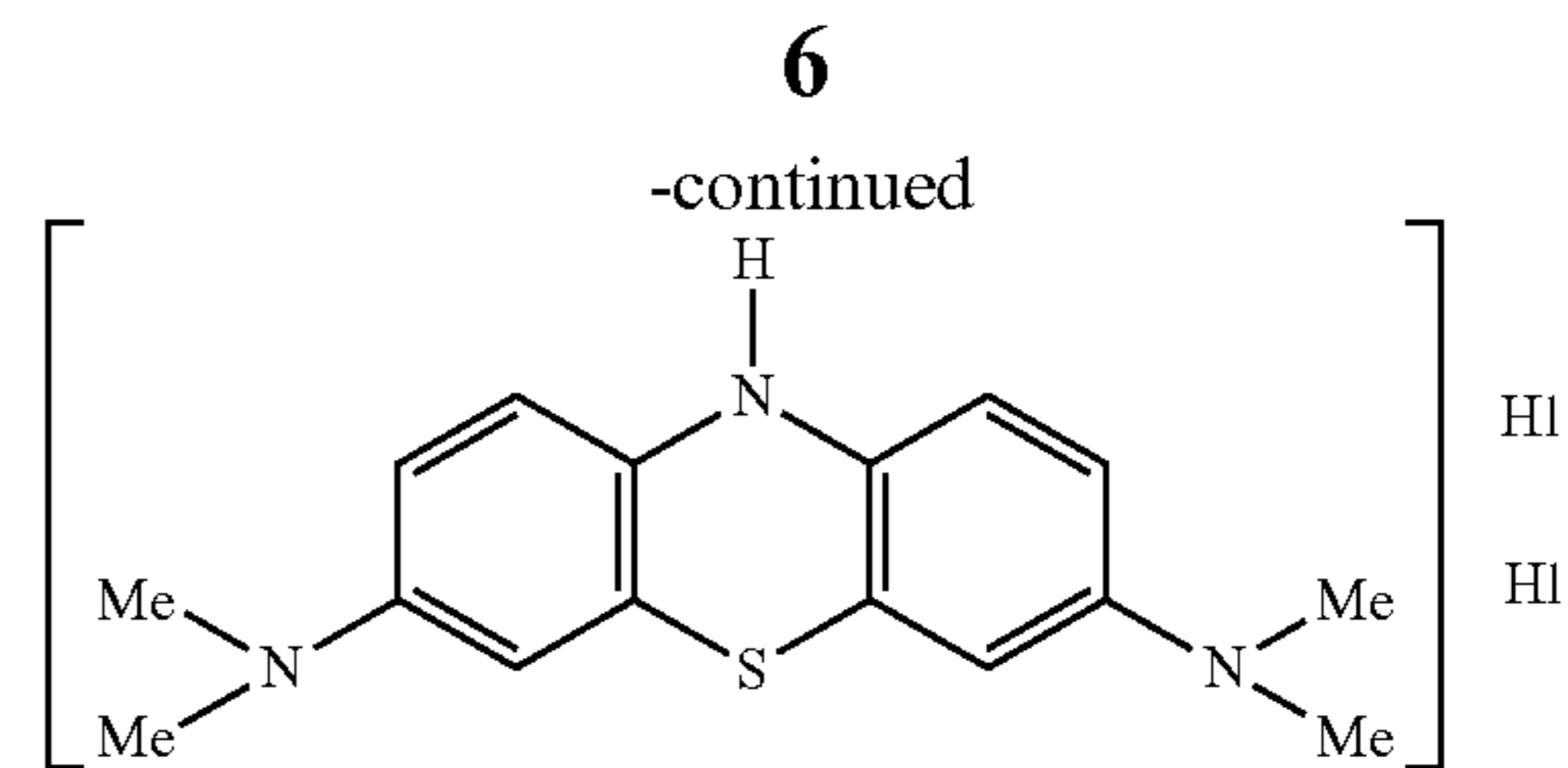
N,N,N',N'-tetramethyl-10H-phenothiazine-3,7-diaminium di(iodide), (LMT•2HI)
