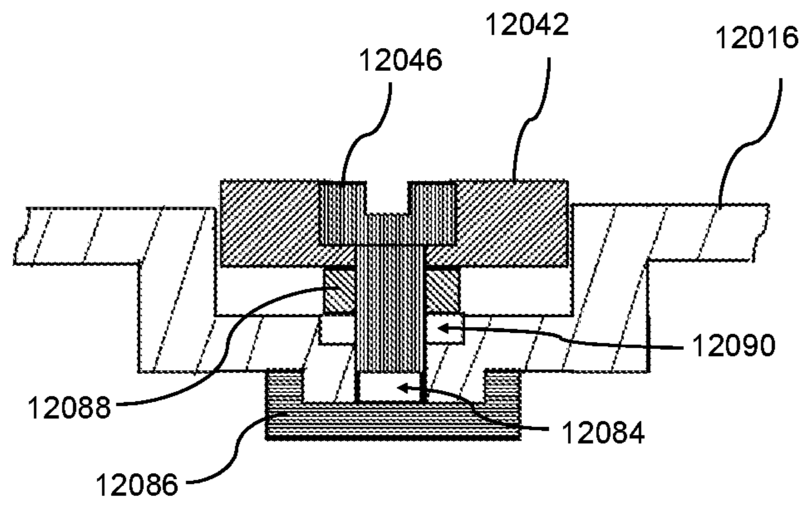
SECTION A
