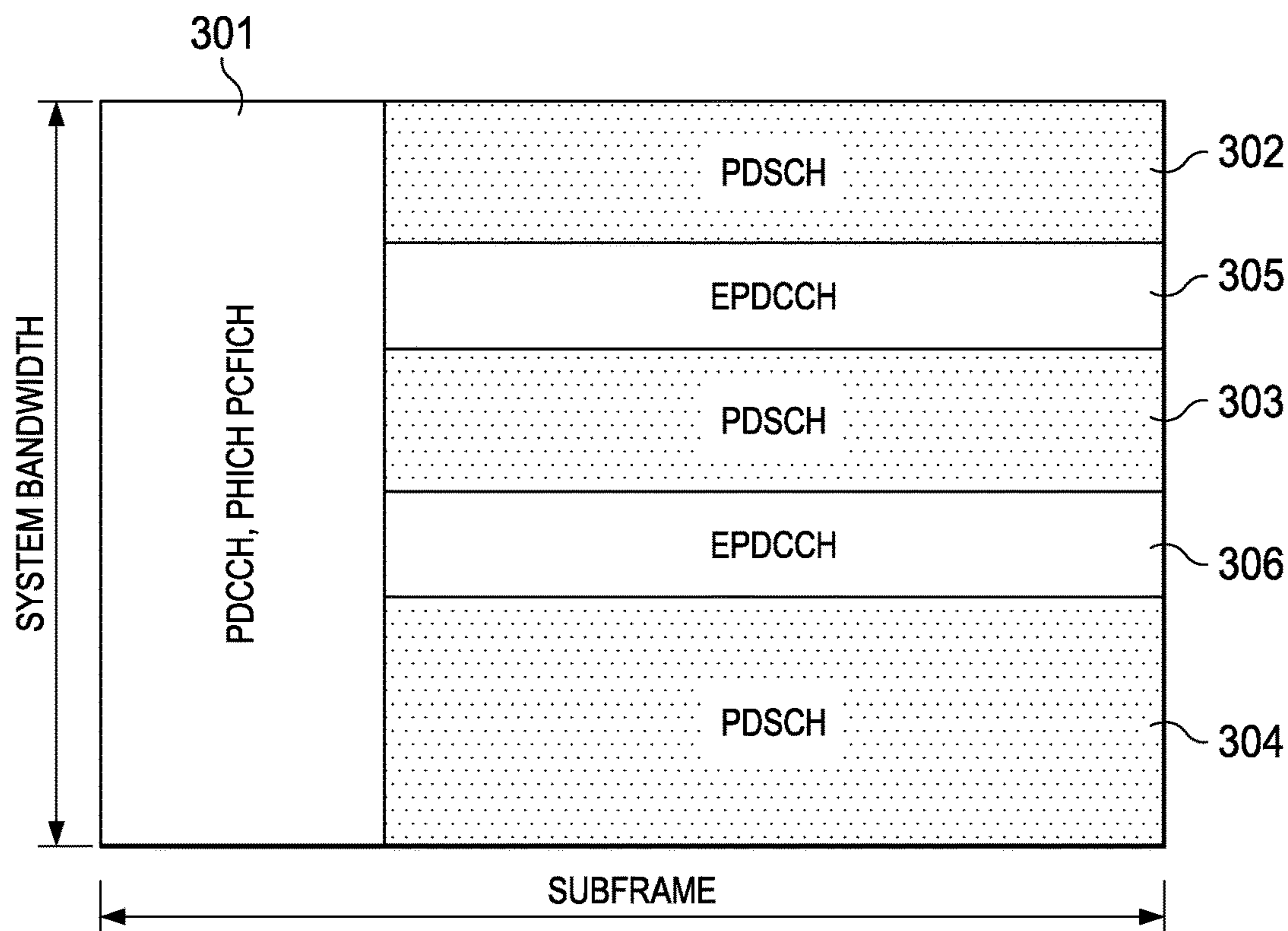
FIG. 3 (PRIOR ART)
