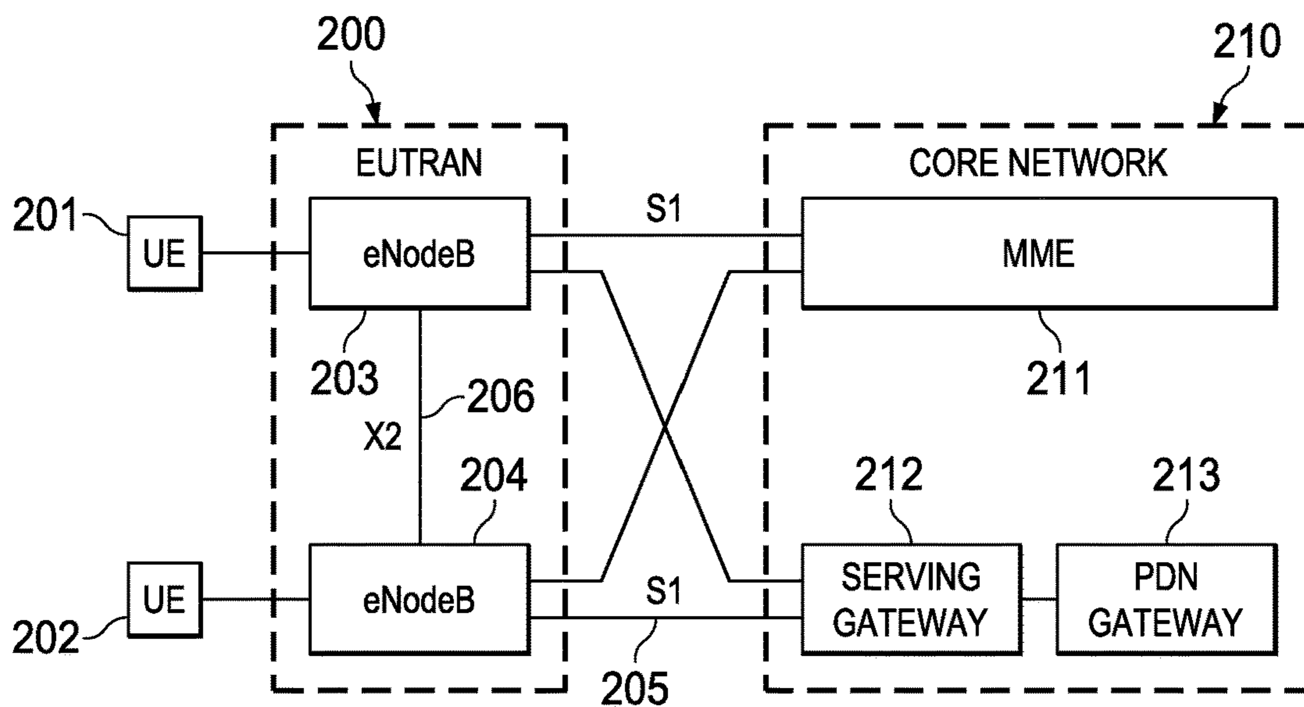
FIG. 2 (PRIOR ART)
