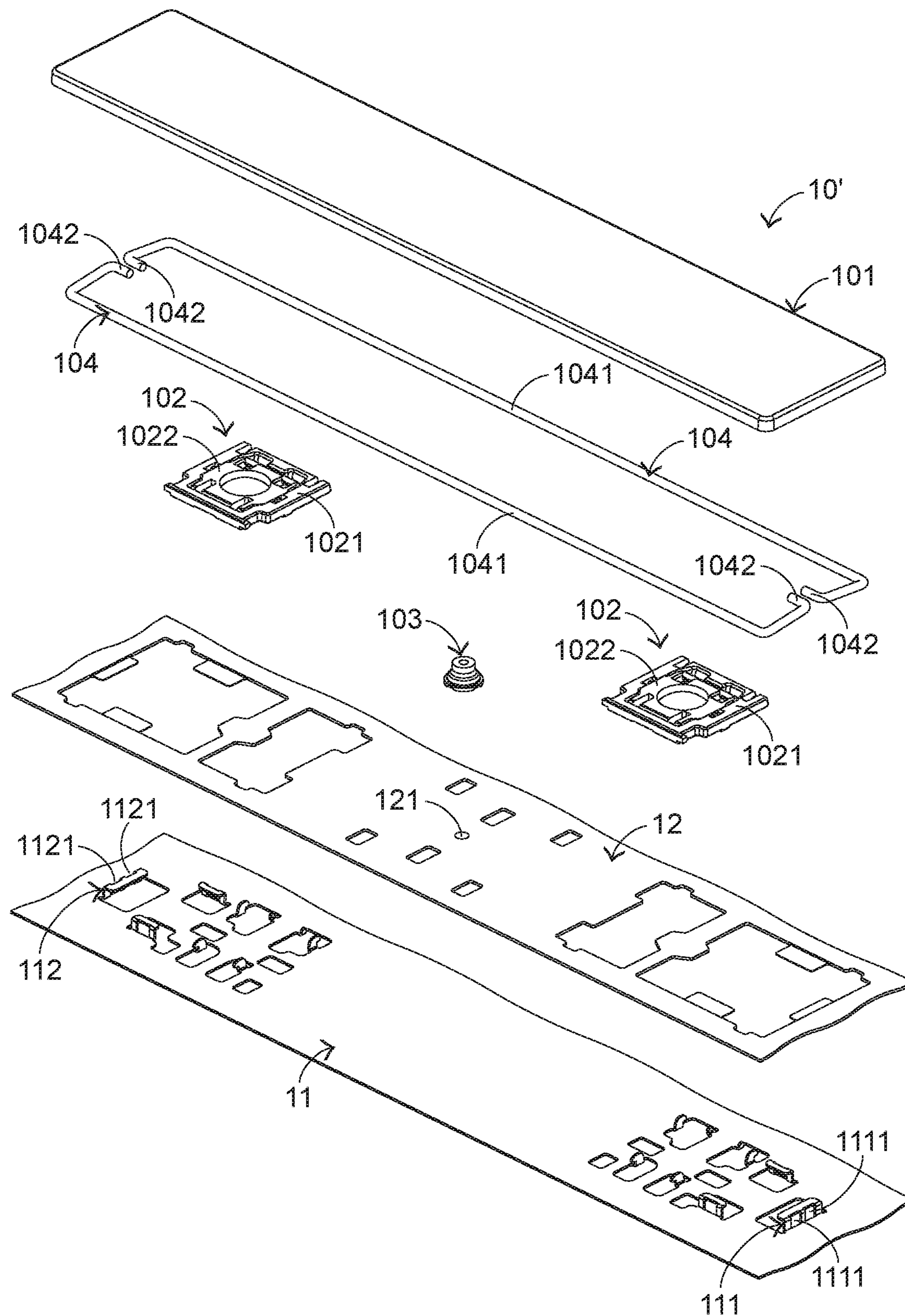
FIG.2 PRIOR ART
