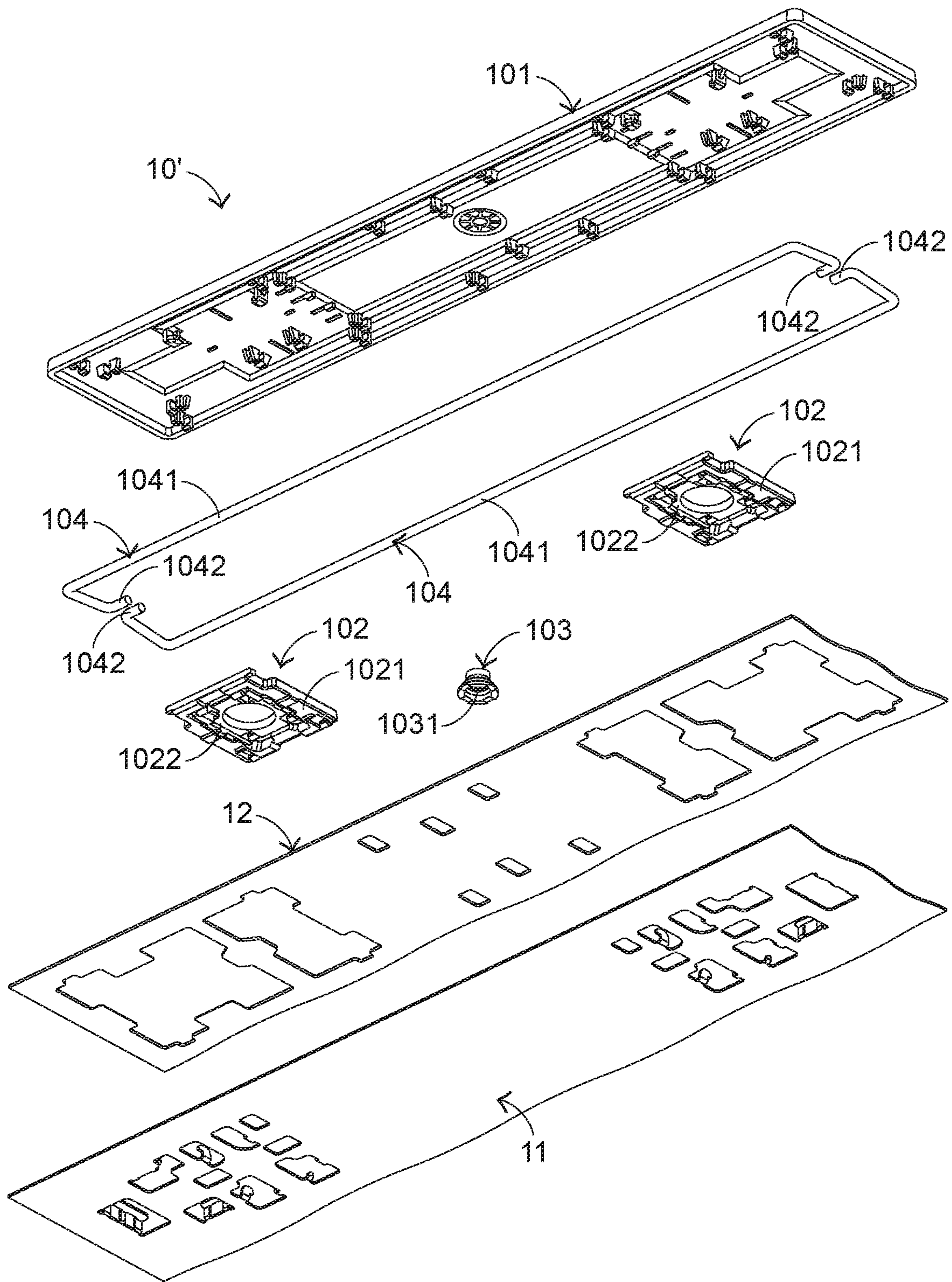
FIG. 3 PRIOR ART
