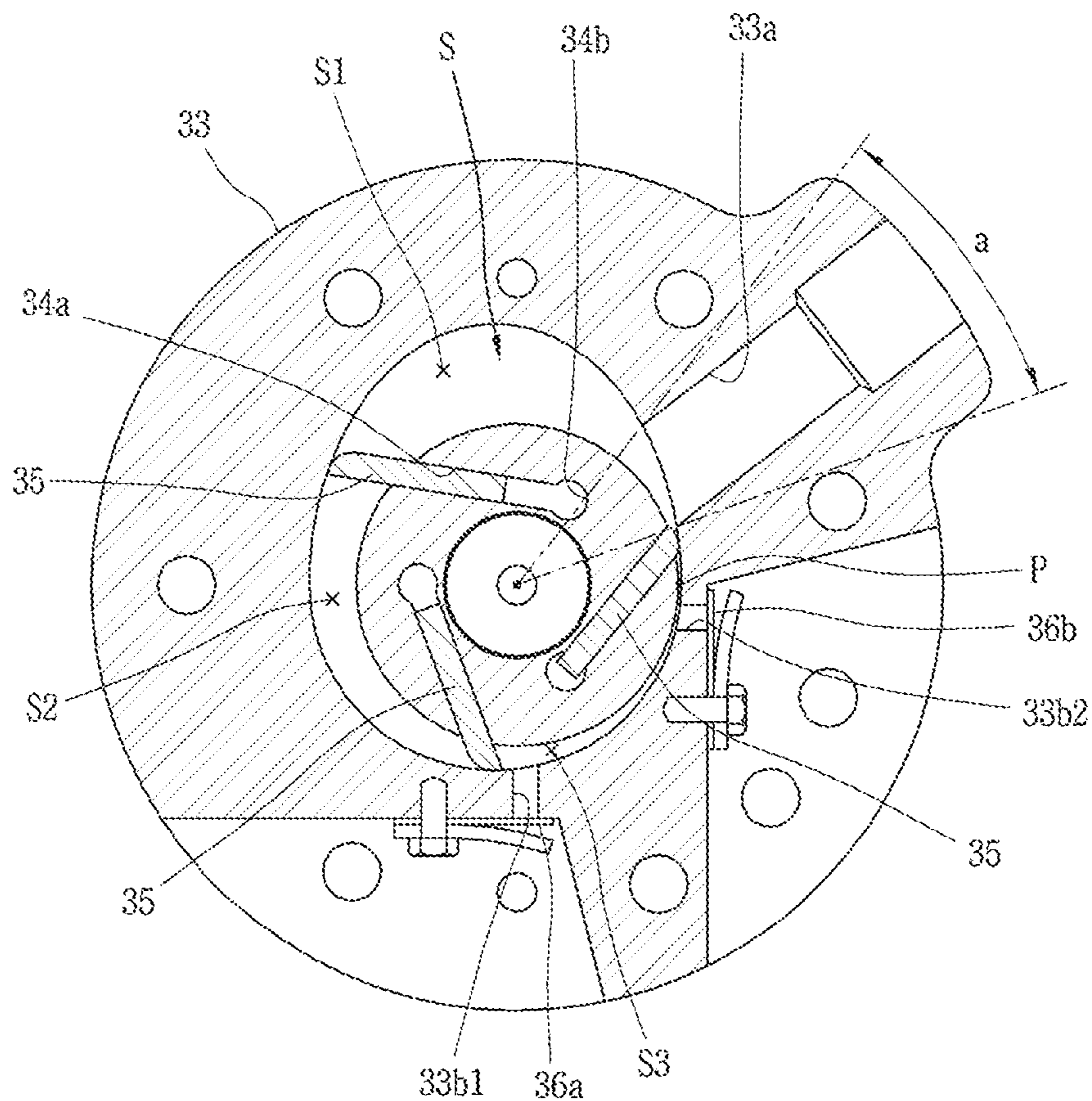
FIG. 2 CONVENTIONAL ART
