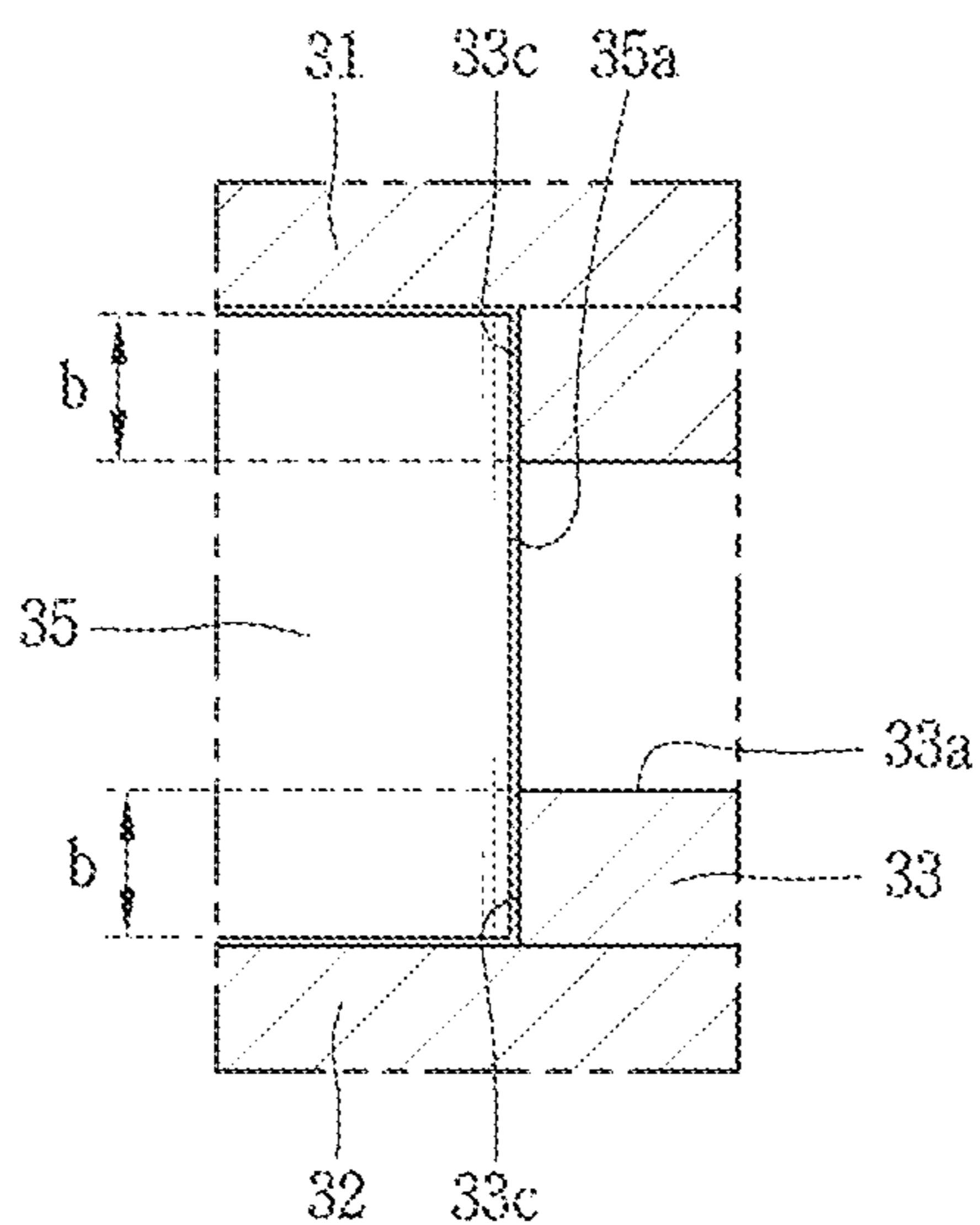
FIG. 3 CONVENTIONAL ART
