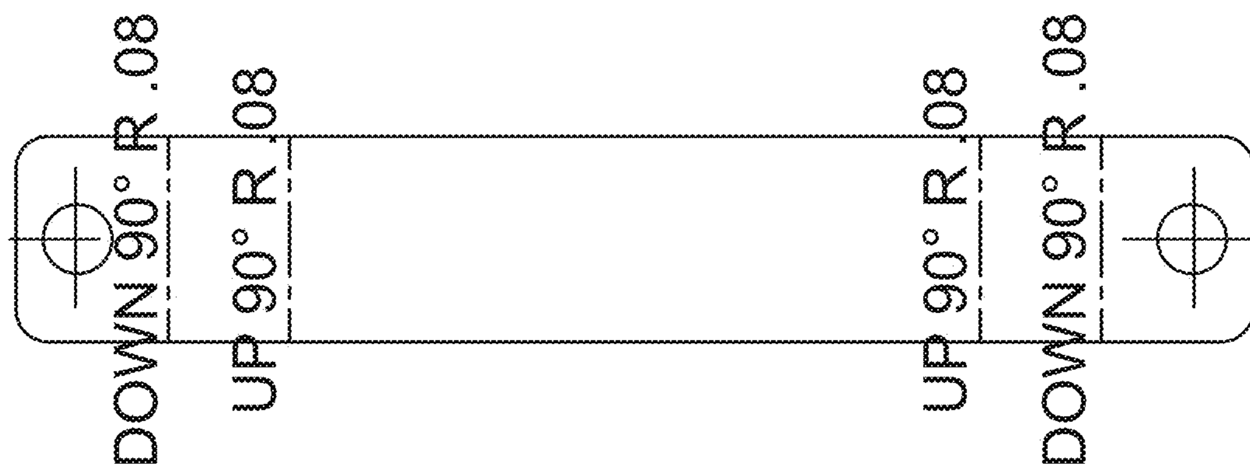
FLAT PATTERN
