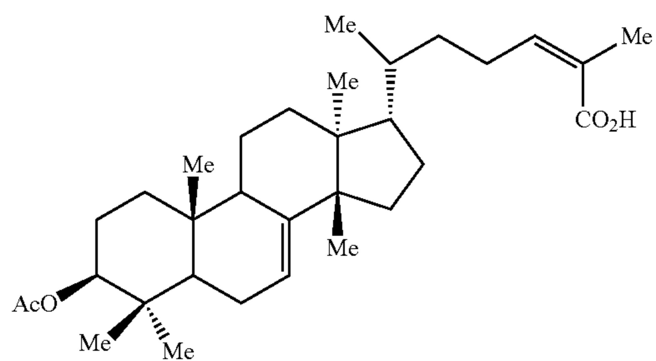
24-Z-3-O-acetyl-masticadienolic acid
