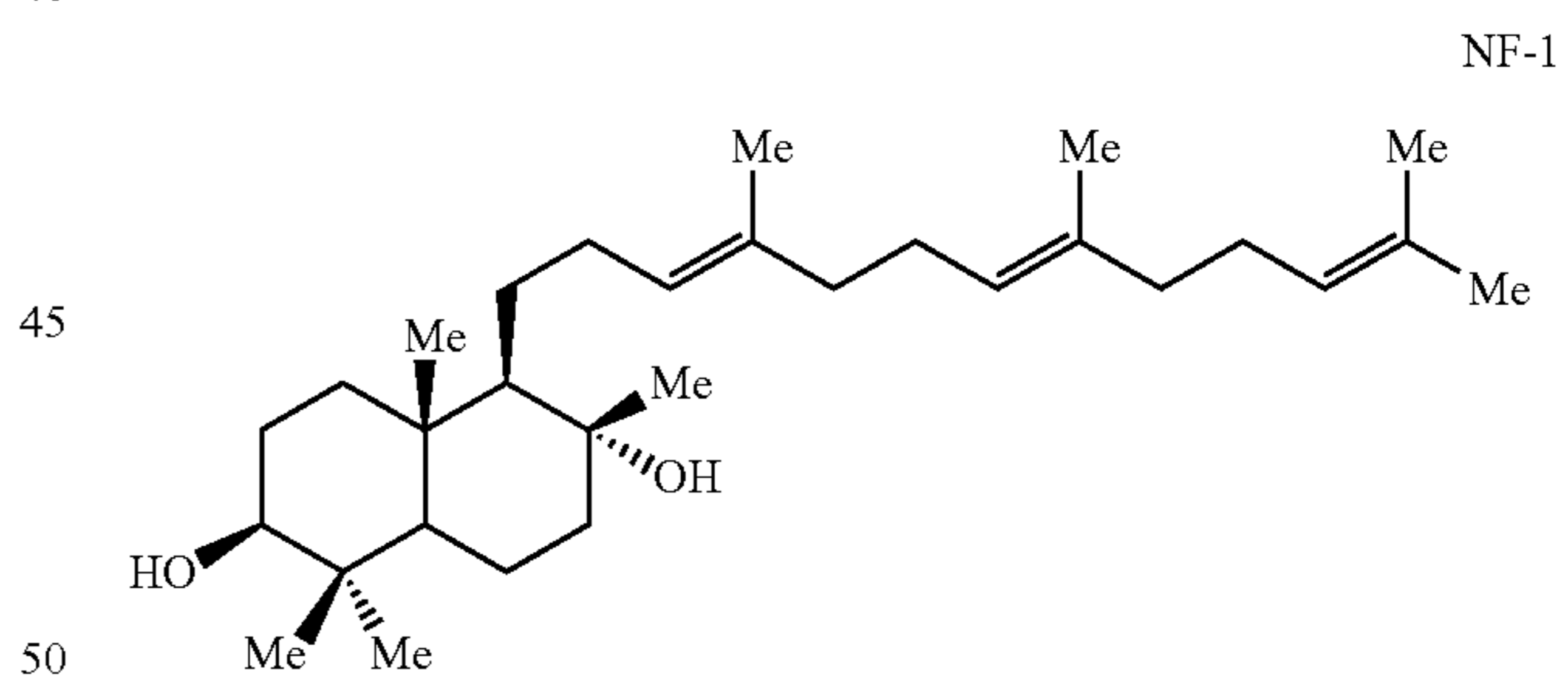
Scheme I
