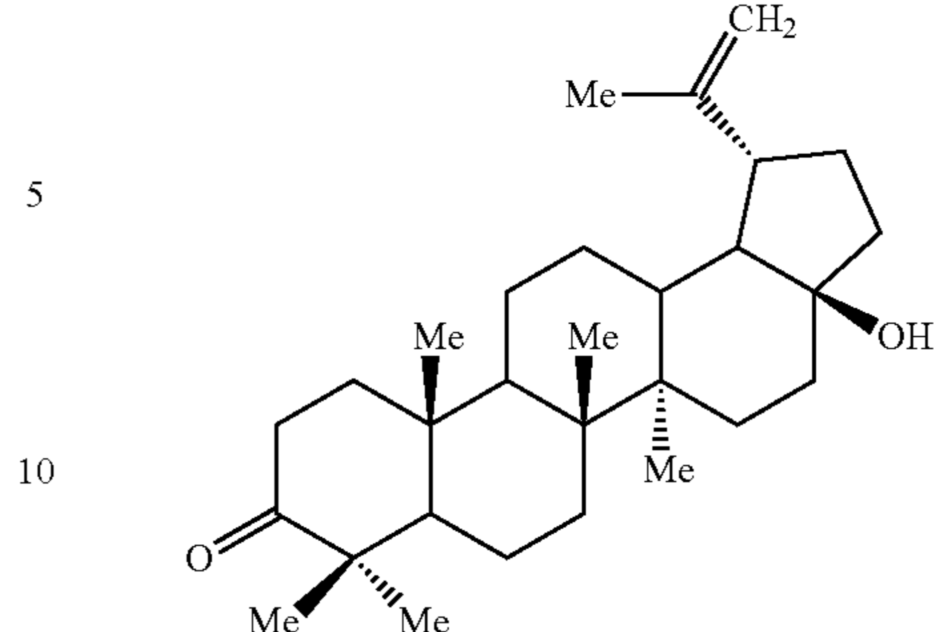
Name: 3-oxo-28nor-17-hydroxy-20(29)-ene (28-nor-17-hydroxybetulone)
