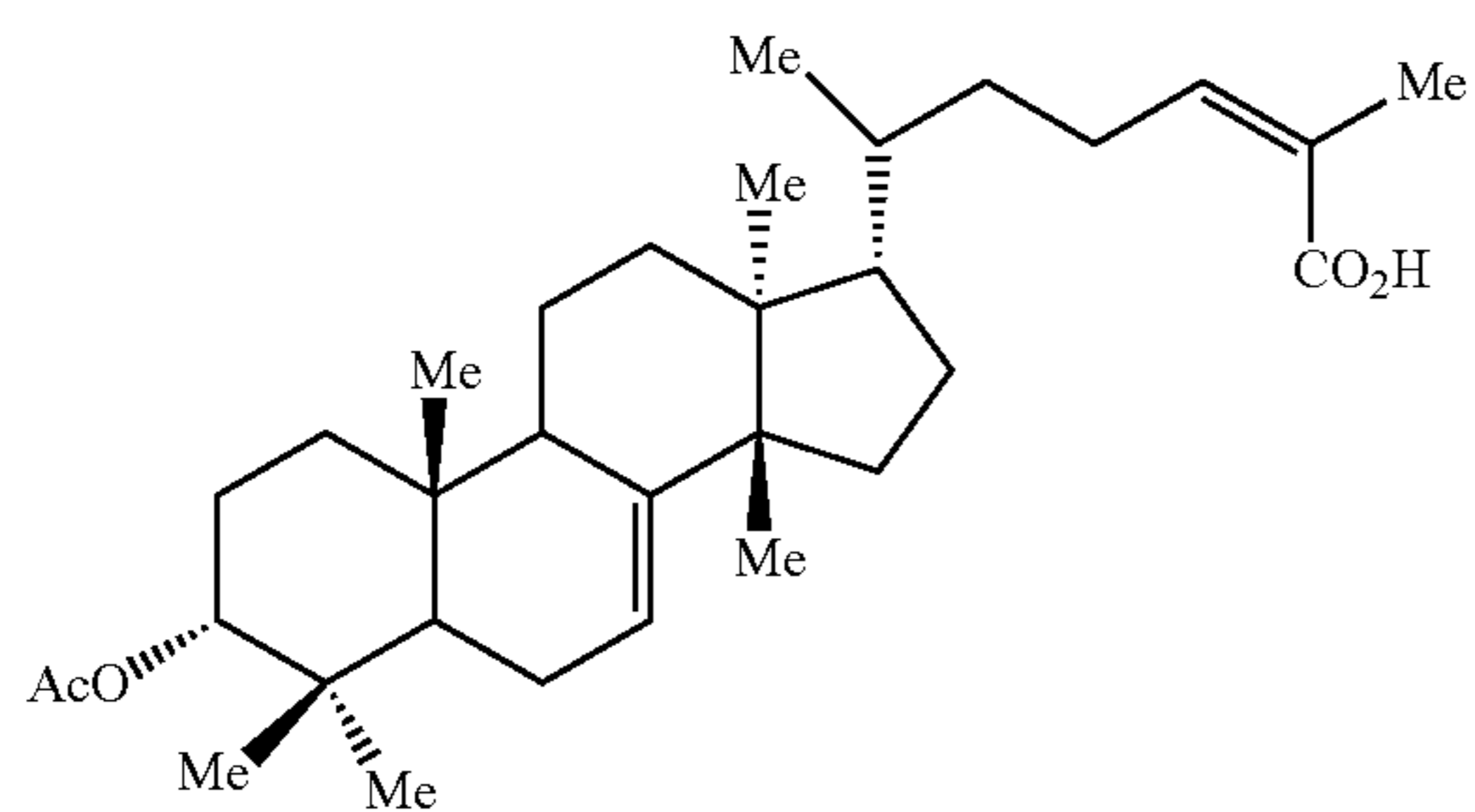
24-Z-3-O-acetyl-epimasticadienolic acid
