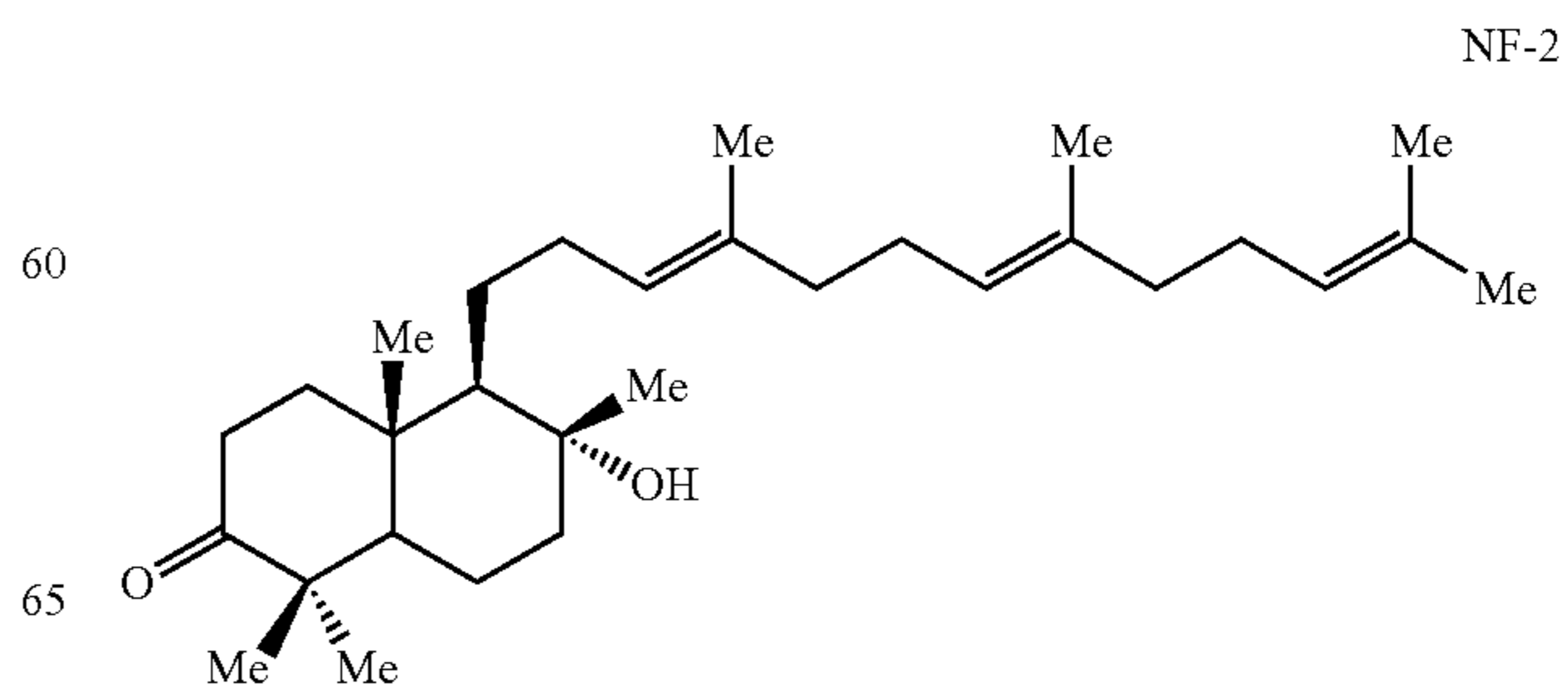
Scheme II
