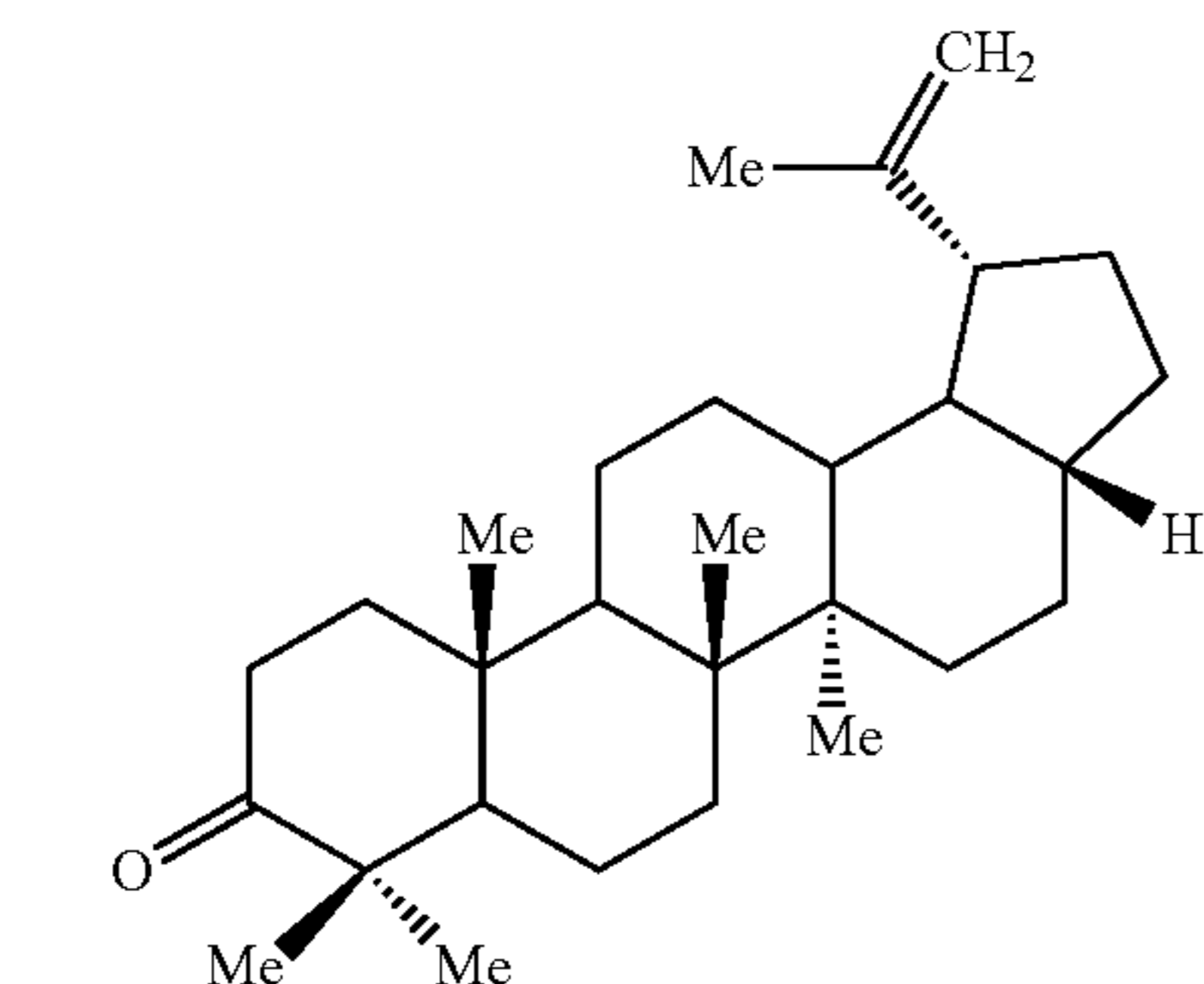
Name: 3-oxo-28-norlup-20(29)-ene (28-nor-betulone)
