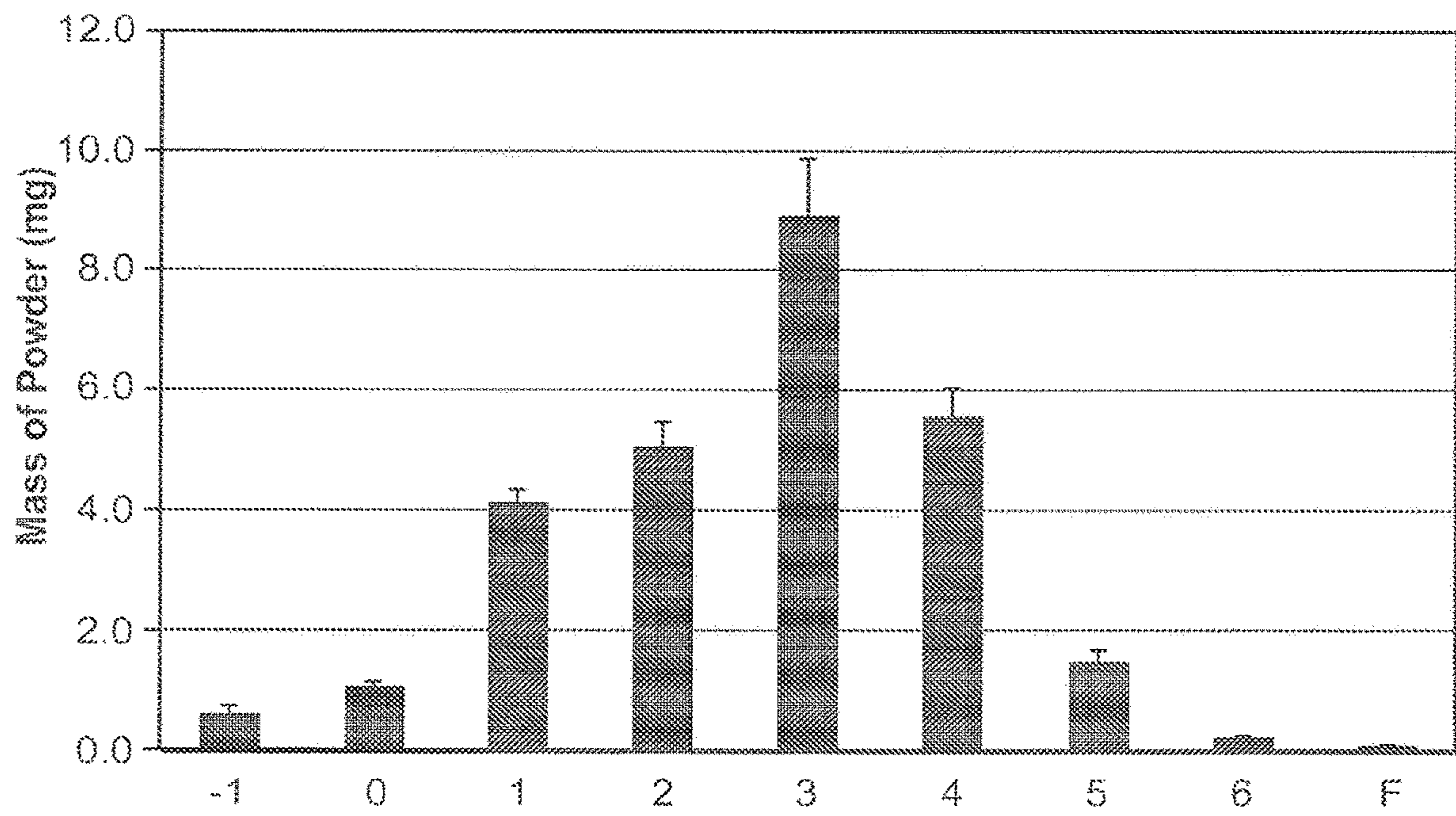
Gravimetric ACI8 at 60LPM (n=3). Formulation V
