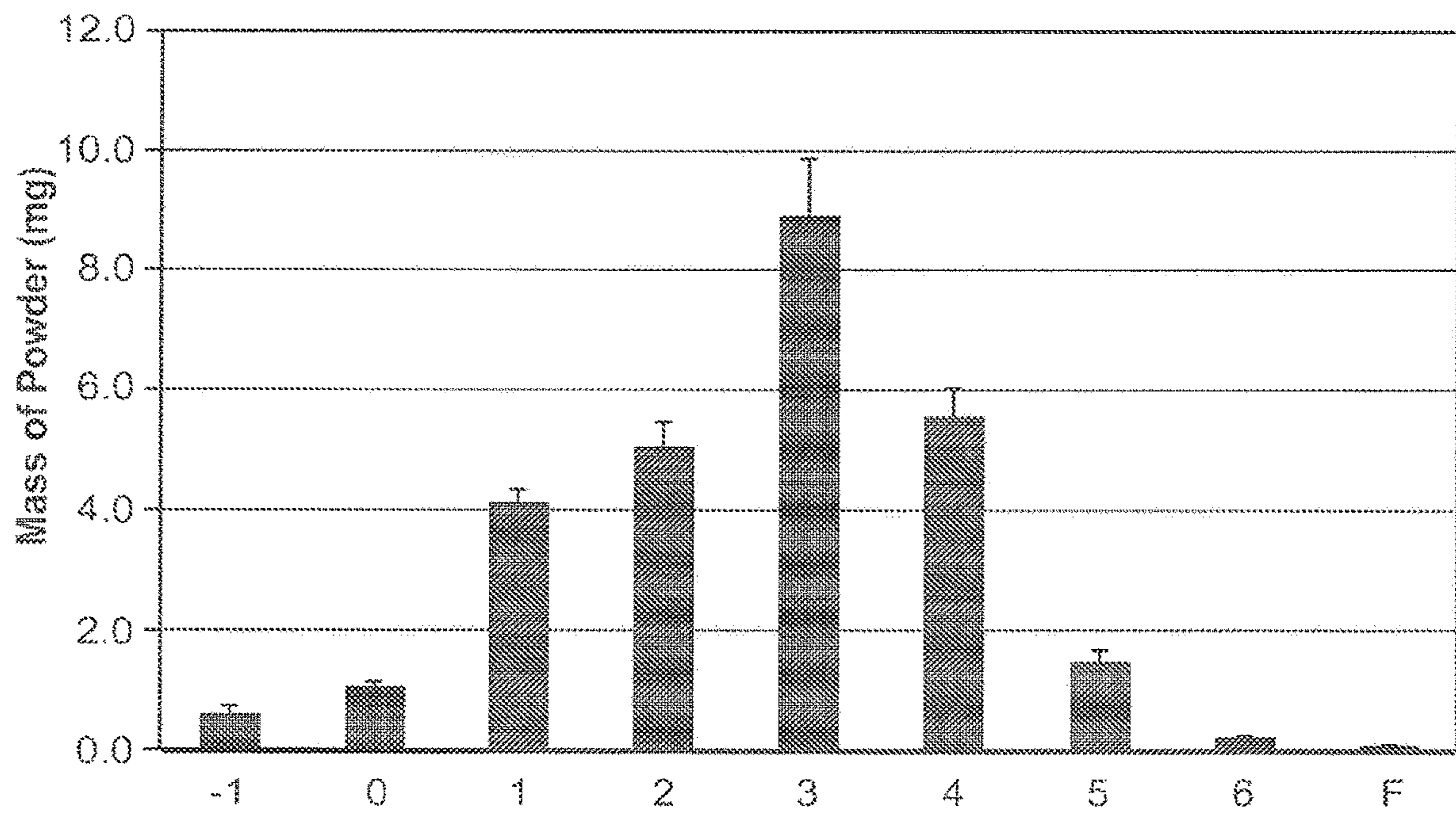
Gravimetric ACI8 at 60LPM (n=3). Formulation V
