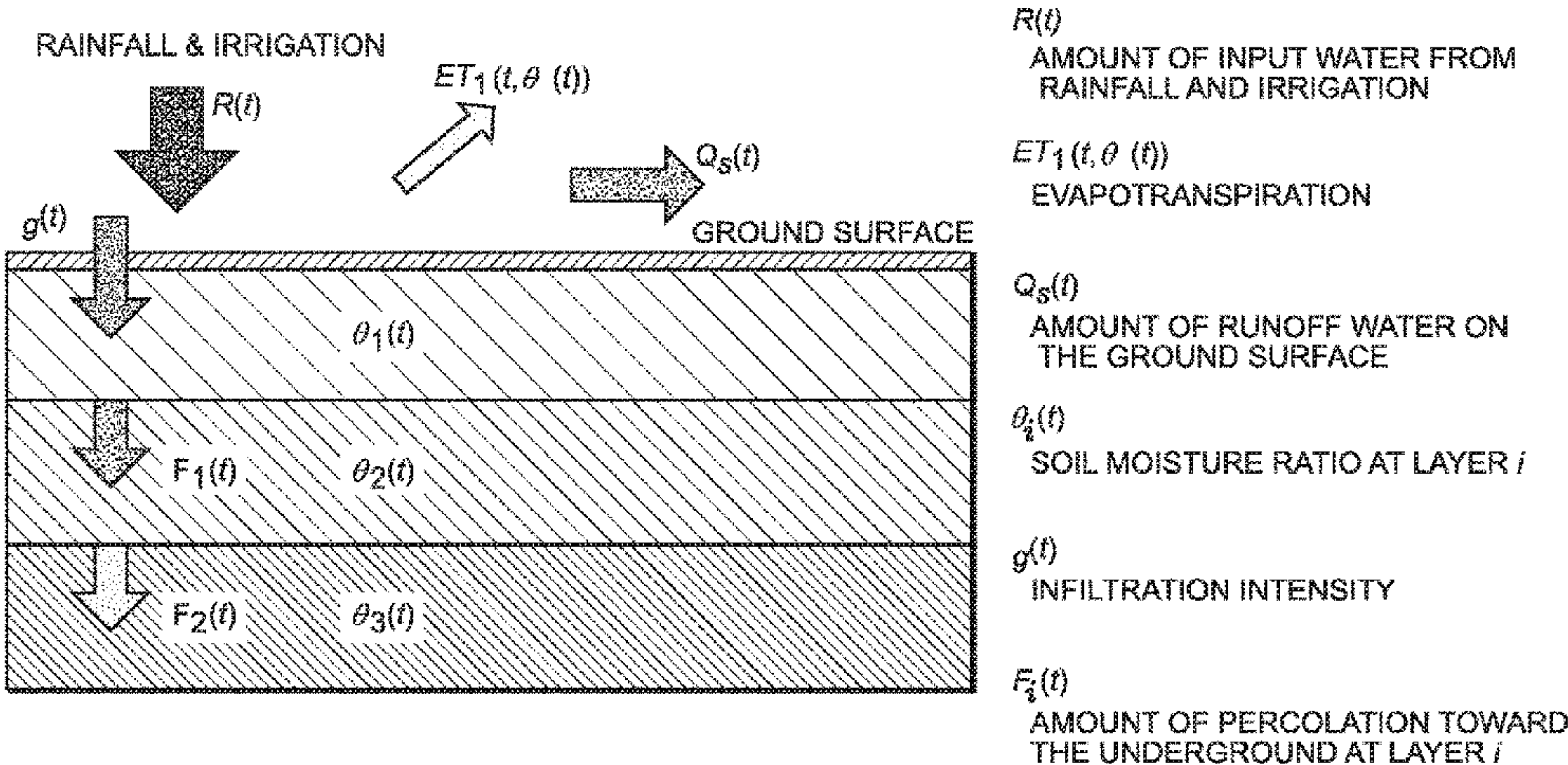
SIMULATION OF WATER PERCOLATION IN MULTIPLE SOIL LAYERS
