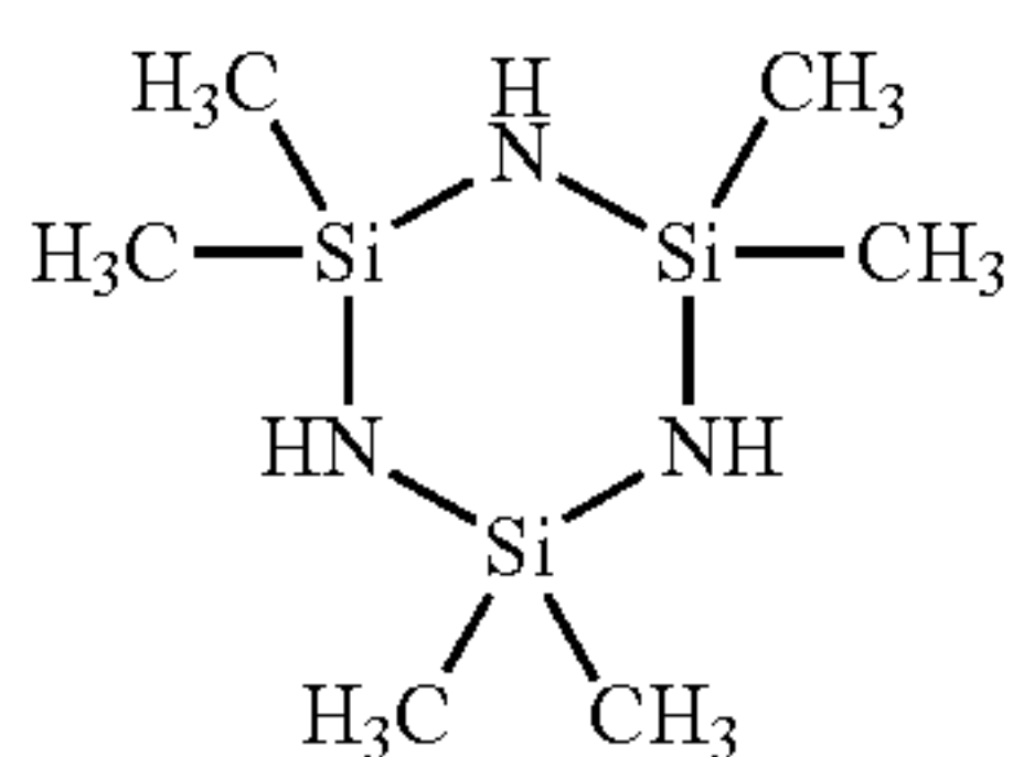
2,2,4,4,6,6-Hexamethyl-1,3,5,2,4,6-triazatrisilazane
