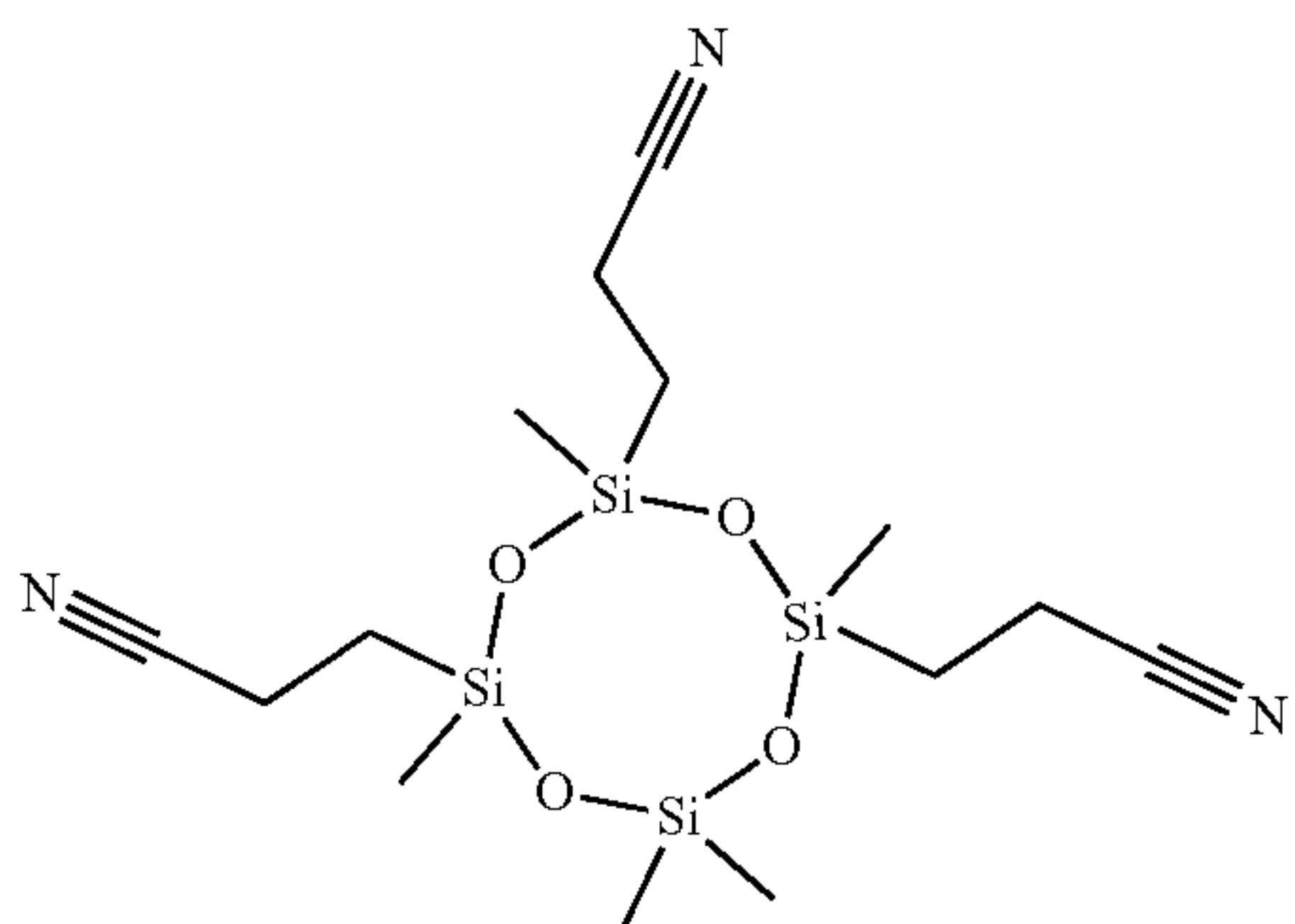
2,2,4,6,8-pentamethyl-4,6,8-tri(2-cyanoethyl)-[1,3,5,7,2,4,6,8]cyclotetrasiloxane
