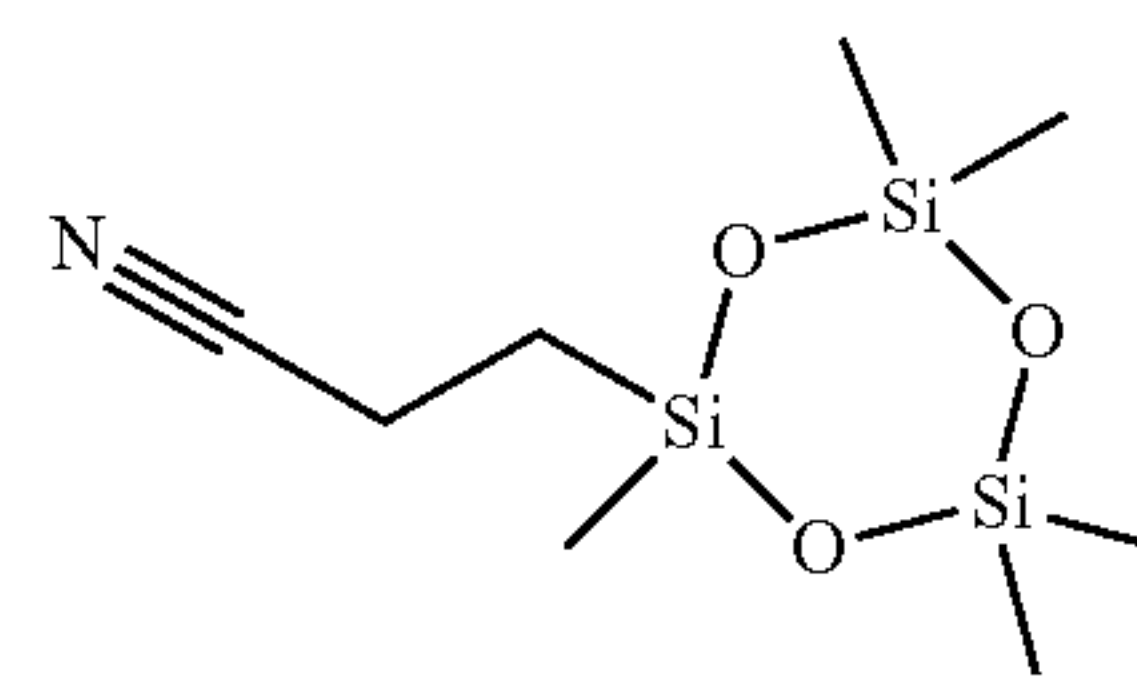
2,2,4,4,6-pentamethyl-6-(2-cyanoethyl)-[1,3,5,2,4,6]cyclotrisiloxane
