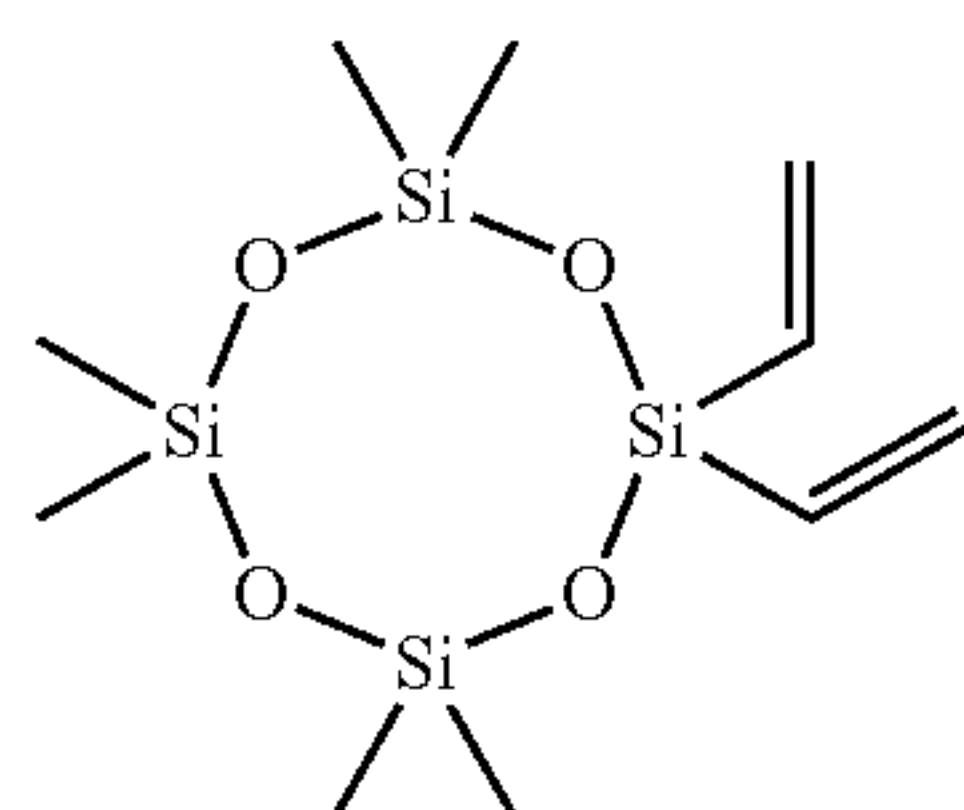
Cyclotetrasiloxane, diethenylhexamethyl-
