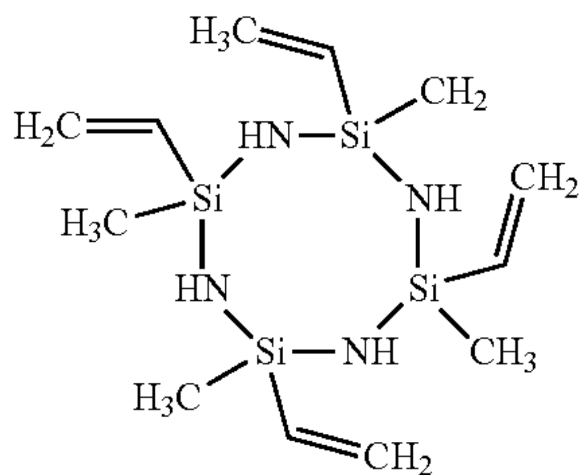
2,4,6,8-Tetramethyl-2,4,6,8-tetravinylcyclotetrasilazane
