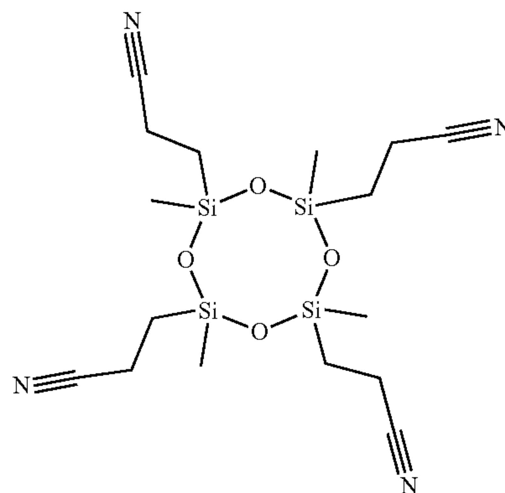
2,4,6,8-tetramethyl-2,4,6,8-tetra(2-cyanoethyl)-[1,3,5,7,2,4,6,8]cyclotetrasiloxane
