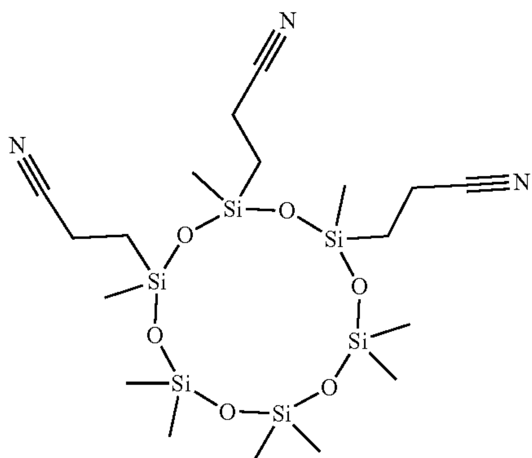
2,2,4,4,6,6,8,8,10,12-nonamethyl-8,10,12-tri(2-cyanoethyl)-[1,3,5,7,9,11,2,4,6,8,10,12]cyclohexasiloxane
