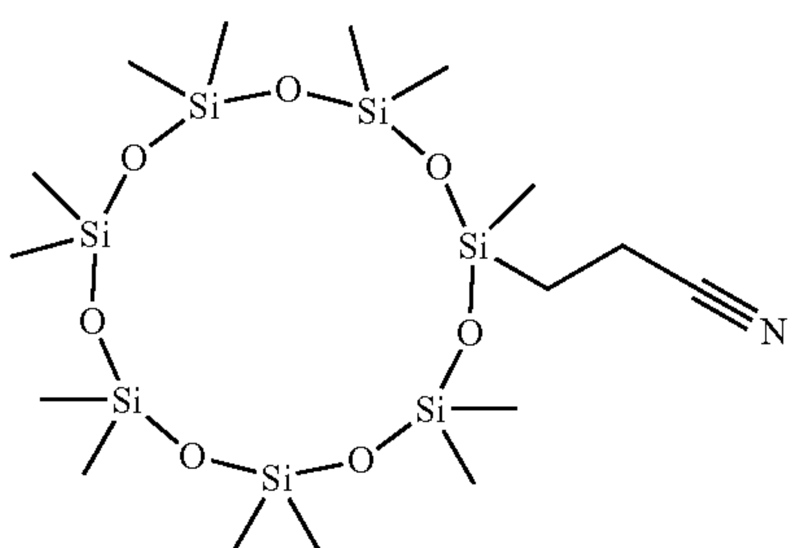
2,2,4,4,6,6,8,8,10,10,12,12,14-tridecamethyl-12-(2-cyanoethyl)-[1,3,5,7,9,11,13,2,4,6,8,10,12,14]cycloheptasiloxane
