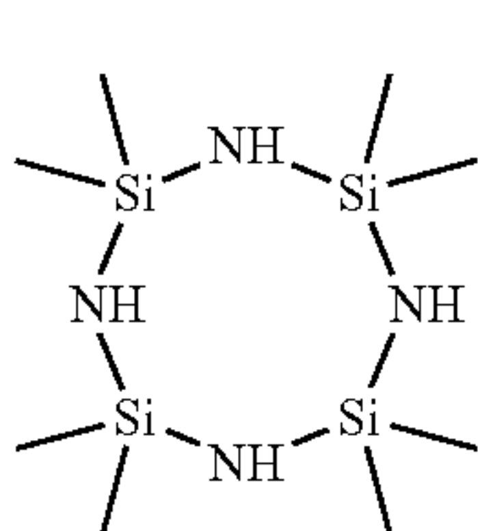
Octamethylcyclotetrasilazane
