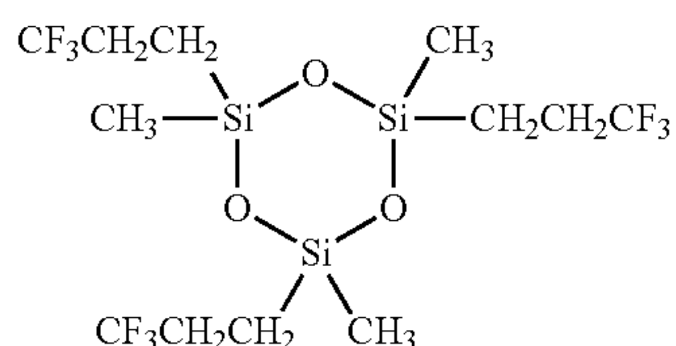
1,3,5-Tris[(3,3,3-trifluoropropyl)methyl]cyclotrisiloxane
