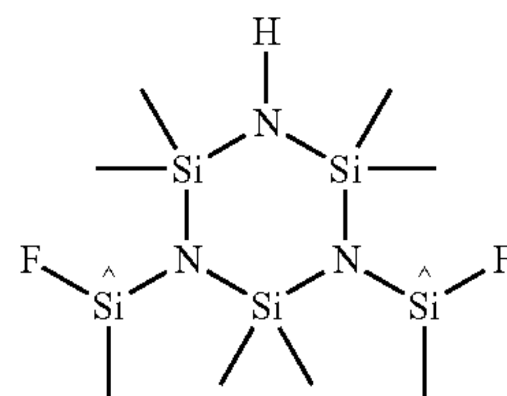
1,3-bis(methylfluorosilyl)-2,2,4,4,6,6-hexamethyl-cyclotrisilazane
