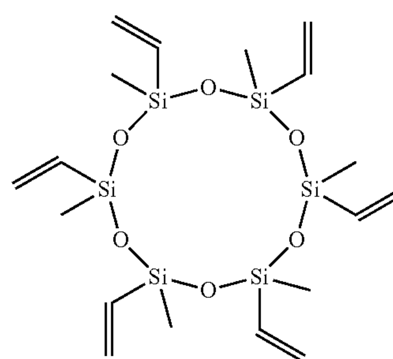
1,3,5,7,9,11-Hexamethyl-1,3,5,7,9,11-hexavinylcyclohexasiloxane
