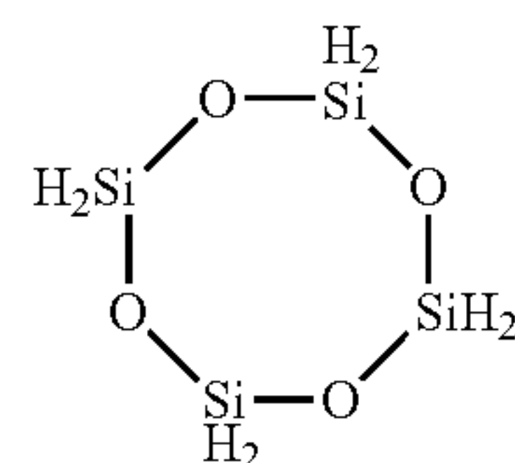
Cyclotetrasiloxane
