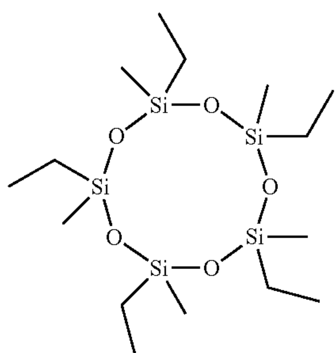
2,4,6,8,10-Pentaethyl-2,4,6,8,10-pentamethylcyclopentasiloxane
