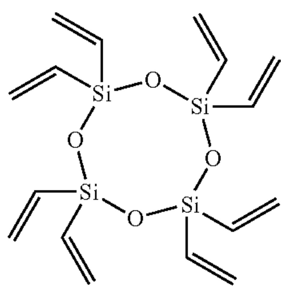
Cyclotetrasiloxane, octaethenyl-
