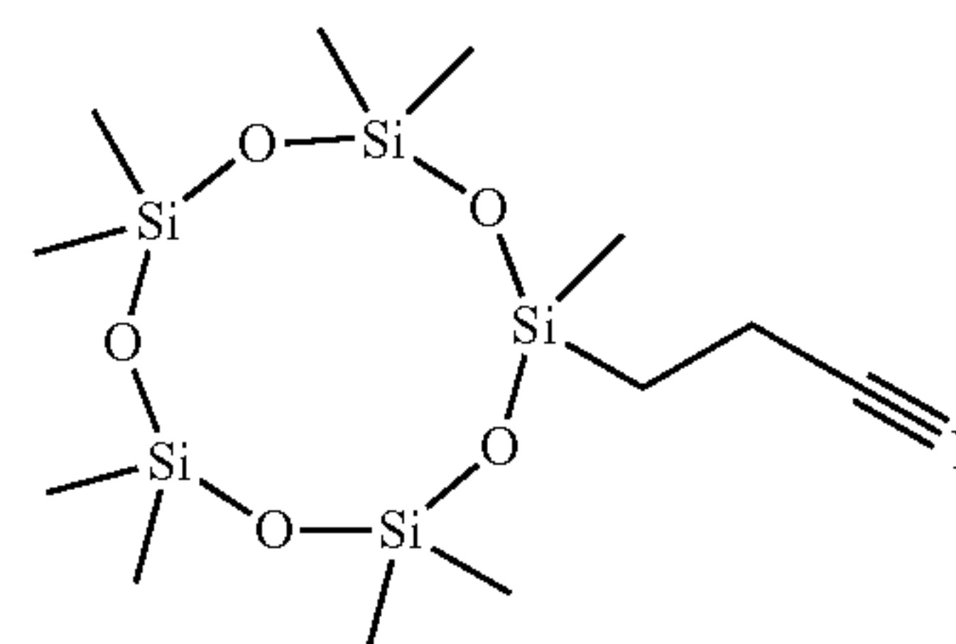
2,2,4,4,6,6,8,8,10-nonamethyl-10-(2-cyanoethyl)-[1,3,5,7,9,2,4,6,8,10]cyclopentasiloxane
