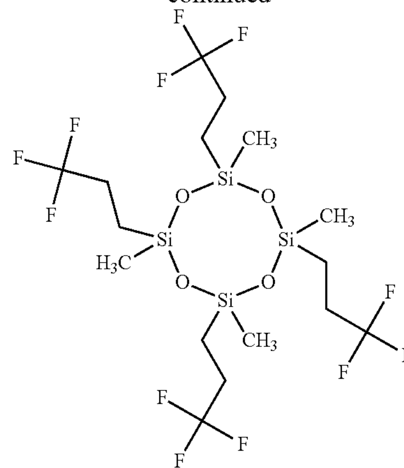
2,4,6,8-Tetramethyl-2,4,6,8-tetra(3,3,3-trifluoropropyl)cyclotriloxane
