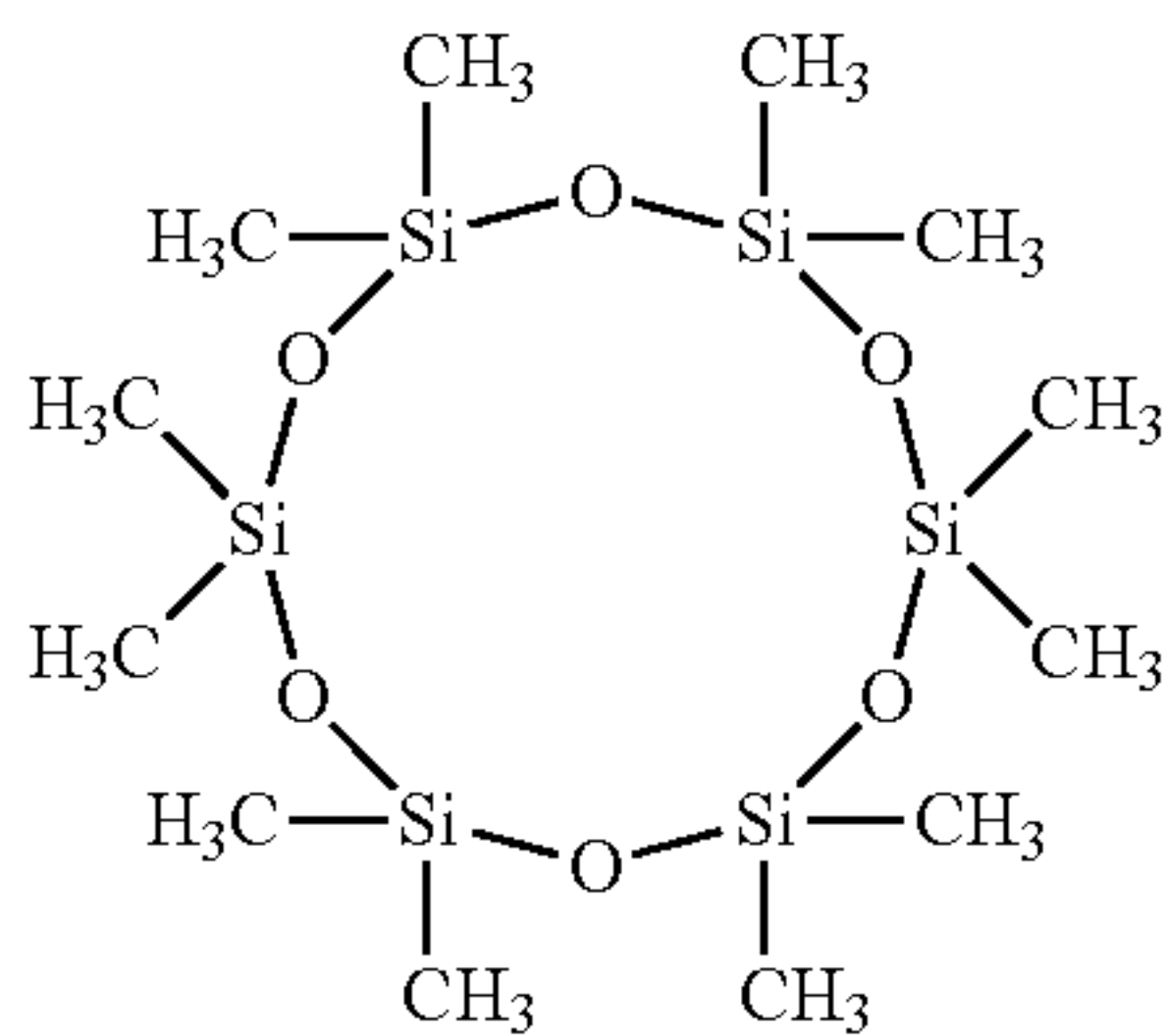
cyclohexasiloxane, dodecamethyl-
