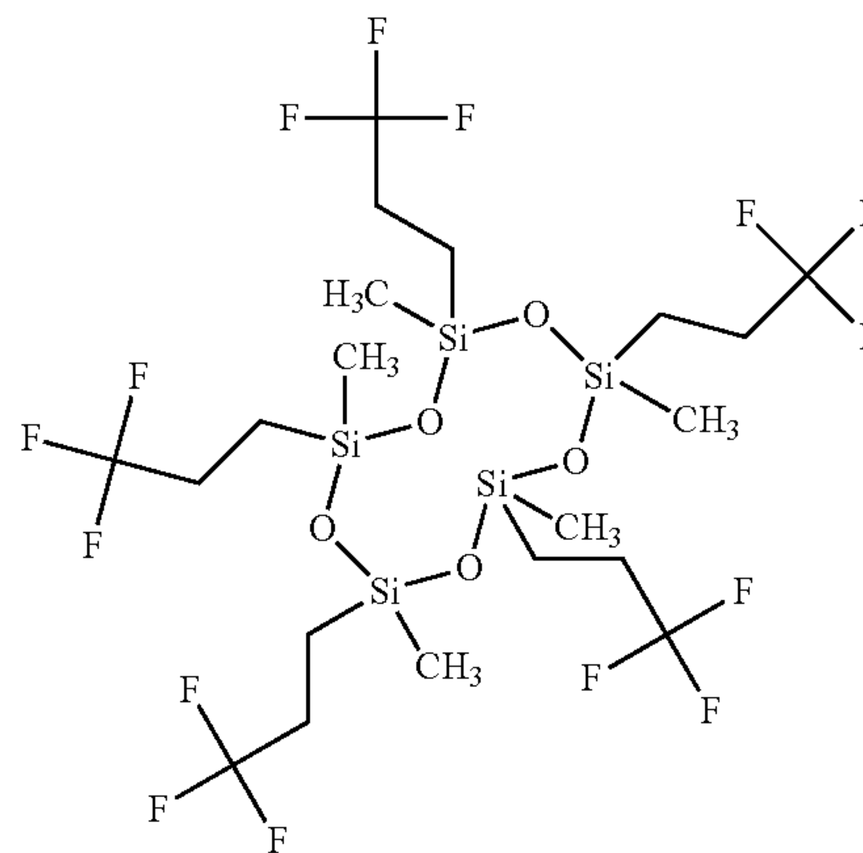
cyclopentasiloxane, 2,4,6,8,10-pentamethyl-2,4,6,8,10-pentakis(3,3,3-trifluoropropyl)-
