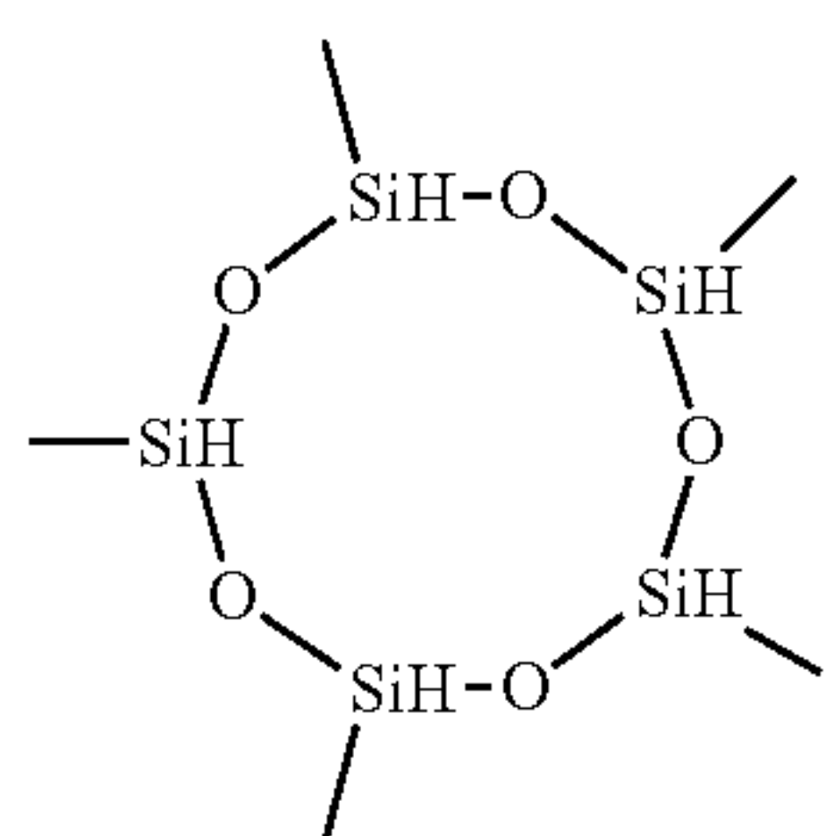
2,4,6,8,10-Pentamethylcyclopentasiloxane
