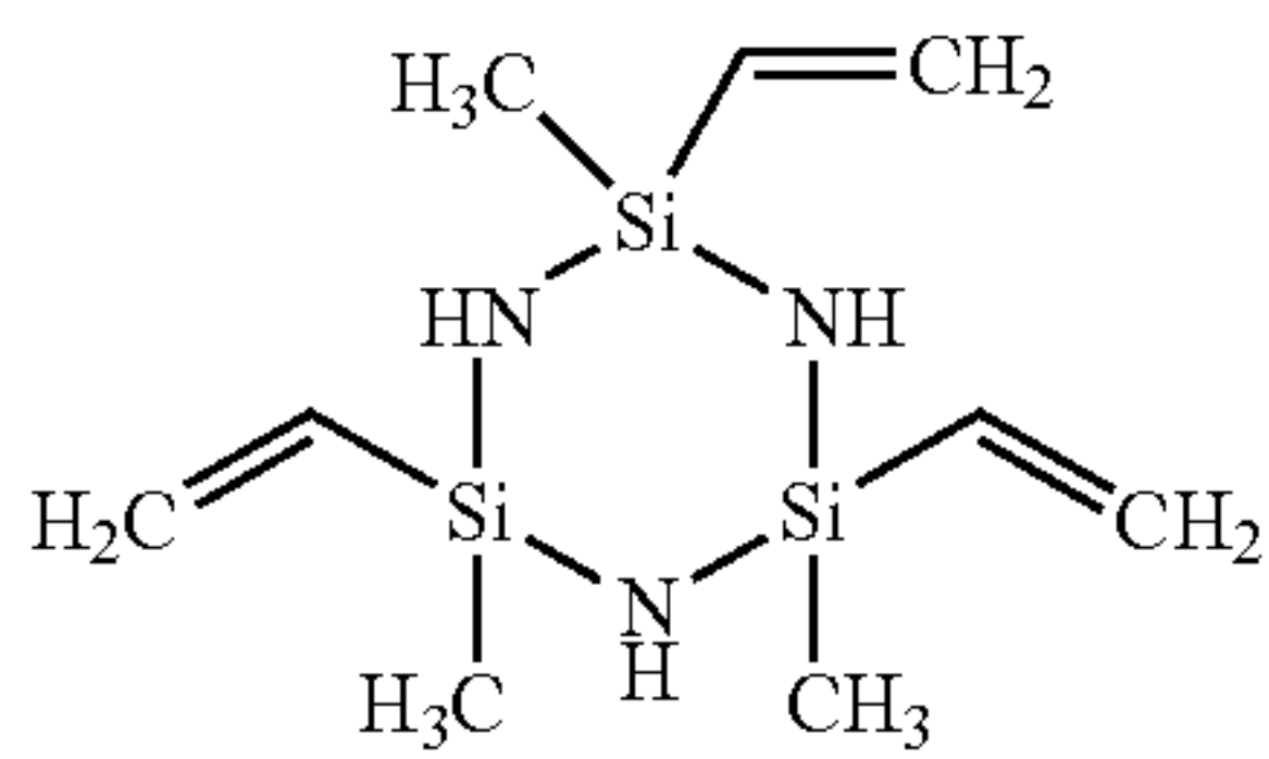
2,4,6-Trimethyl-2,4,6-trivinylcyclotrisilazane (TriMTVCTS) (CAS: 5505-72-6)
