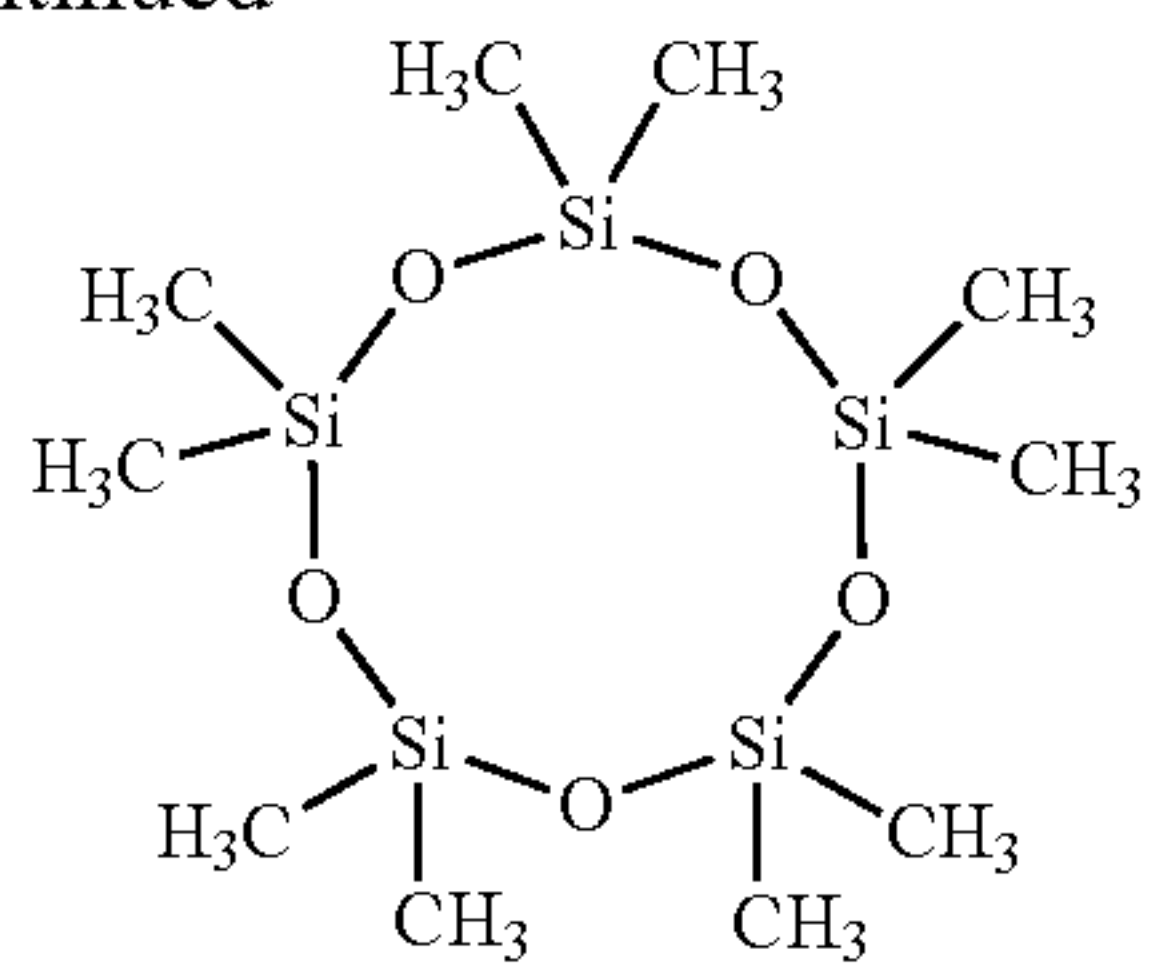
Decamethylcyclopentasiloxane
