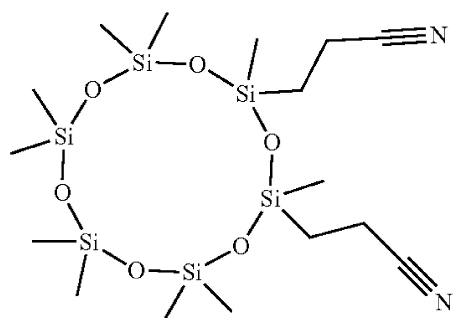
2,2,4,4,6,6,8,8,10,12-decamethyl-10,12-di(2-cyanoethyl)-[1,3,5,7,9,11,2,4,6,8,10,12]cyclohexasiloxane
