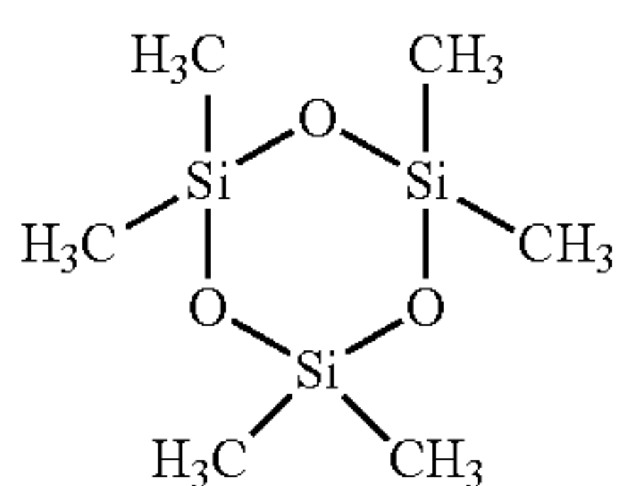
Hexamethylcyclotrisiloxane
