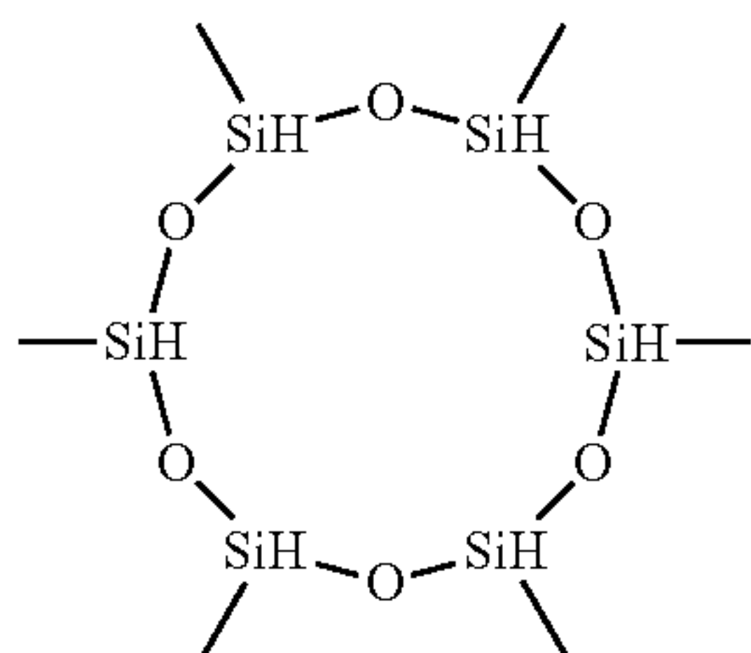
2,4,6,8,10,12-Hexamethylcyclohexasiloxane
