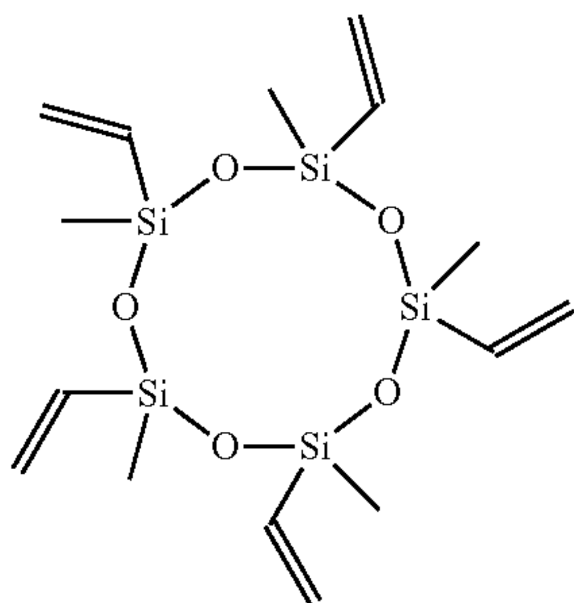
1,3,5,7,9-Pentamethyl-1,3,5,7,9-pentavinylcyclopentasiloxane
