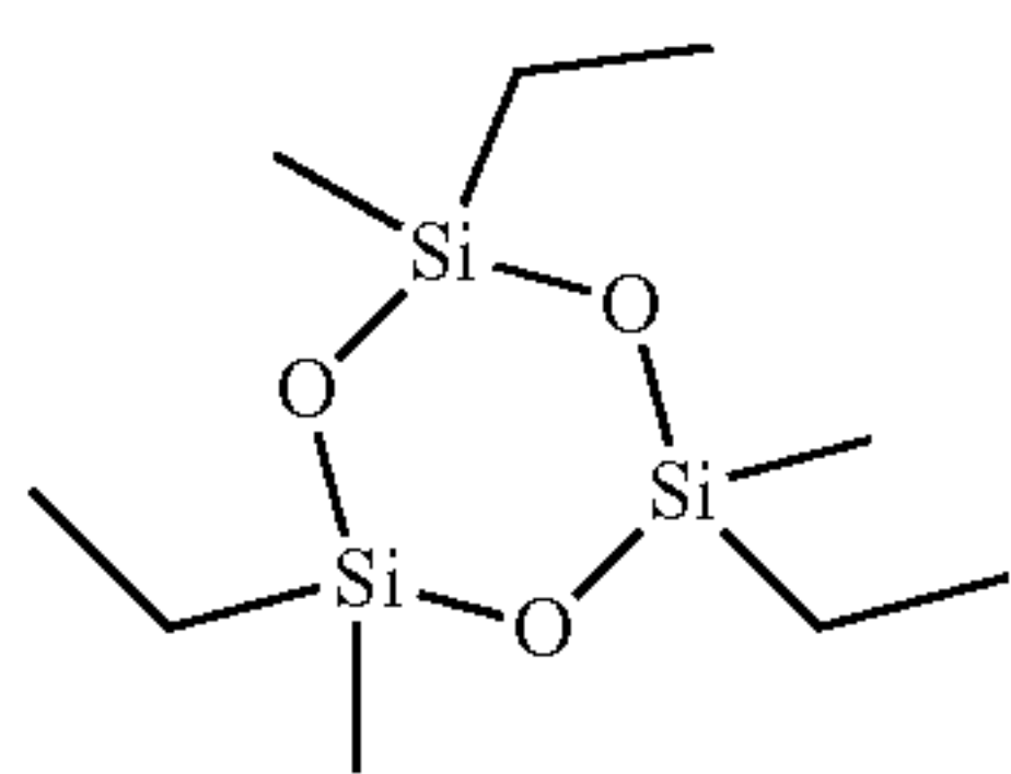
2,4,6-Triethyl-2,4,6-trimethylcyclotrisiloxane
