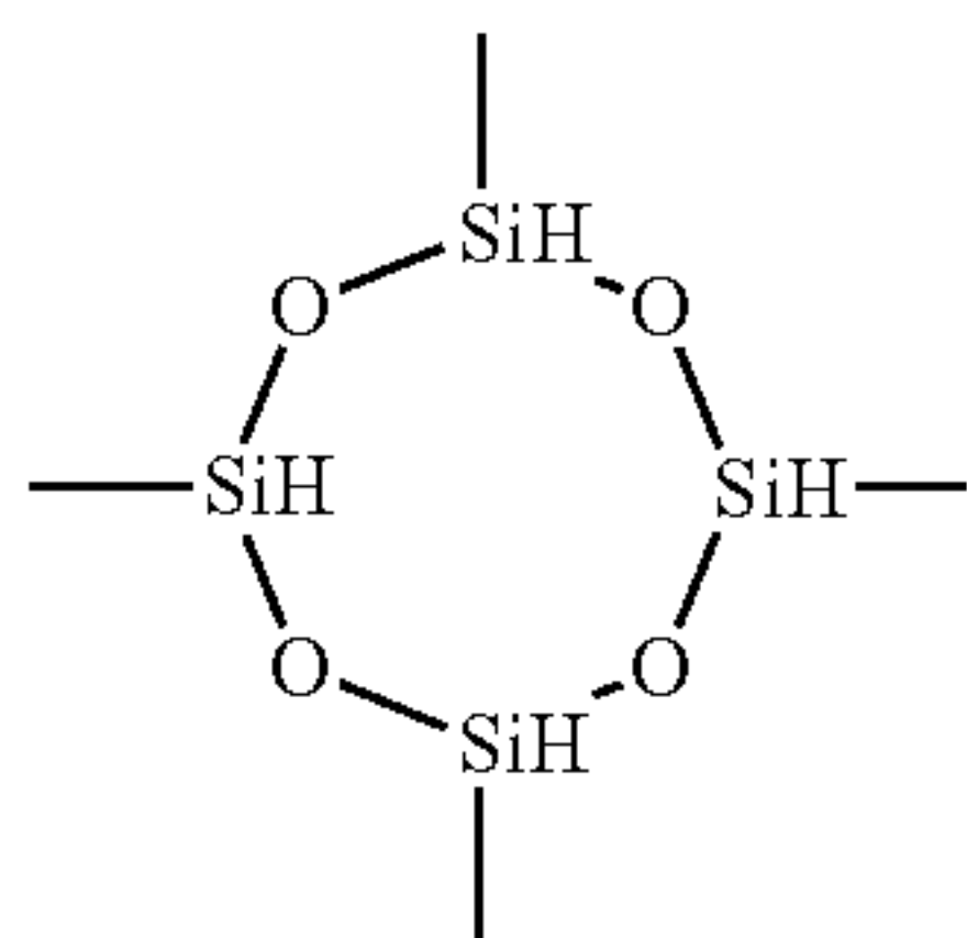
2,4,6,8-Tetramethylcyclotetrasiloxane
