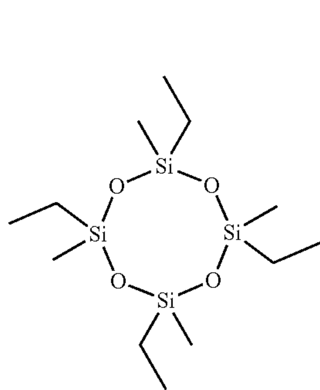
2,4,6,8-Tetraethyl-2,4,6,8-tetramethylcyclotetrasiloxane
