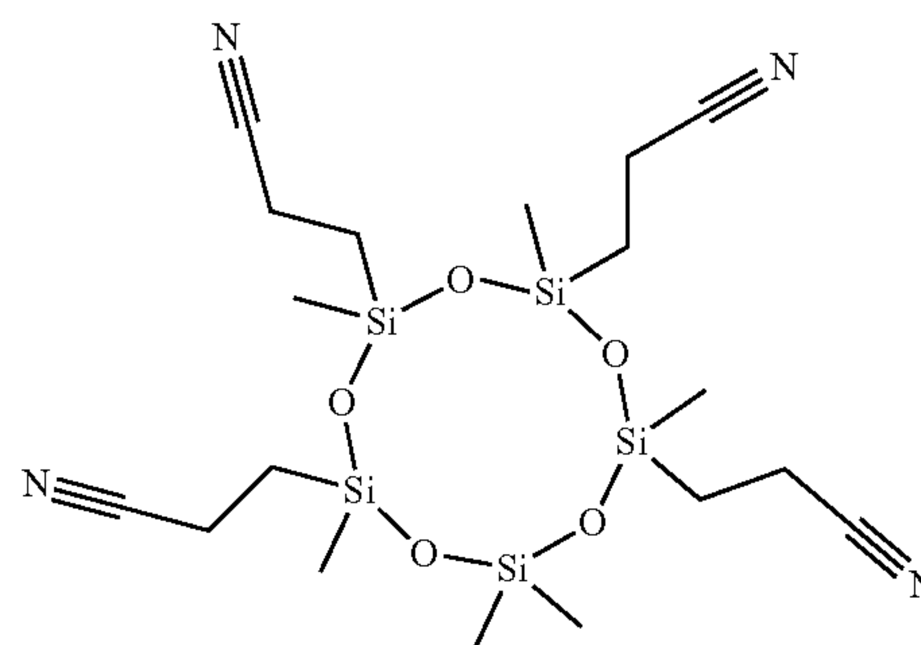
2,2,4,6,8,10-hexamethyl-4,6,8,10-tetra(2-cyanoethyl)-[1,3,5,7,9,2,4,6,8,10]cyclopentasiloxane
