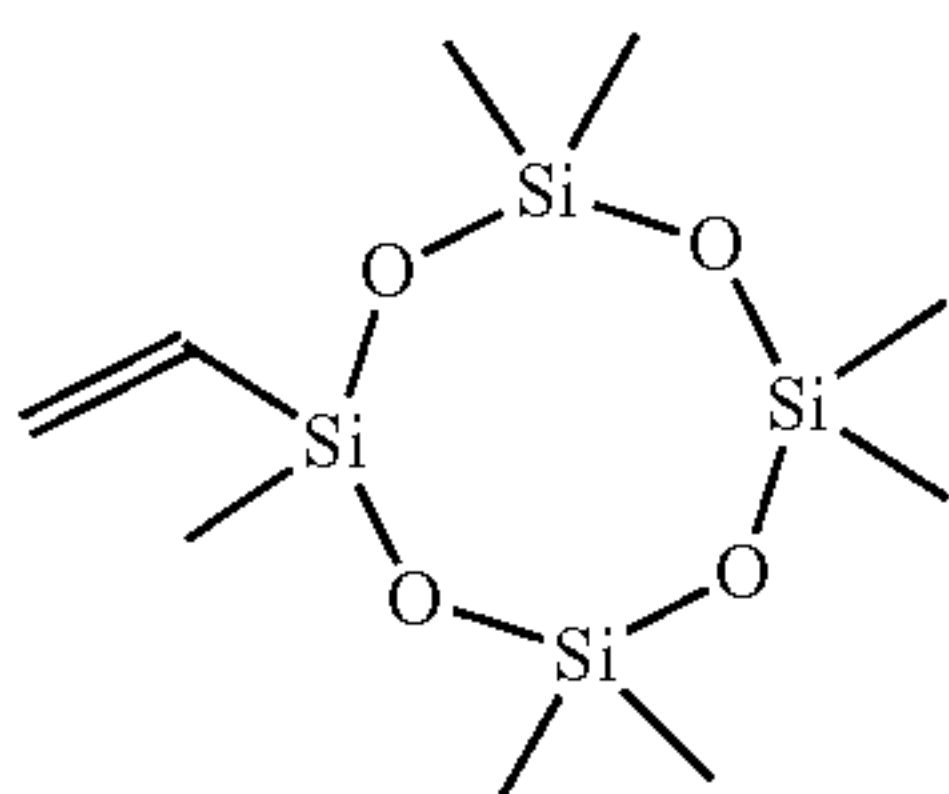
cyclotetrasiloxane, heptamethyl-, vinyl-
