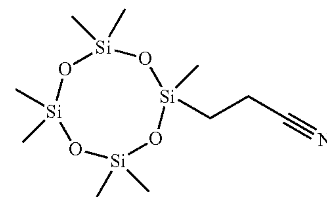
2,2,4,4,6,6,8-heptomethyl-8-(2-cyanoethyl)-[1,3,5,7,2,4,6,8]cyclotetrasiloxane
