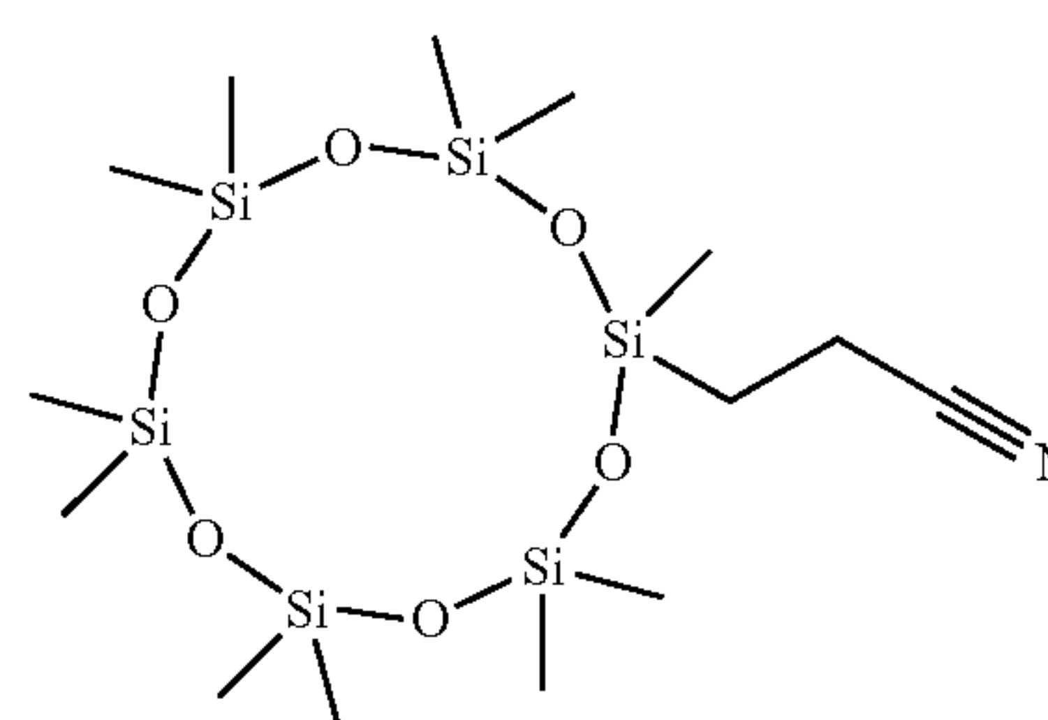
2,2,4,4,6,6,8,8,10,10,12-undecamethyl-12-(2-cyanoethyl)-[1,3,5,7,9,11,2,4,6,8,10,12]cyclohexasiloxane
