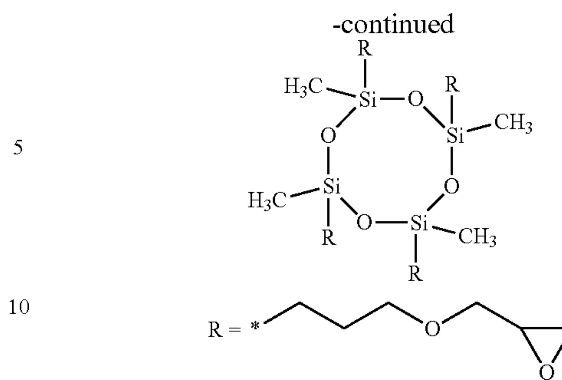
2,4,6,8-Tetramethyl-2,4,6,8-tetrakis (propyl glycidyl ether)cyclotetrasiloxane
