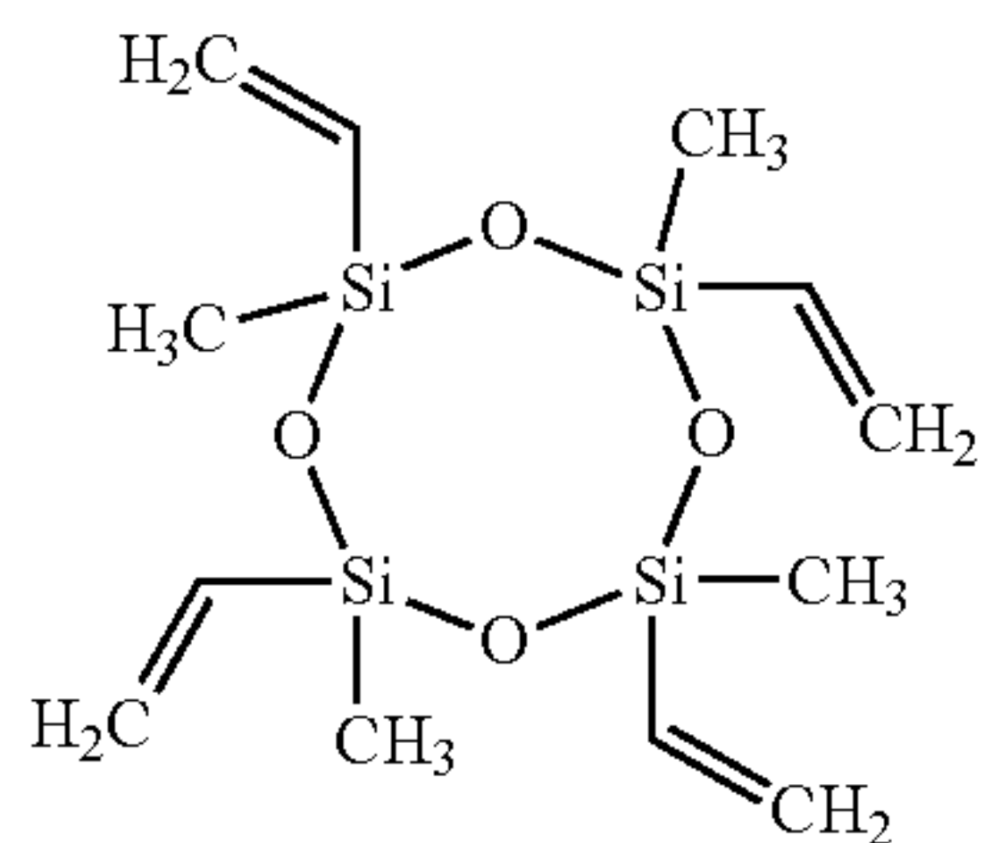
2,4,6,8-Tetramethyl-2,4,6,8-tetravinylcyclotetrasiloxane (TetraMTVCTS)
