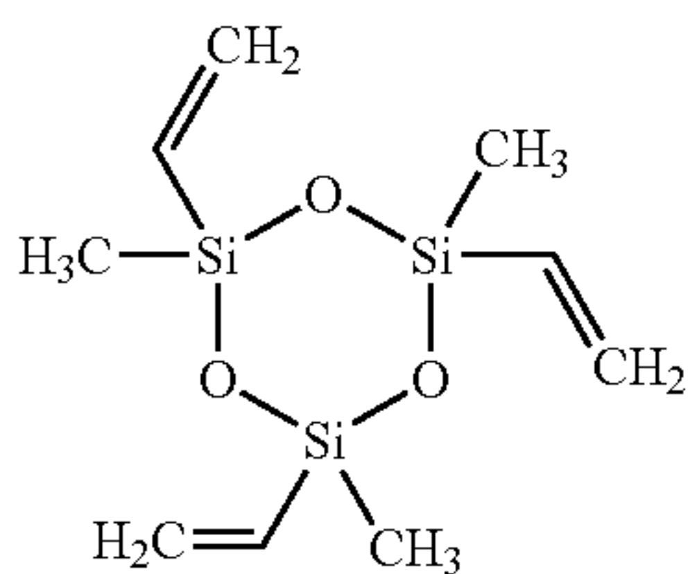
1,3,5-Trivinyl-1,3,5-trimethylcyclotrisiloxane
