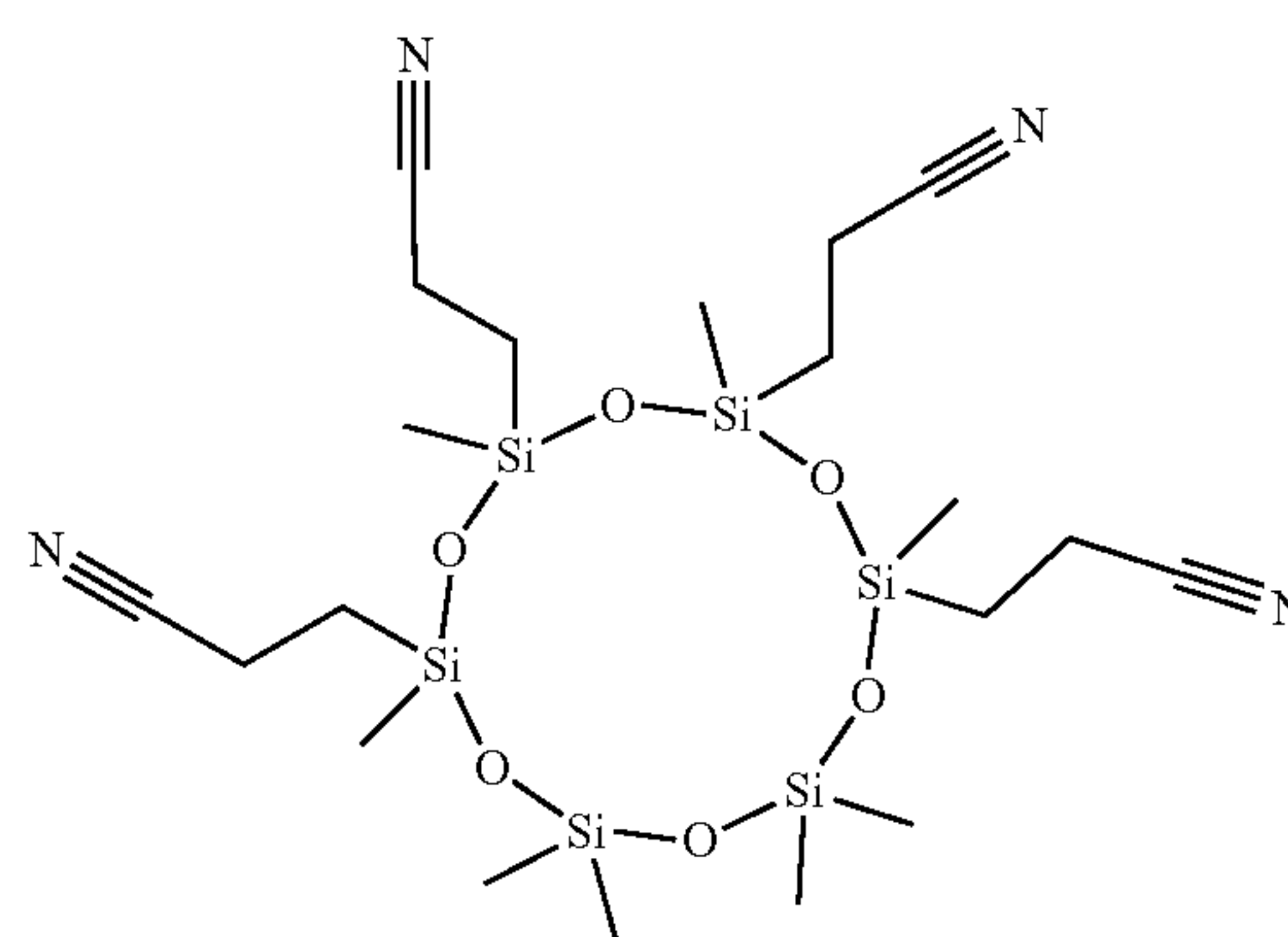
2,2,4,4,6,6,8,8,10,12-octamethyl-6,8,10,12-tetra(2-cyanoethyl)-[1,3,5,7,9,11,2,4,6,8,10,12]cyclohexasiloxane
