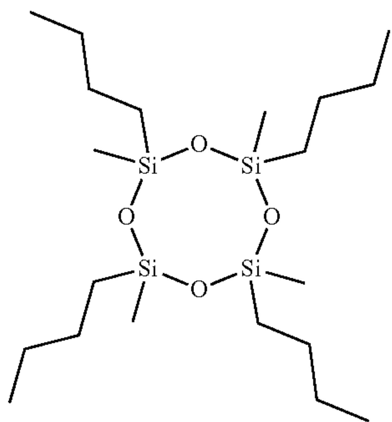
2,4,6,8-Tetrabutyl-2,4,6,8-tetramethyl-1,3,5,7,2,4,6,8-tetraoxatetrasiloxane
