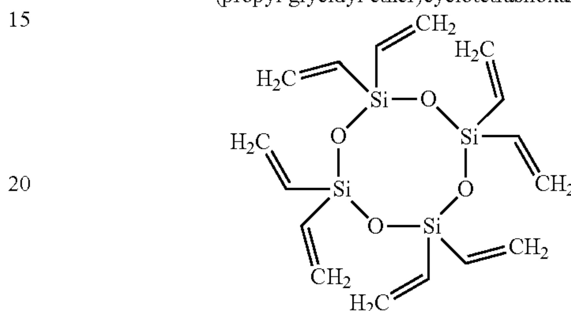
2,2,4,4,6,6,8,8-octavinyl- 1,3,5,7,2,4,6,8-tetraoxatetrasiloxane
