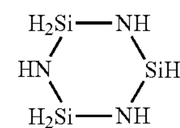
1,3,5,2,4,6-Triazatrisilane
