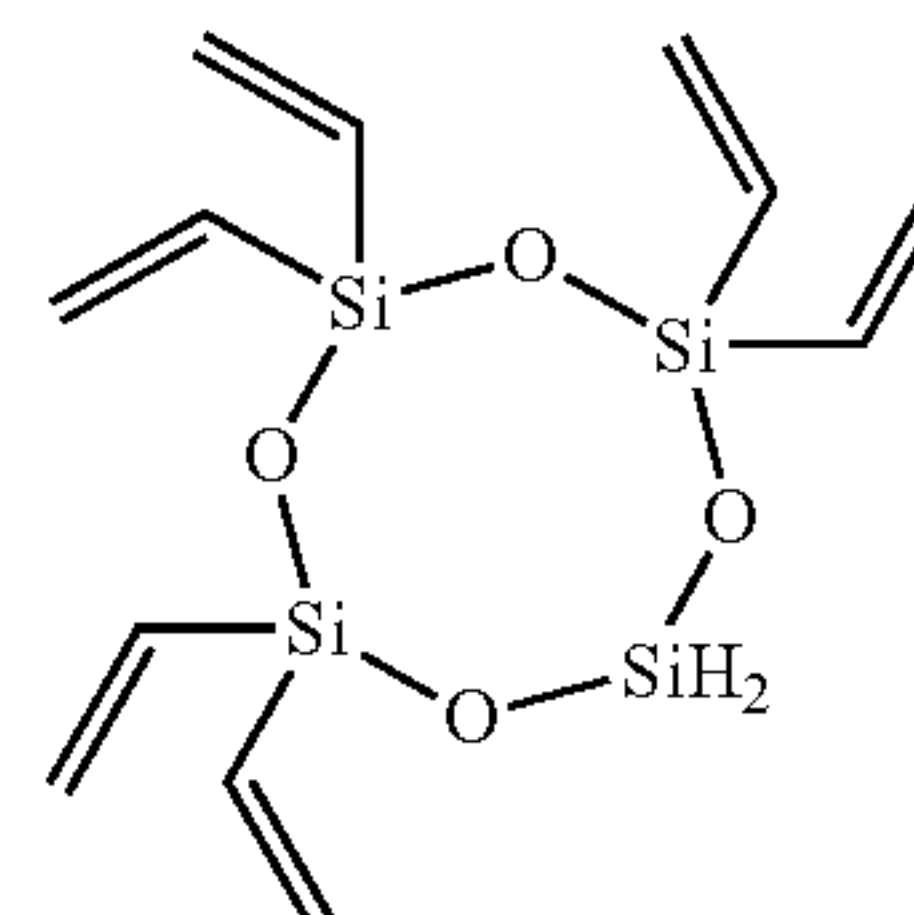
2,2,4,4,6,6-hexavinyl-1,3,5,7,2,4,6,8-tetraoxatetrasilocane
