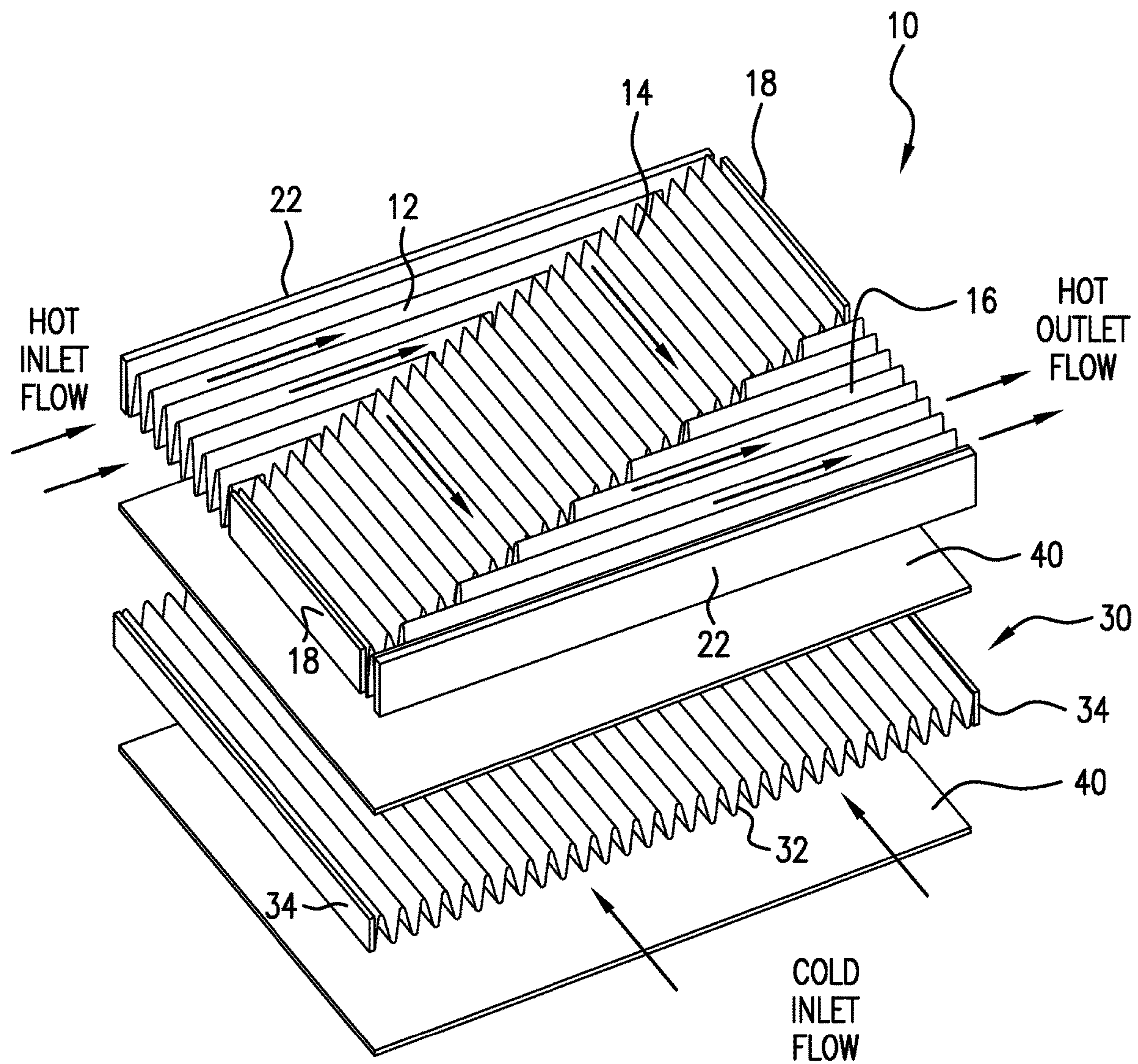
FIG. 1 (Prior Art)
