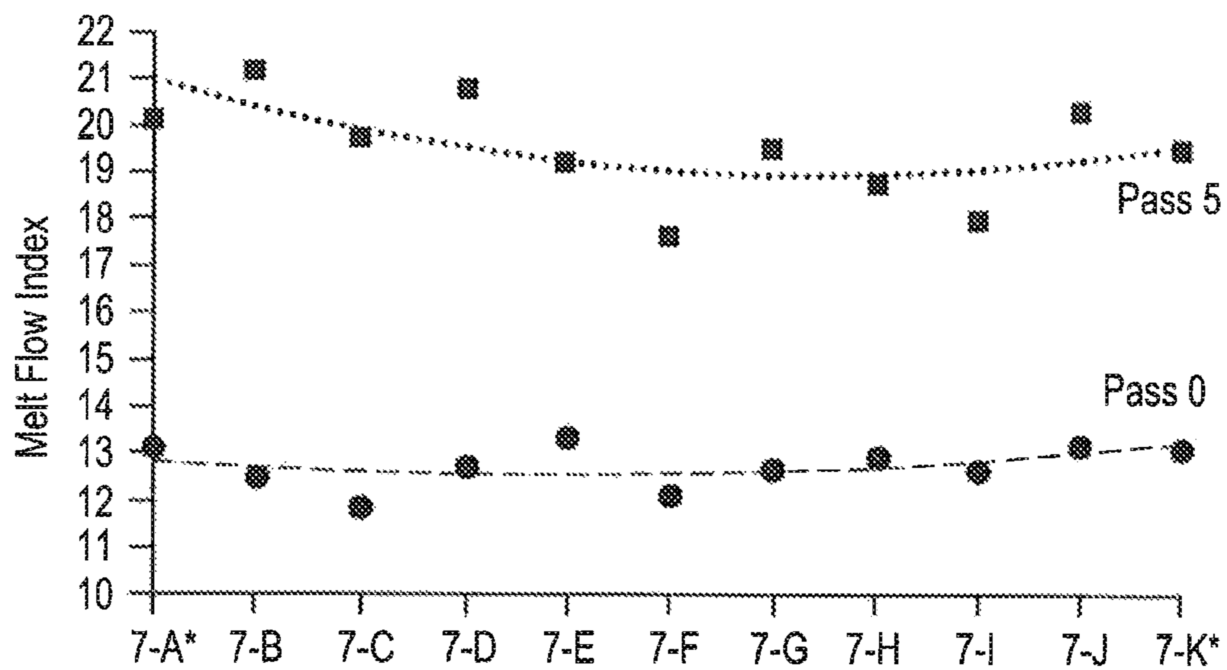
Melt Flow Index of the Formulations Before and After Processing
