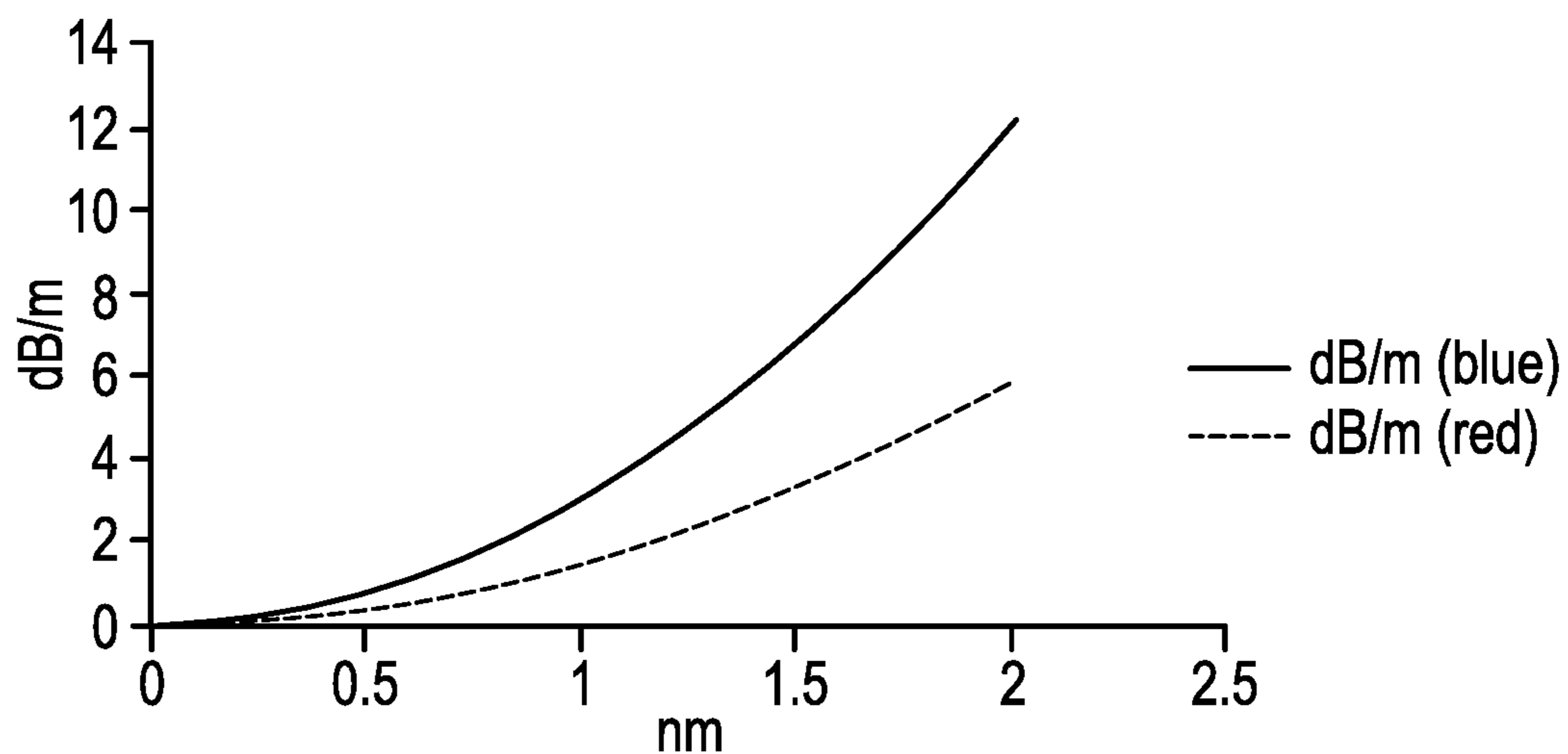
Estimated loss versus RMS roughness
