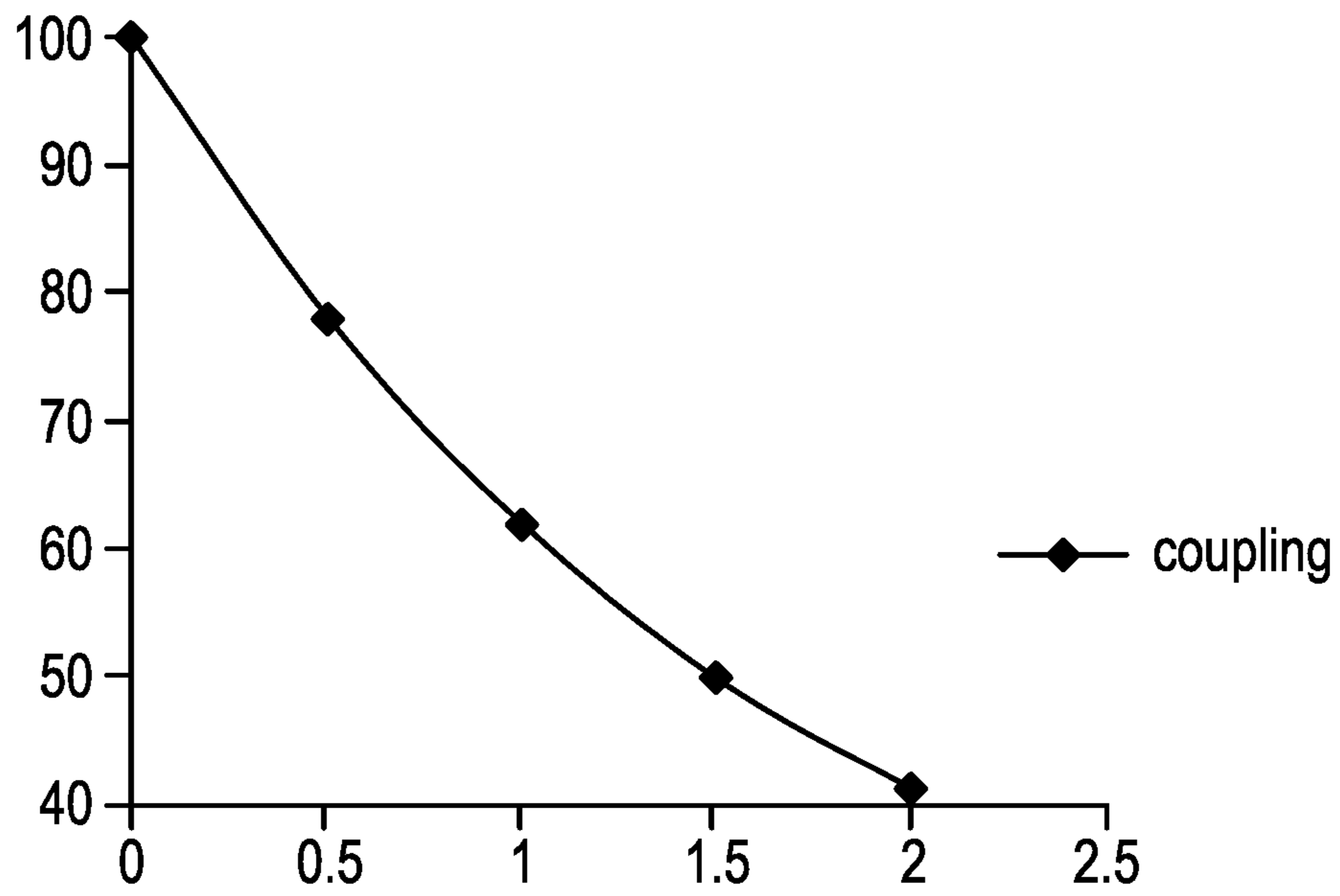
Light coupling versus LED to LGP distance
