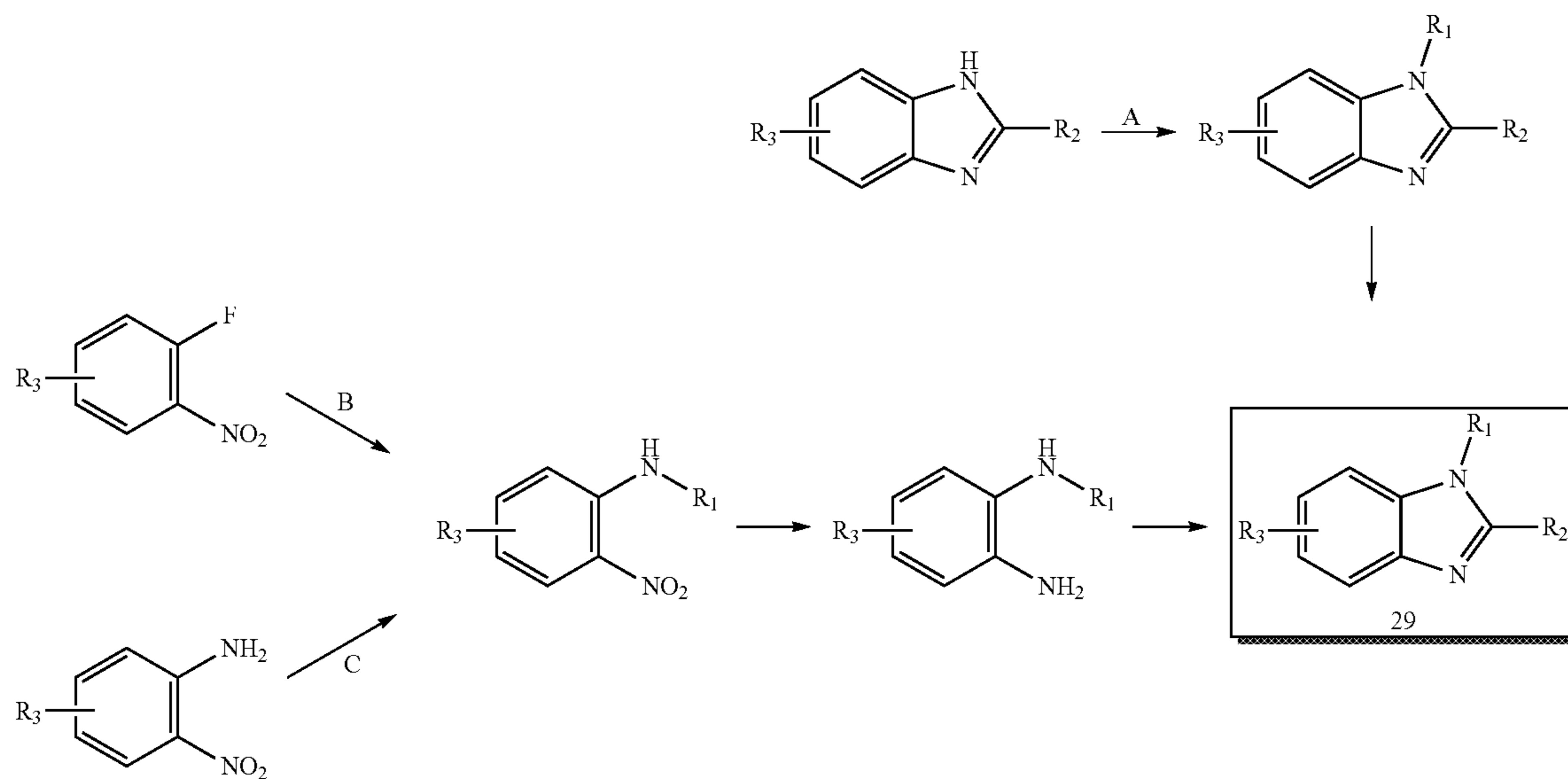
Scheme 2: Synthesis of benzimidazole analogs
